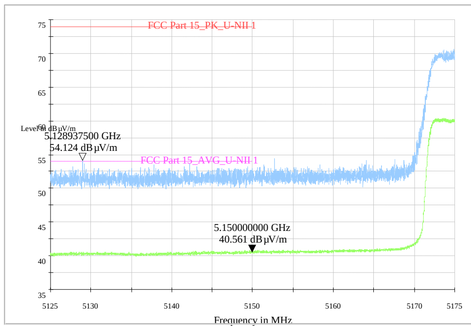
RE-Power_5.125G-5.175GHz
