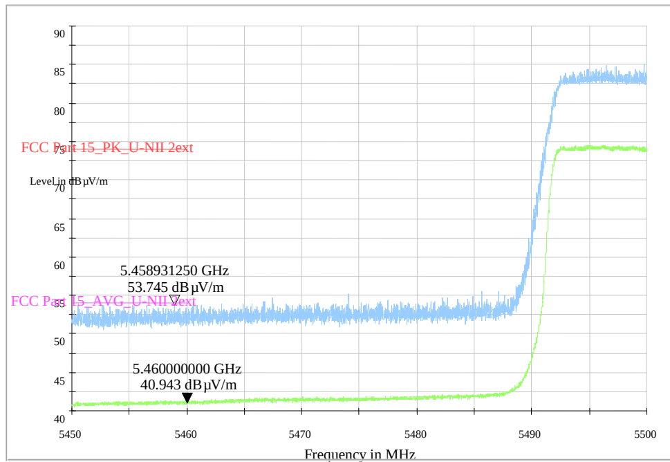
RE-Power_5.45G-5.5GHz
