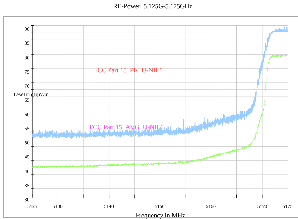
Fig. 44 Band Edges (802.11n-HT20, 5180MHz)
