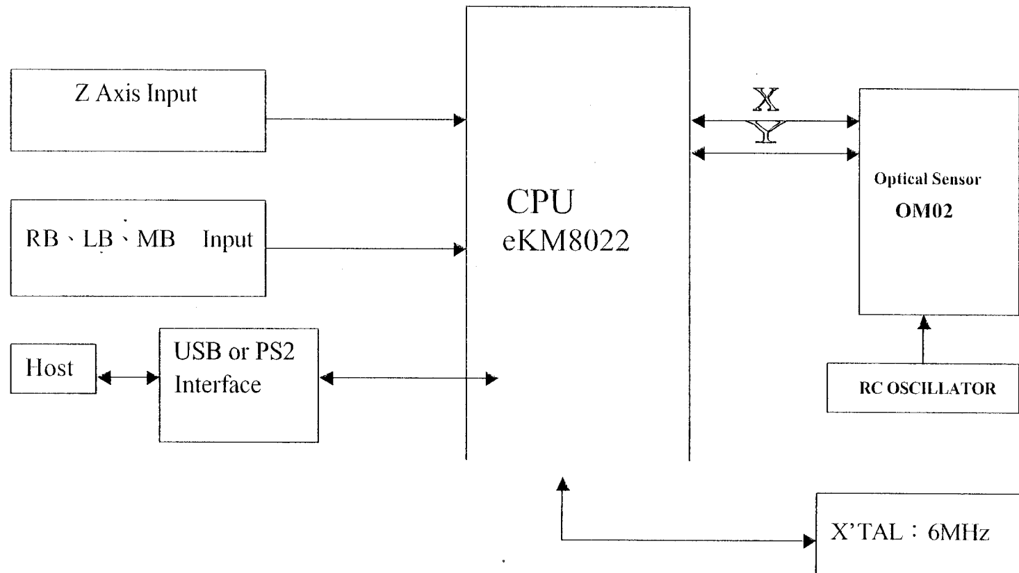
MS27U / MS28U / MS29U BLOCK DIAGRAM
