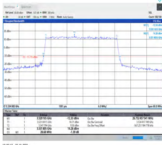
1-N77-3450-3550-PC2-30-30-H-1-DFT-QPSK-Outer_Full-75@0-Ant1-26.752-28.680-≤30-PASS
