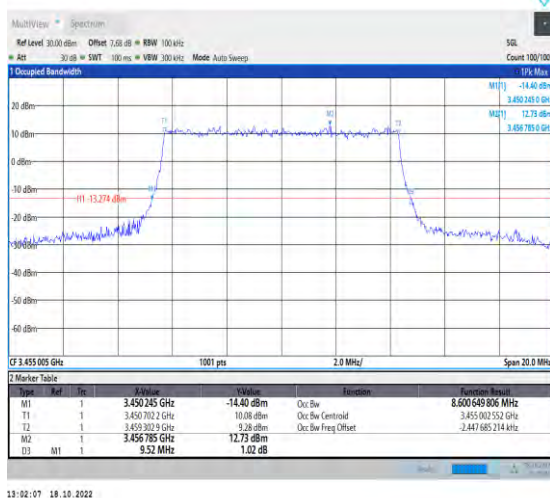
1-N77-3450-3550-PC2-30-10-L-4-DFT-64QAM-Outer_Full-24@0-Ant1-8.601-9.520-≤10-PASS
