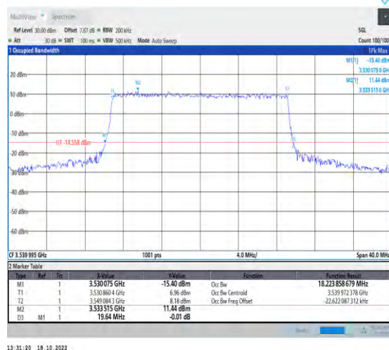
1-N77-3450-3550-PC2-30-20-H-7-CP-16QAM-Outer_Full-51@0-Ant1-18.224-19.640-≤20-PASS
