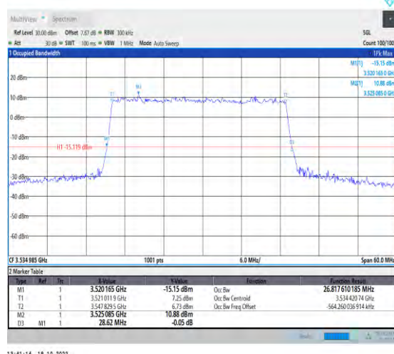
1-N77-3450-3550-PC2-30-30-H-5-DFT-256QAM-Outer_Full-75@0-Ant1-26.818-28.620-≤30-PASS
