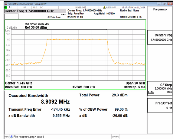
13A_n66 10M DFT-s-OFDM 64QAM Outer_Full Mid
