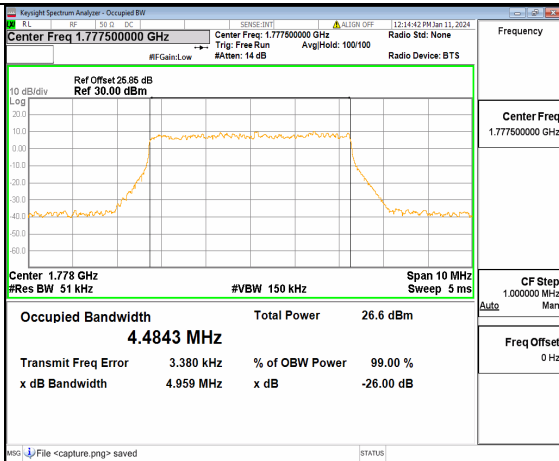
13A_n66 5M DFT-s-OFDM 256QAM Outer_Full High
