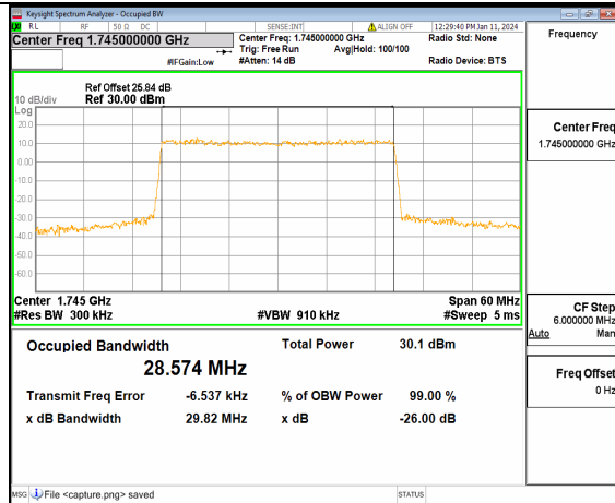
13A_n66 30M DFT-s-OFDM 16QAM Outer_Full Mid
