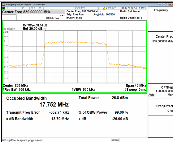
2A_n5 20M DFT-s-OFDM 256QAM Outer_Full High
