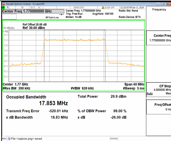
13A_n66 20M DFT-s-OFDM 16QAM Outer_Full High
