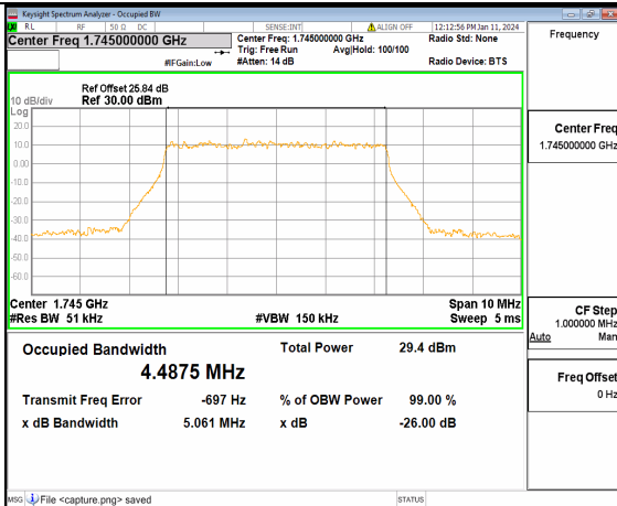
13A_n66 5M DFT-s-OFDM 16QAM Outer_Full Mid
