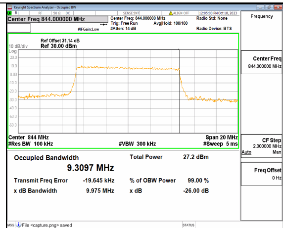
2A_n5 10M CP-OFDM QPSK Outer_Full High
