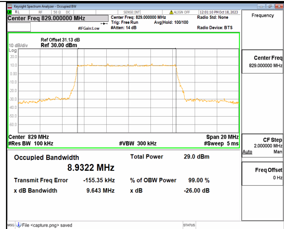
2A_n5 10M DFT-s-OFDM 64QAM Outer_Full Low
