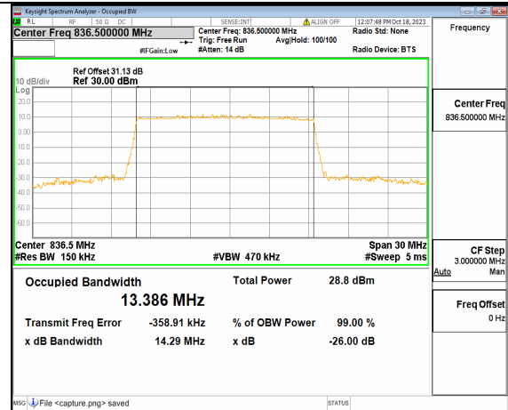
2A_n5 15M DFT-s-OFDM 64QAM Outer_Full Mid
