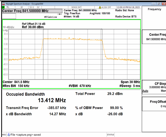
2A_n5 15M DFT-s-OFDM 16QAM Outer_Full High
