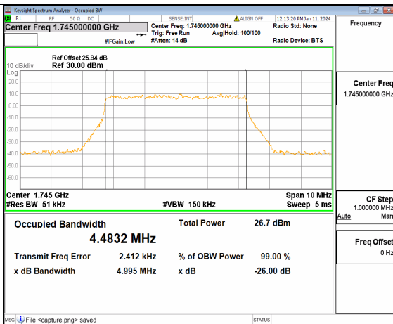
13A_n66 5M DFT-s-OFDM 256QAM Outer_Full Mid
