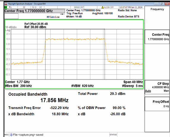
13A_n66 20M DFT-s-OFDM 64QAM Outer_Full High
