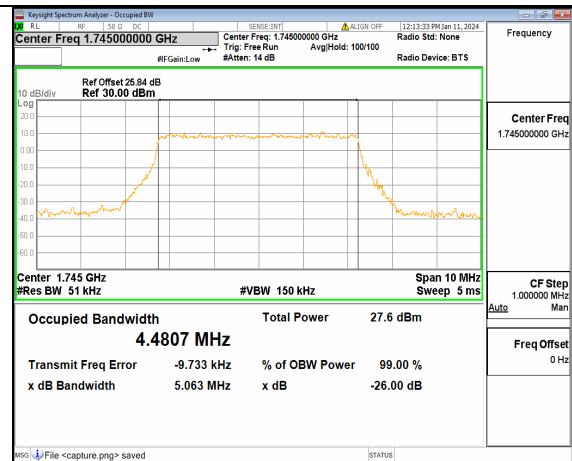
13A_n66 5M CP-OFDM QPSK Outer_Full Mid
