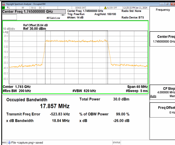
13A_n66 20M DFT-s-OFDM 16QAM Outer_Full Mid
