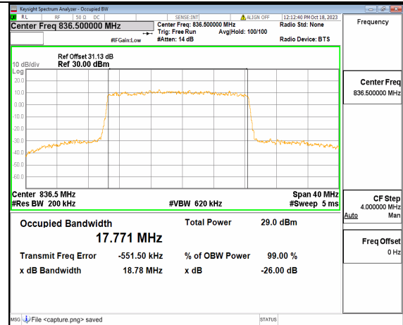
2A_n5 20M DFT-s-OFDM 64QAM Outer_Full Mid
