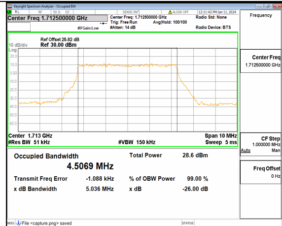
13A_n66 5M DFT-s-OFDM 64QAM Outer_Full Low
