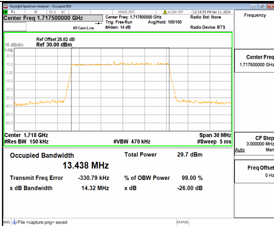
13A_n66 15M DFT-s-OFDM 16QAM Outer_Full Low
