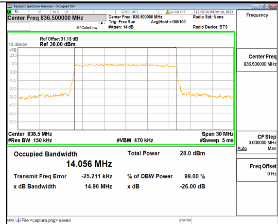
2A_n5 15M CP-OFDM QPSK Outer_Full Mid
