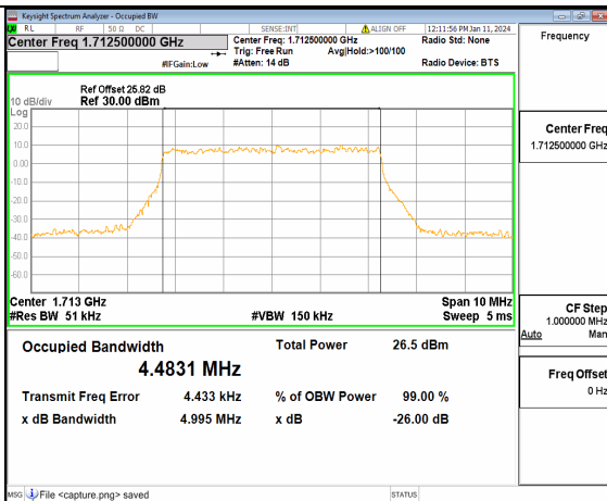
13A_n66 5M DFT-s-OFDM 256QAM Outer_Full Low
