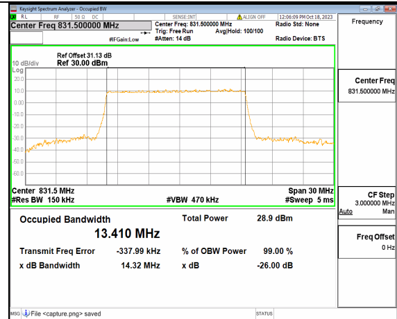
2A_n5 15M DFT-s-OFDM 64QAM Outer_Full Low
