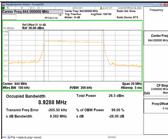
2A_n5 10M DFT-s-OFDM 256QAM Outer_Full High
