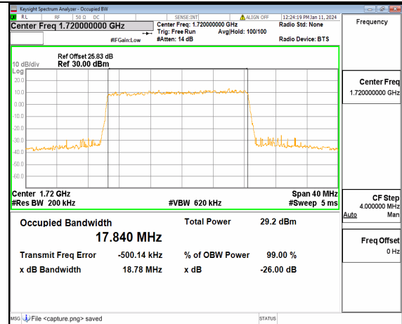
13A_n66 20M DFT-s-OFDM 64QAM Outer_Full Low
