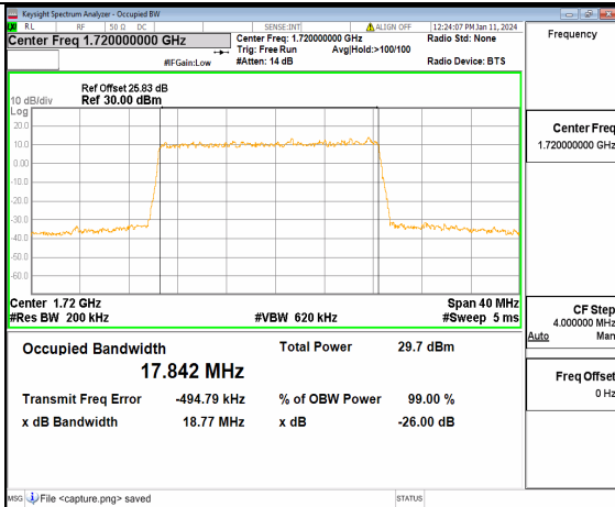
13A_n66 20M DFT-s-OFDM 16QAM Outer_Full Low
