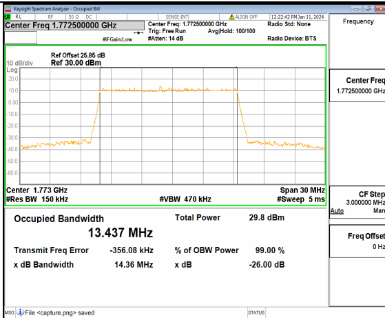
13A_n66 15M DFT-s-OFDM 16QAM Outer_Full High
