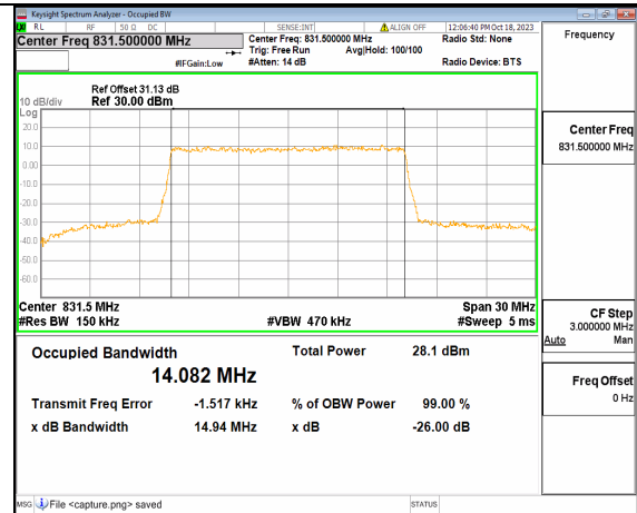
2A_n5 15M CP-OFDM QPSK Outer_Full Low
