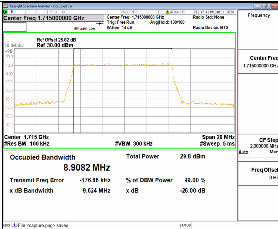
13A_n66 10M DFT-s-OFDM 16QAM Outer_Full Low
