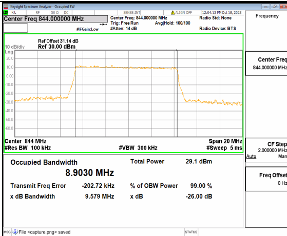
2A_n5 10M DFT-s-OFDM 16QAM Outer_Full High
