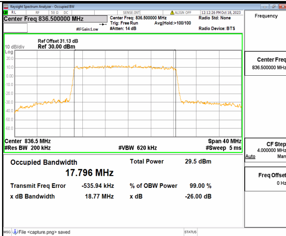
2A_n5 20M DFT-s-OFDM 16QAM Outer_Full Mid
