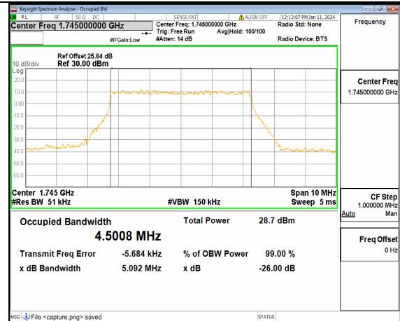
13A_n66 5M DFT-s-OFDM 64QAM Outer_Full Mid
