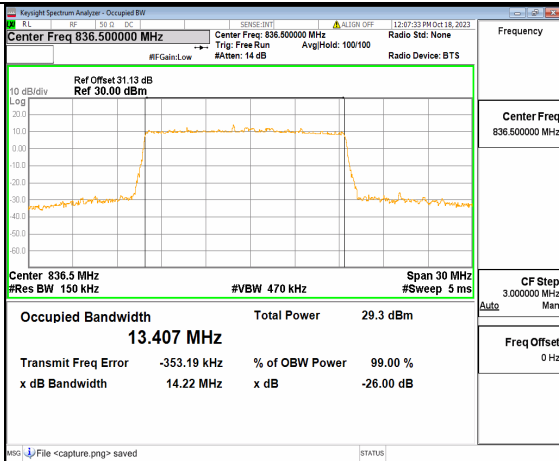
2A_n5 15M DFT-s-OFDM 16QAM Outer_Full Mid
