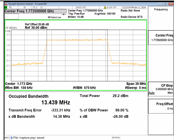
13A_n66 15M DFT-s-OFDM 64QAM Outer_Full High
