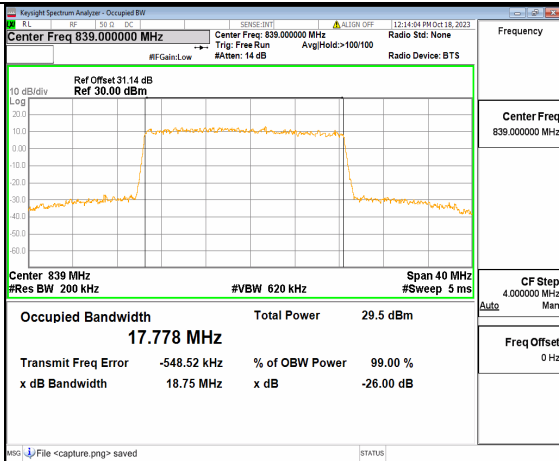
2A_n5 20M DFT-s-OFDM 16QAM Outer_Full High
