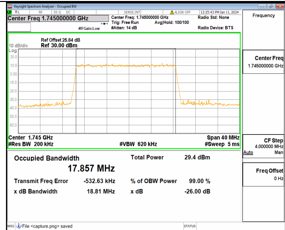
13A_n66 20M DFT-s-OFDM 64QAM Outer_Full Mid
