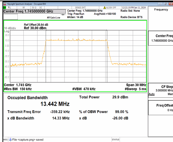
13A_n66 15M DFT-s-OFDM 16QAM Outer_Full Mid
