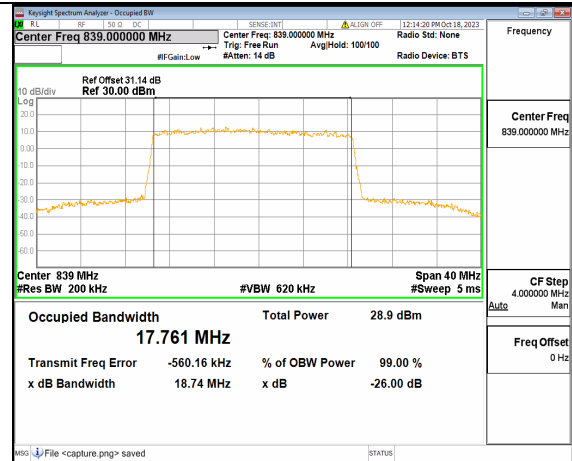
2A_n5 20M DFT-s-OFDM 64QAM Outer_Full High
