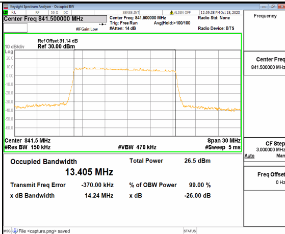
2A_n5 15M DFT-s-OFDM 256QAM Outer_Full High
