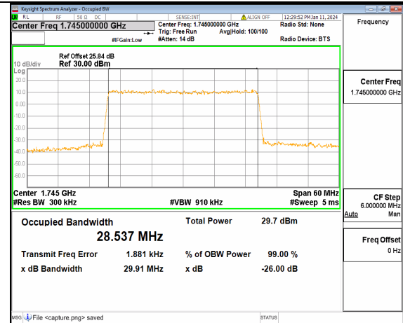
13A_n66 30M DFT-s-OFDM 64QAM Outer_Full Mid
