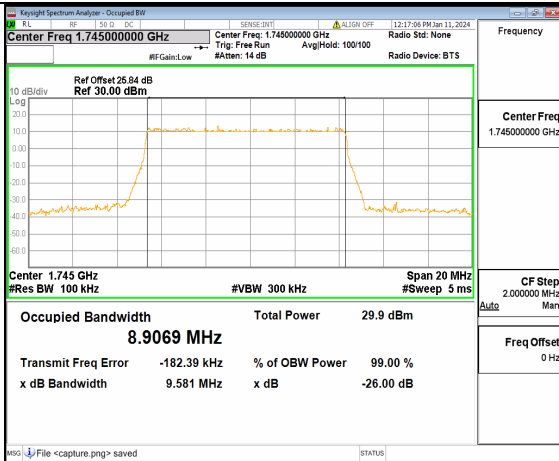
13A_n66 10M DFT-s-OFDM 16QAM Outer_Full Mid
