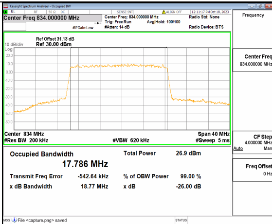
2A_n5 20M DFT-s-OFDM 256QAM Outer_Full Low
