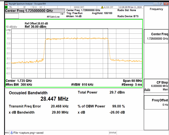
13A_n66 30M DFT-s-OFDM 64QAM Outer_Full Low
