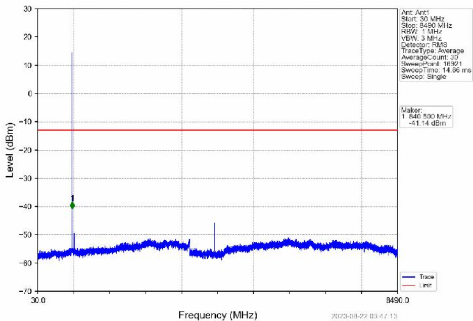
Band5 1.4MHz 16QAM HCH 848.3MHz RB 1_0 NTN
