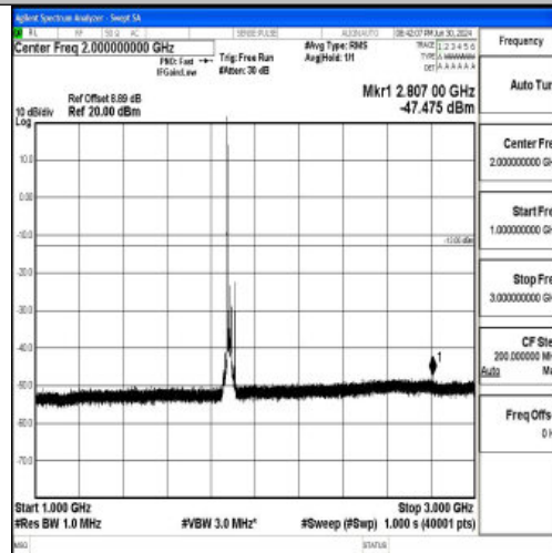
Band25_20MHz_16QAM_26365_1RB#0_1000~3000_1000~3000
