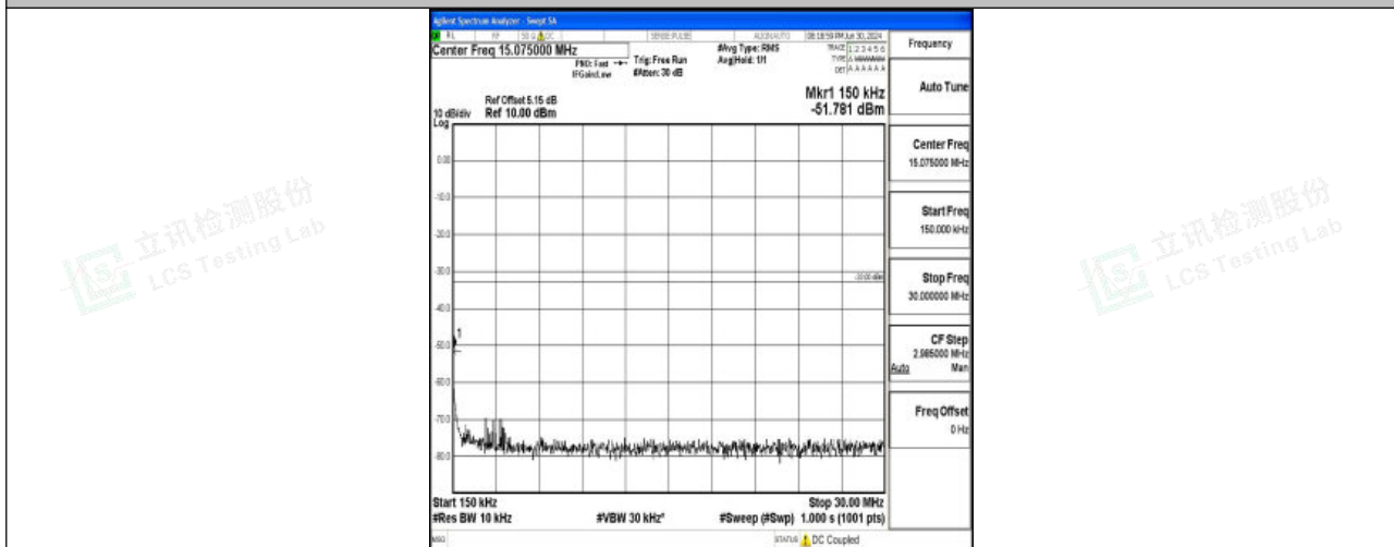
Band25_15MHz_16QAM_26115_1RB#0_0.15~30_0.15~30
