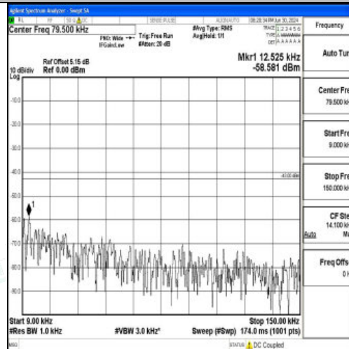
Band25_15MHz_QPSK_26615_1RB#0_0.009~0.15_0.009~0.15
