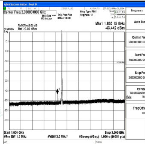
Band25_5MHz_QPSK_26665_1RB#0_1000~3000_1000~3000
