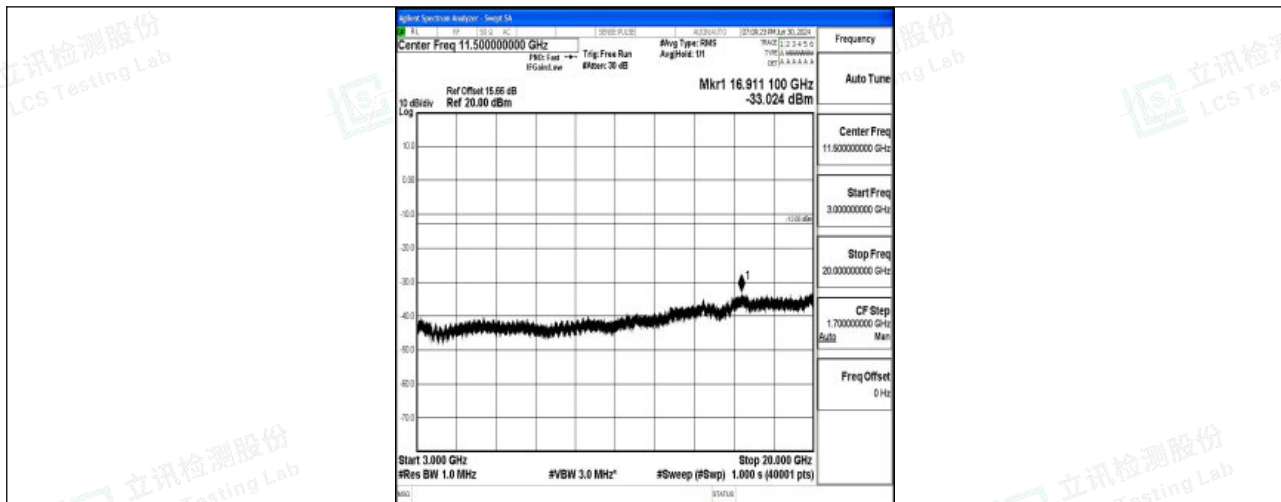
Band25_3MHz_QPSK_26055_1RB#0_3000~20000_3000~20000
