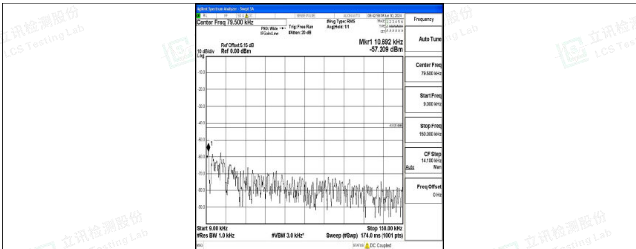
Band25_20MHz_16QAM_26590_1RB#0_0.009~0.15_0.009~0.15
