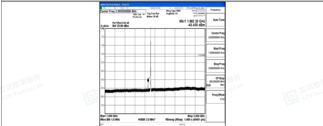
Band25_3MHz_QPSK_26675_1RB#0_1000~3000_1000~3000
