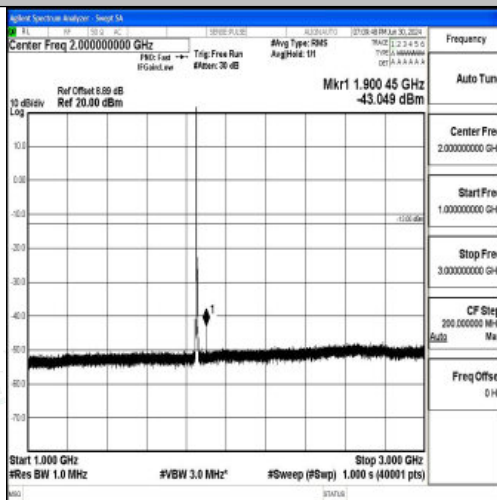
Band25_3MHz_16QAM_26055_1RB#0_1000~3000_1000~3000
