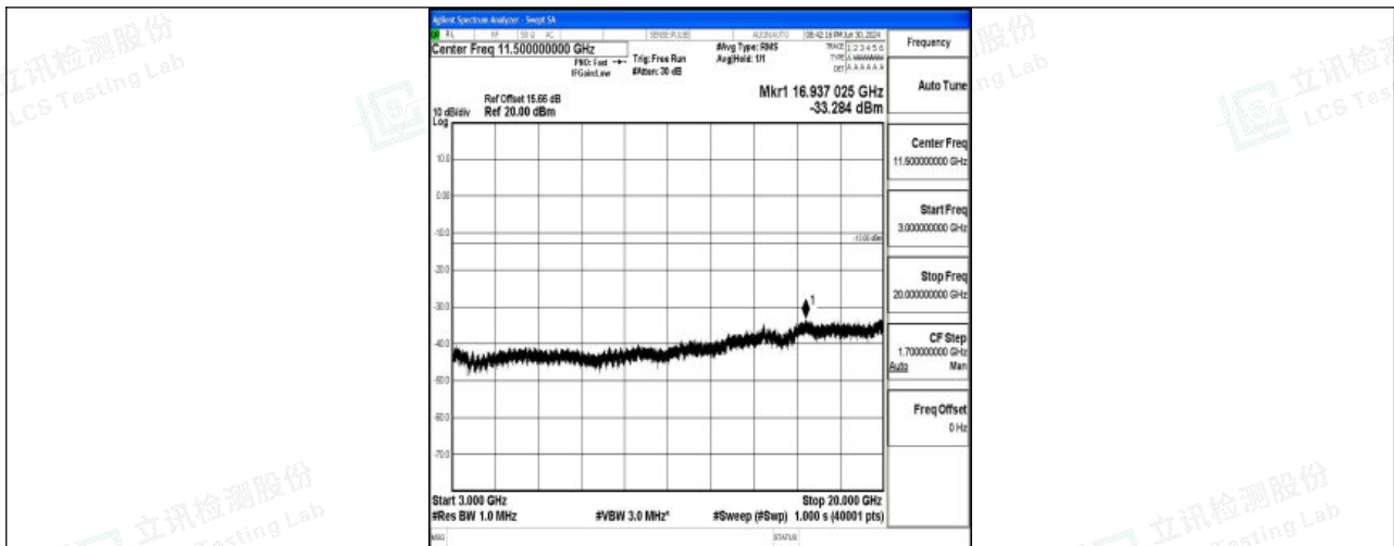
Band25_20MHz_16QAM_26365_1RB#0_3000~20000_3000~20000
