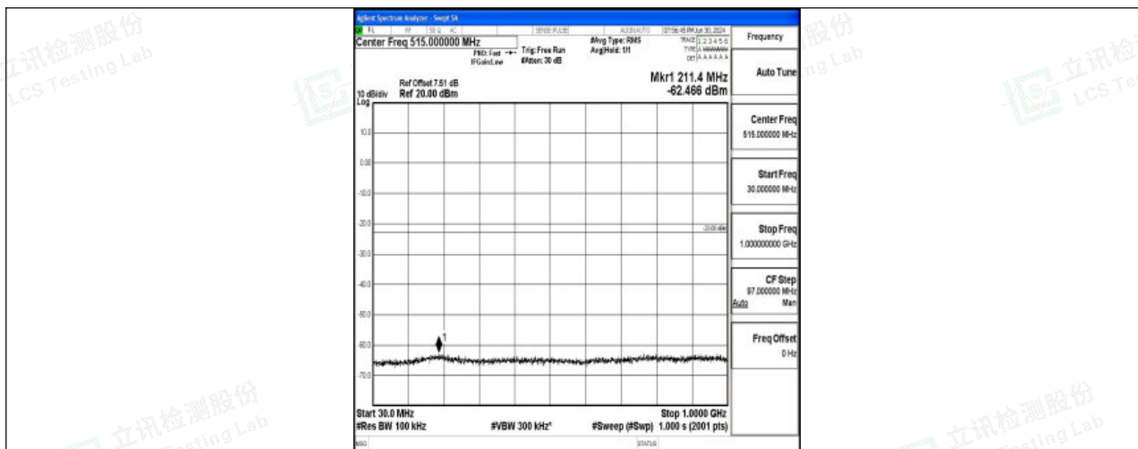
Band25_10MHz_16QAM_26090_1RB#0_30~1000_30~1000
