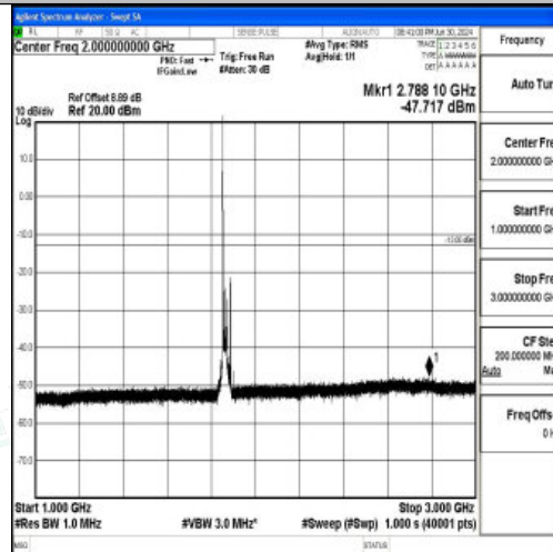
Band25_20MHz_16QAM_26140_1RB#0_1000~3000_1000~3000
