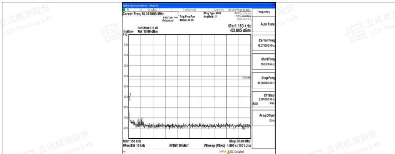
Band25_3MHz_16QAM_26365_1RB#0_0.15~30_0.15~30
