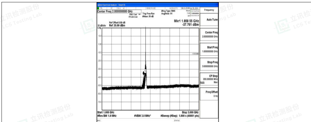
Band25_15MHz_16QAM_26615_1RB#0_1000~3000_1000~3000
