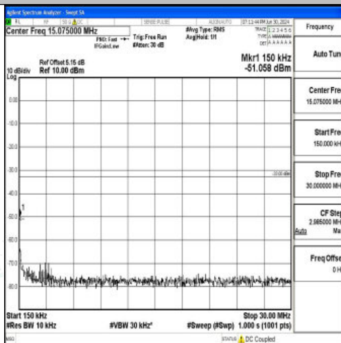
Band25_3MHz_16QAM_26675_1RB#0_0.15~30_0.15~30
