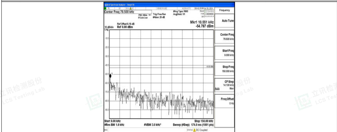
Band25_20MHz_QPSK_26590_1RB#0_0.009~0.15_0.009~0.15
