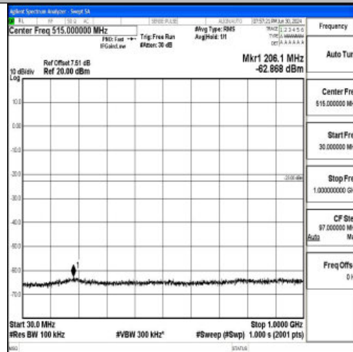
Band25_10MHz_QPSK_26365_1RB#0_30~1000_30~1000
