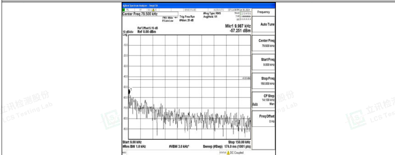
Band25_3MHz_QPSK_26675_1RB#0_0.009~0.15_0.009~0.15
