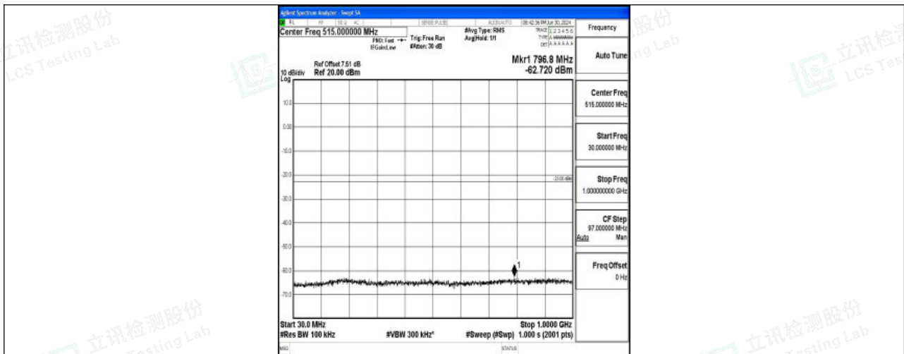
Band25_20MHz_QPSK_26590_1RB#0_30~1000_30~1000
