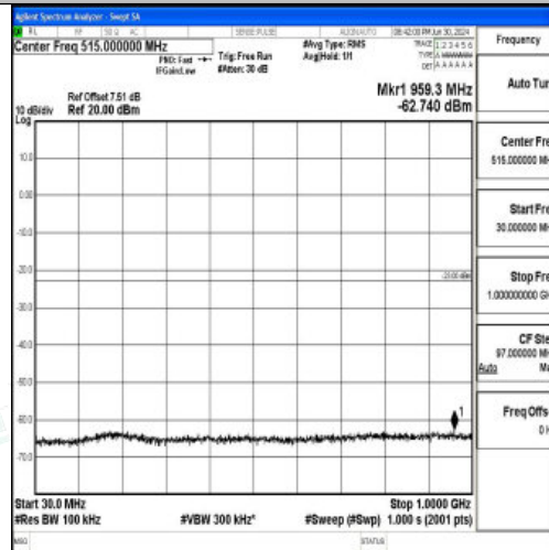
Band25_20MHz_16QAM_26365_1RB#0_30~1000_30~1000
