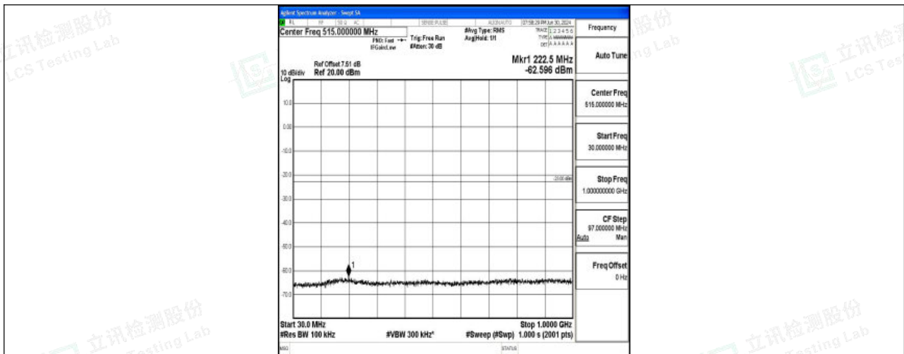
Band25_10MHz_QPSK_26640_1RB#0_30~1000_30~1000
