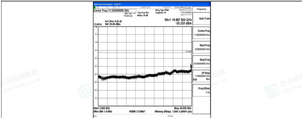
Band25_10MHz_16QAM_26640_1RB#0_3000~20000_3000~20000
