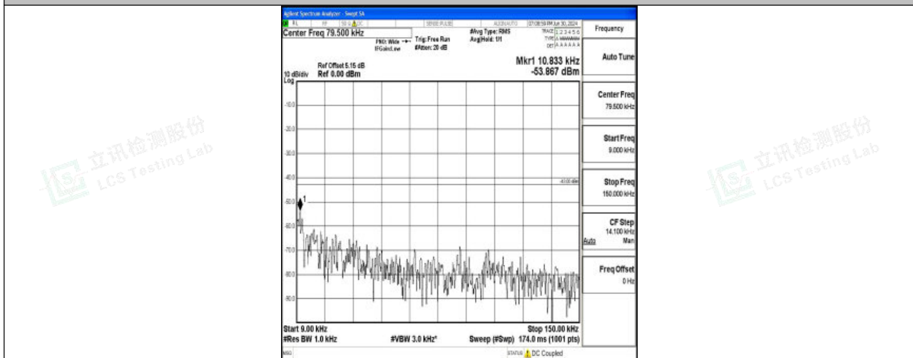
Band25_3MHz_QPSK_26055_1RB#0_0.009~0.15_0.009~0.15
