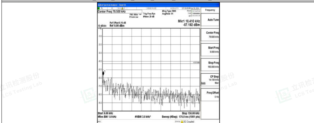
Band25_5MHz_16QAM_26065_1RB#0_0.009~0.15_0.009~0.15
