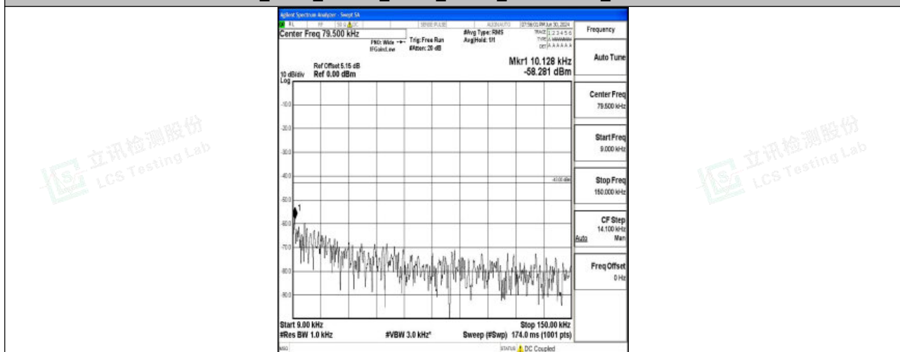
Band25_10MHz_QPSK_26090_1RB#0_0.009~0.15_0.009~0.15
