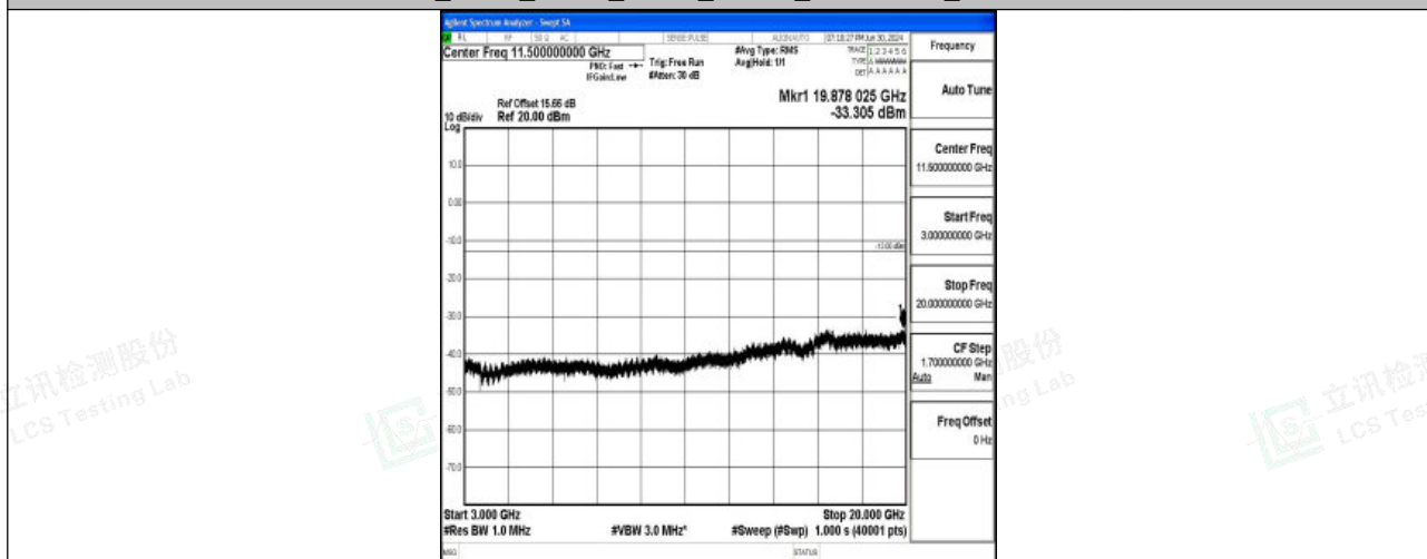
Band25_3MHz_QPSK_26365_1RB#0_3000~20000_3000~20000
