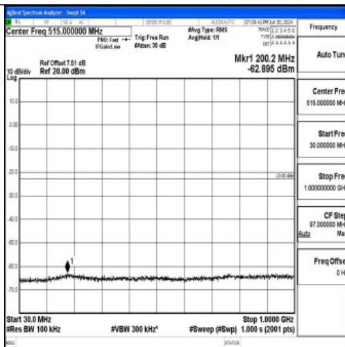
Band25_3MHz_16QAM_26055_1RB#0_30~1000_30~1000
