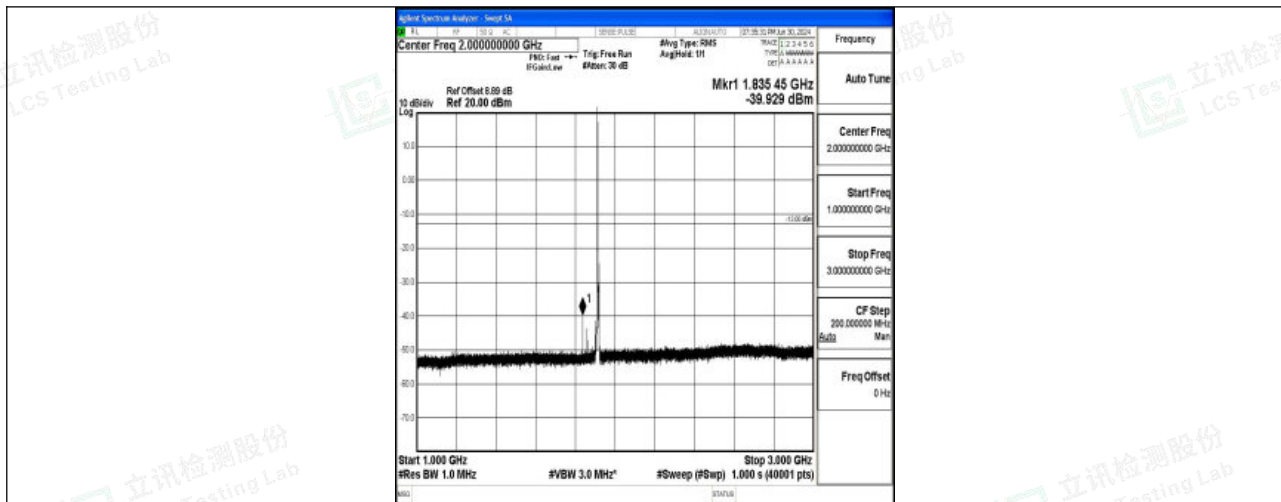
Band25_5MHz_16QAM_26665_1RB#0_1000~3000_1000~3000
