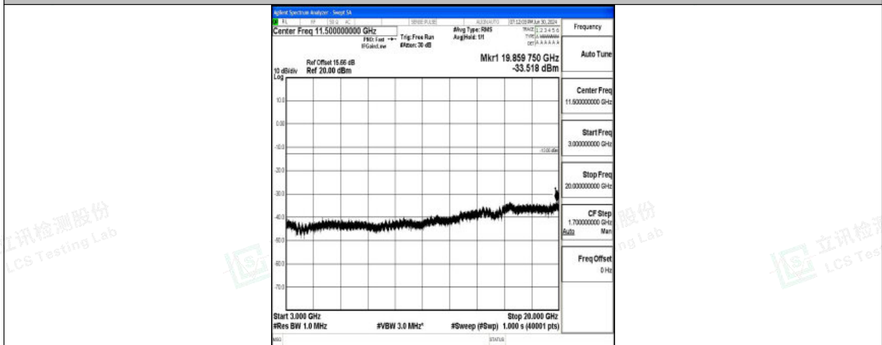
Band25_3MHz_16QAM_26675_1RB#0_3000~20000_3000~20000
