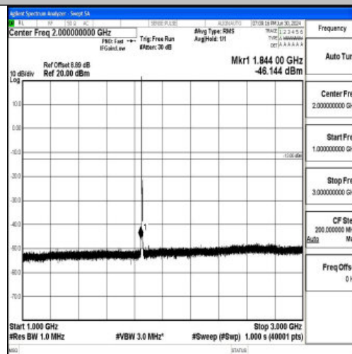
Band25_3MHz_QPSK_26055_1RB#0_1000~3000_1000~3000
