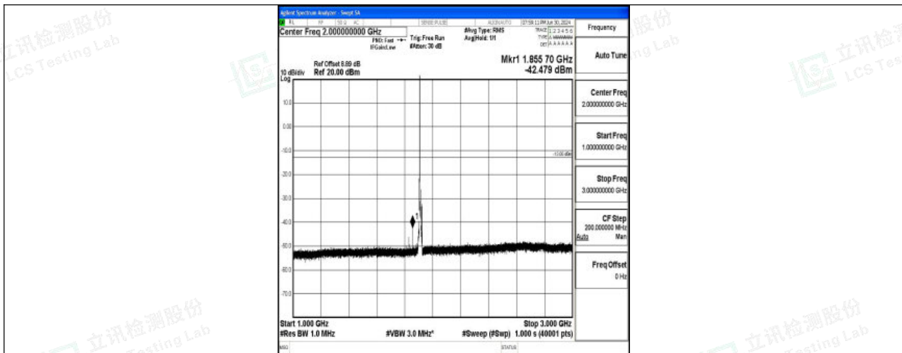
Band25_10MHz_16QAM_26640_1RB#0_1000~3000_1000~3000
