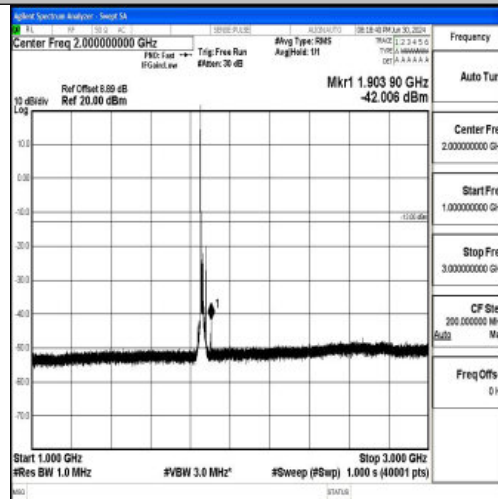
Band25_15MHz_QPSK_26115_1RB#0_1000~3000_1000~3000
