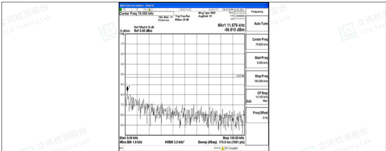
Band25_15MHz_QPSK_26365_1RB#0_0.009~0.15_0.009~0.15
