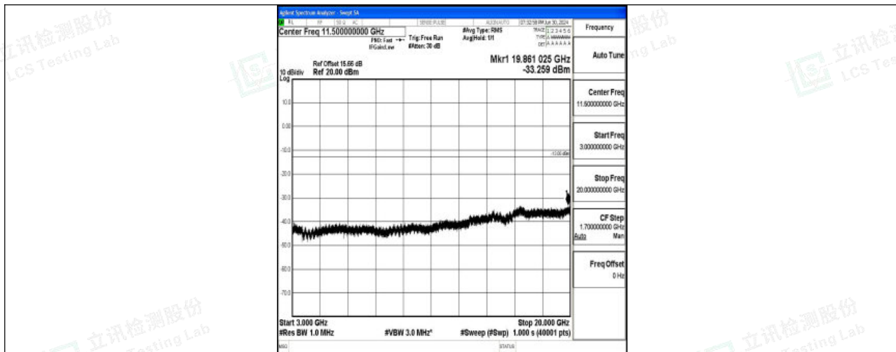
Band25_5MHz_QPSK_26065_1RB#0_3000~20000_3000~20000
