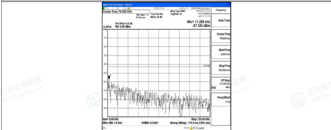
Band25_15MHz_16QAM_26115_1RB#0_0.009~0.15_0.009~0.15
