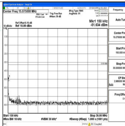
Band25_3MHz_QPSK_26055_1RB#0_0.15~30_0.15~30
