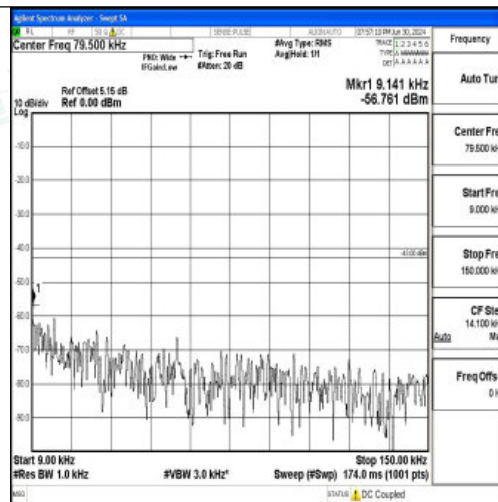
Band25_10MHz_QPSK_26365_1RB#0_0.009~0.15_0.009~0.15
