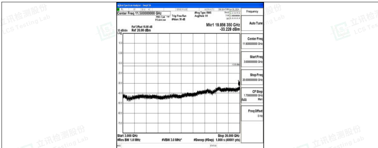
Band25_15MHz_QPSK_26115_1RB#0_3000~20000_3000~20000
