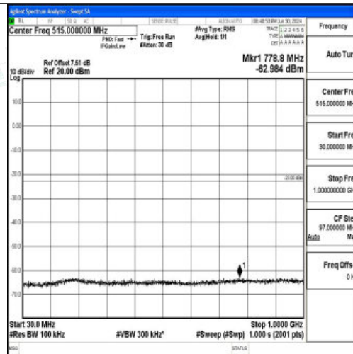
Band25_20MHz_16QAM_26140_1RB#0_30~1000_30~1000
