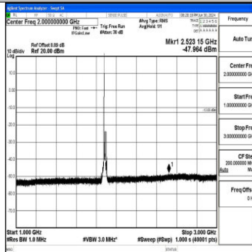
Band25_15MHz_16QAM_26365_1RB#0_1000~3000_1000~3000
