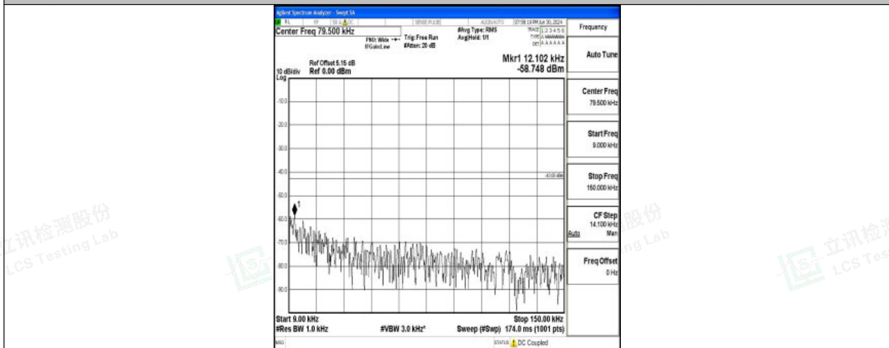
Band25_10MHz_QPSK_26640_1RB#0_0.009~0.15_0.009~0.15
