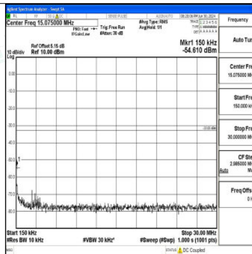
Band25_15MHz_16QAM_26365_1RB#0_0.15~30_0.15~30
