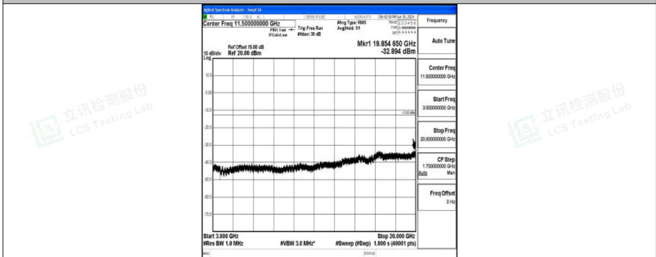
Band25_20MHz_QPSK_26590_1RB#0_3000~20000_3000~20000
