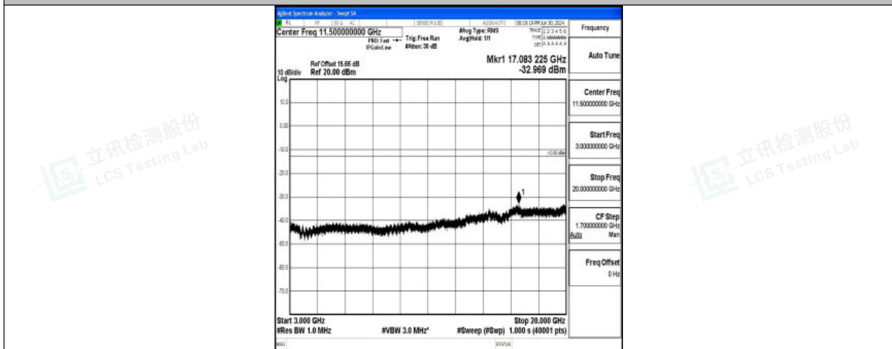
Band25_15MHz_16QAM_26115_1RB#0_3000~20000_3000~20000
