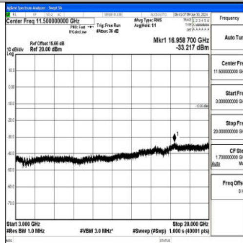
Band25_20MHz_16QAM_26140_1RB#0_3000~20000_3000~20000
