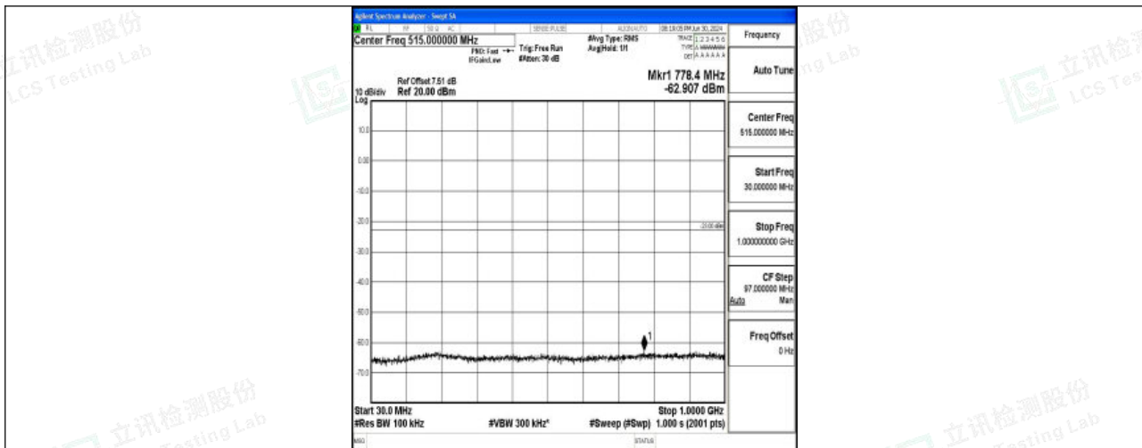
Band25_15MHz_16QAM_26115_1RB#0_30~1000_30~1000
