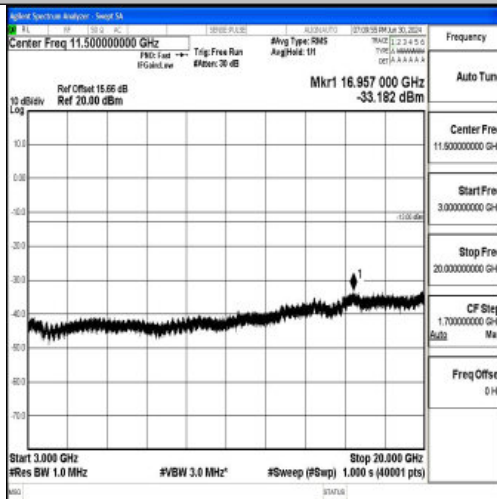
Band25_3MHz_16QAM_26055_1RB#0_3000~20000_3000~20000
