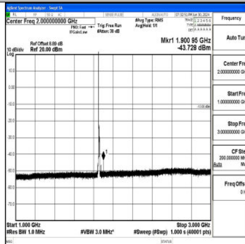
Band25_5MHz_QPSK_26065_1RB#0_1000~3000_1000~3000
