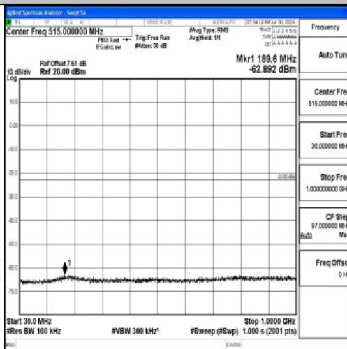
Band25_5MHz_16QAM_26365_1RB#0_30~1000_30~1000
