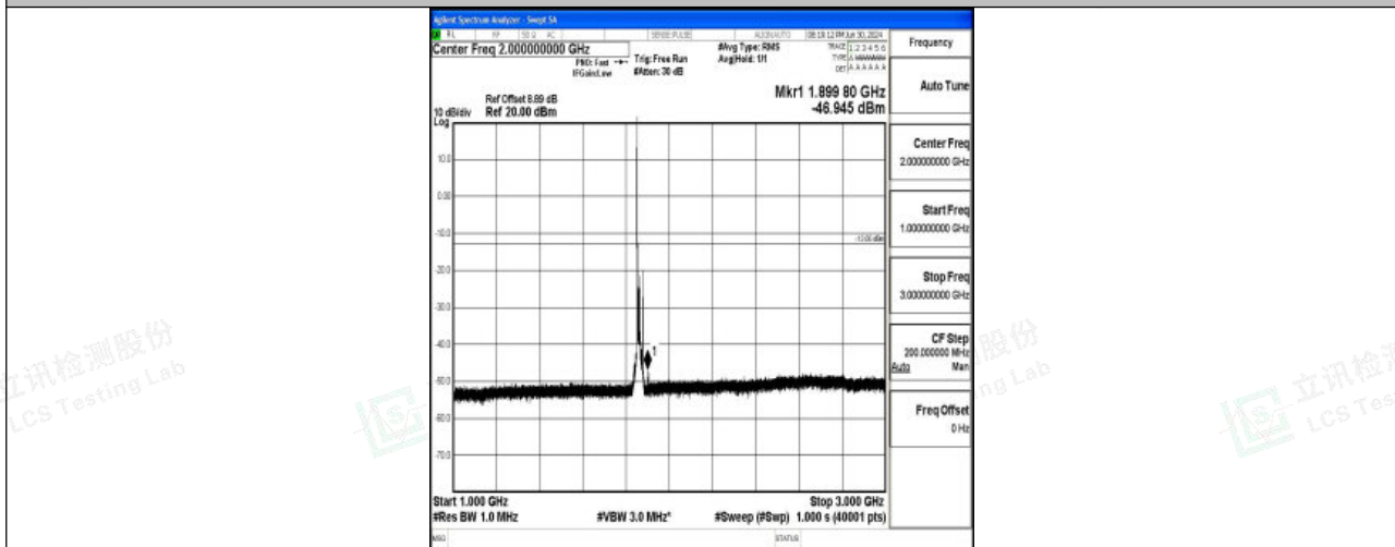
Band25_15MHz_16QAM_26115_1RB#0_1000~3000_1000~3000
