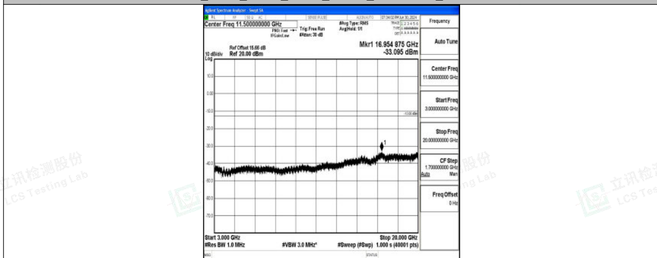
Band25_5MHz_QPSK_26365_1RB#0_3000~20000_3000~20000
