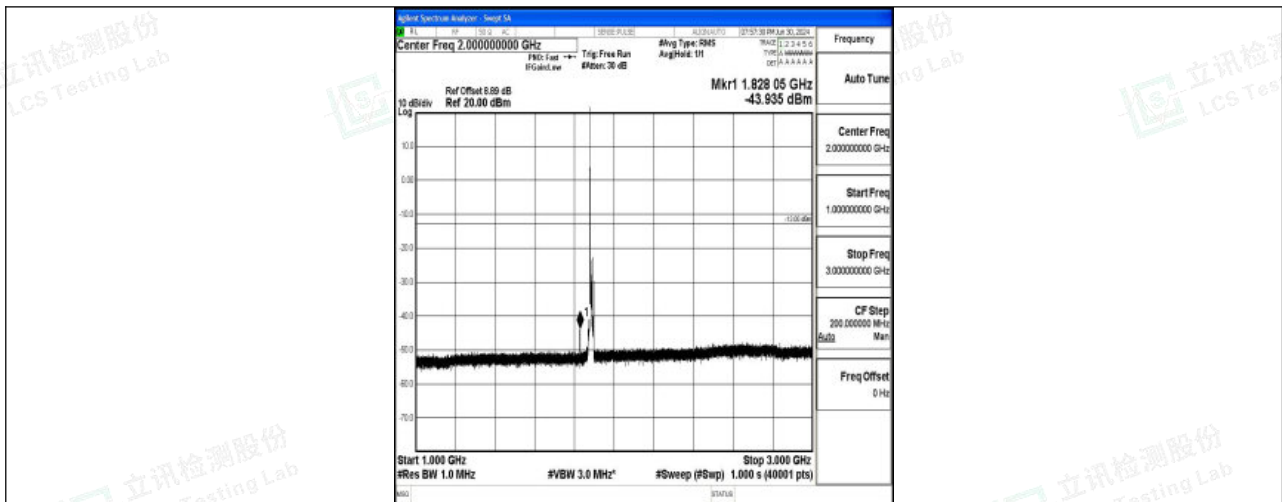
Band25_10MHz_QPSK_26365_1RB#0_1000~3000_1000~3000
