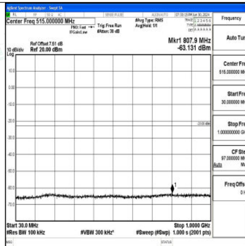
Band25_5MHz_16QAM_26065_1RB#0_30~1000_30~1000
