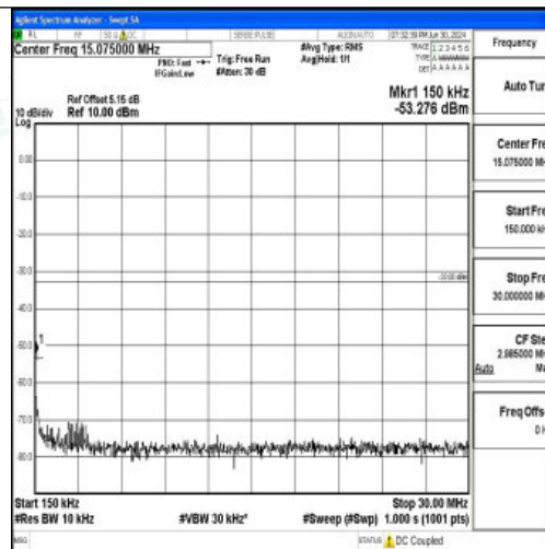
Band25_5MHz_QPSK_26065_1RB#0_0.15~30_0.15~30
