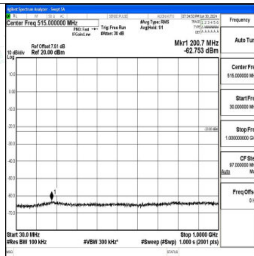
Band25_5MHz_QPSK_26665_1RB#0_30~1000_30~1000
