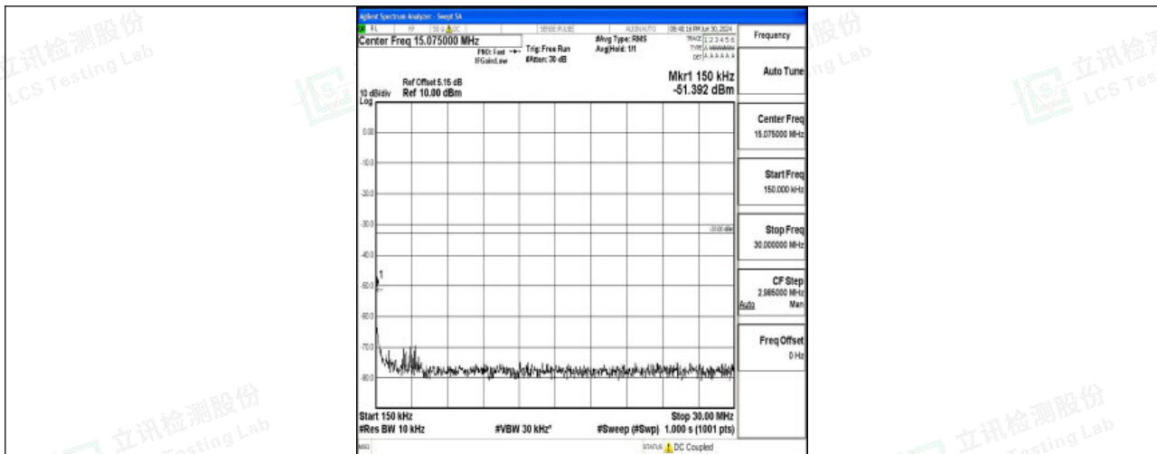
Band25_20MHz_QPSK_26140_1RB#0_0.15~30_0.15~30
