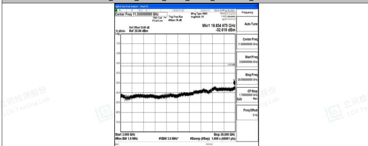
Band25_15MHz_16QAM_26615_1RB#0_3000~20000_3000~20000
