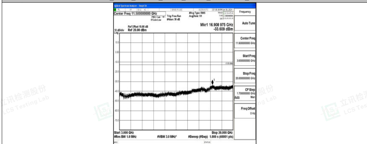
Band25_5MHz_16QAM_26665_1RB#0_3000~20000_3000~20000
