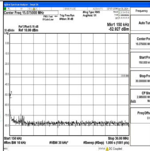
Band25_10MHz_QPSK_26365_1RB#0_0.15~30_0.15~30
