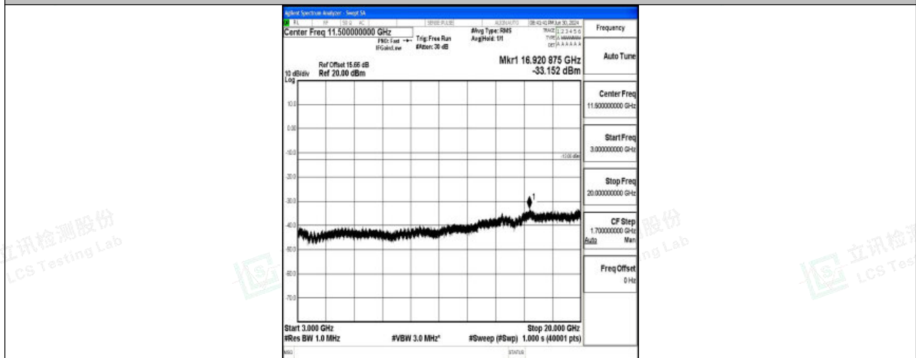
Band25_20MHz_QPSK_26365_1RB#0_3000~20000_3000~20000
