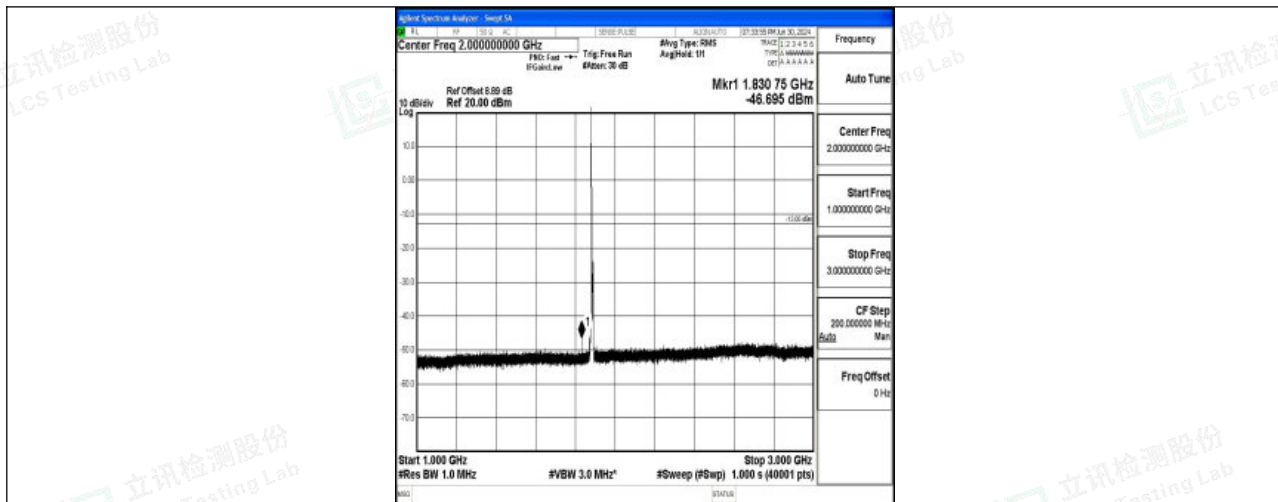
Band25_5MHz_QPSK_26365_1RB#0_1000~3000_1000~3000
