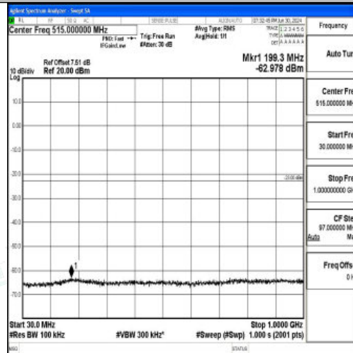
Band25_5MHz_QPSK_26065_1RB#0_30~1000_30~1000
