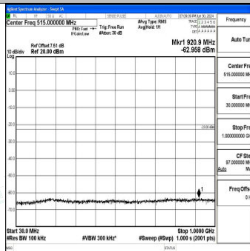
Band25_3MHz_QPSK_26055_1RB#0_30~1000_30~1000
