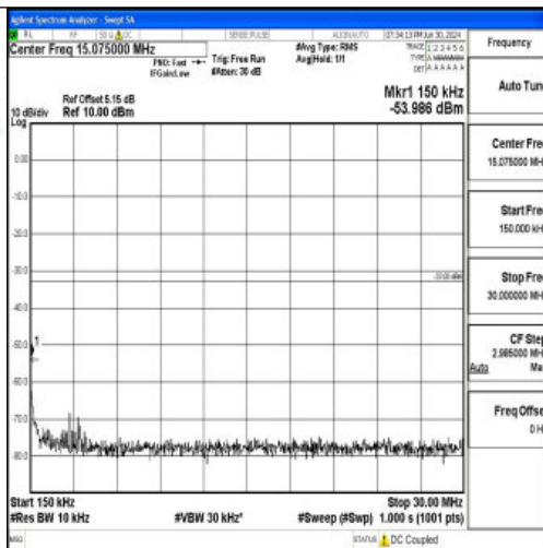
Band25_5MHz_16QAM_26365_1RB#0_0.15~30_0.15~30
