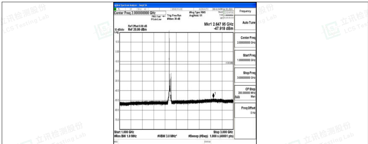
Band25_20MHz_QPSK_26365_1RB#0_1000~3000_1000~3000
