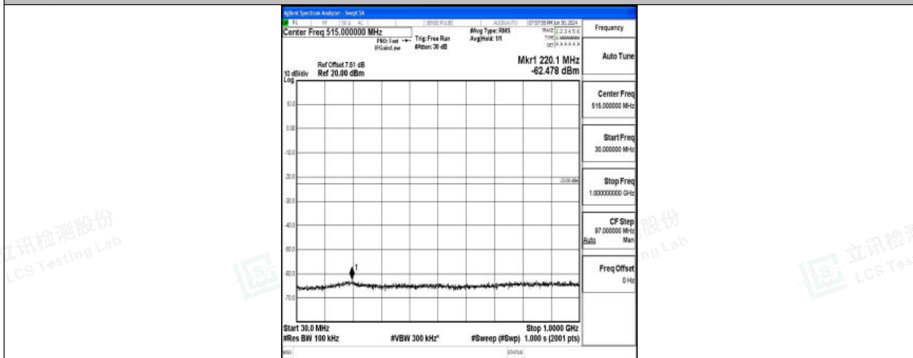
Band25_10MHz_16QAM_26365_1RB#0_30~1000_30~1000
