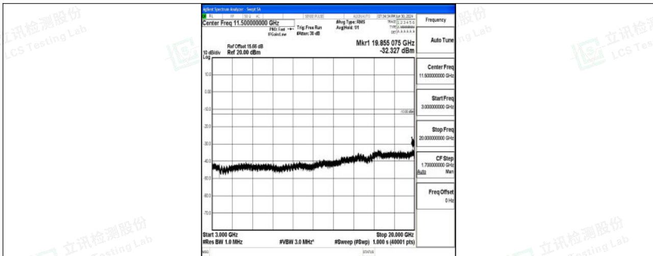
Band25_5MHz_16QAM_26365_1RB#0_3000~20000_3000~20000
