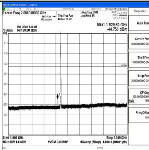
Band25_5MHz_16QAM_26365_1RB#0_1000~3000_1000~3000
