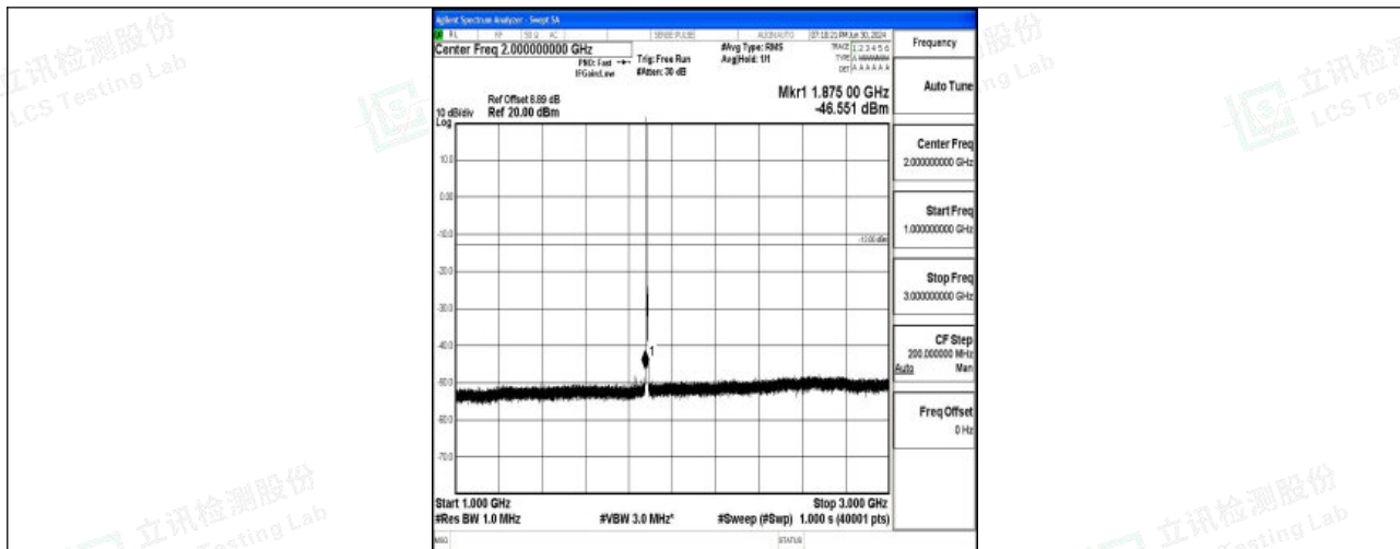
Band25_3MHz_QPSK_26365_1RB#0_1000~3000_1000~3000
