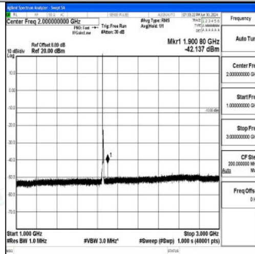
Band25_5MHz_16QAM_26065_1RB#0_1000~3000_1000~3000
