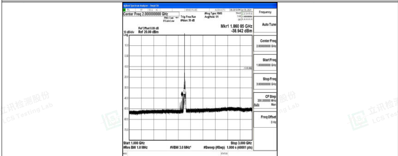
Band25_15MHz_QPSK_26615_1RB#0_1000~3000_1000~3000
