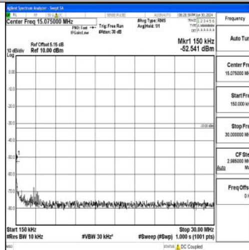
Band25_15MHz_QPSK_26615_1RB#0_0.15~30_0.15~30
