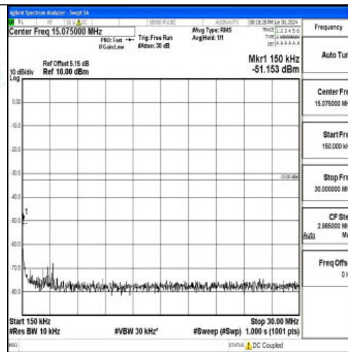
Band25_15MHz_QPSK_26115_1RB#0_0.15~30_0.15~30
