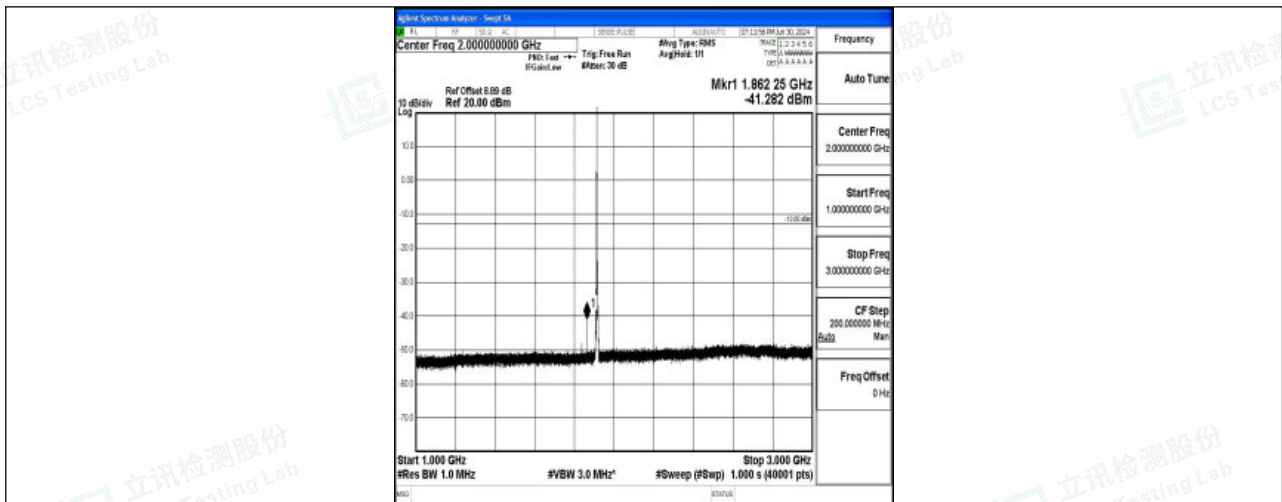
Band25_3MHz_16QAM_26675_1RB#0_1000~3000_1000~3000
