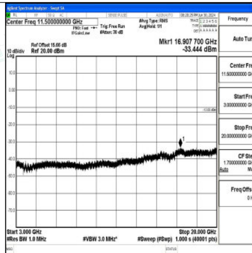
Band25_15MHz_16QAM_26365_1RB#0_3000~20000_3000~20000
