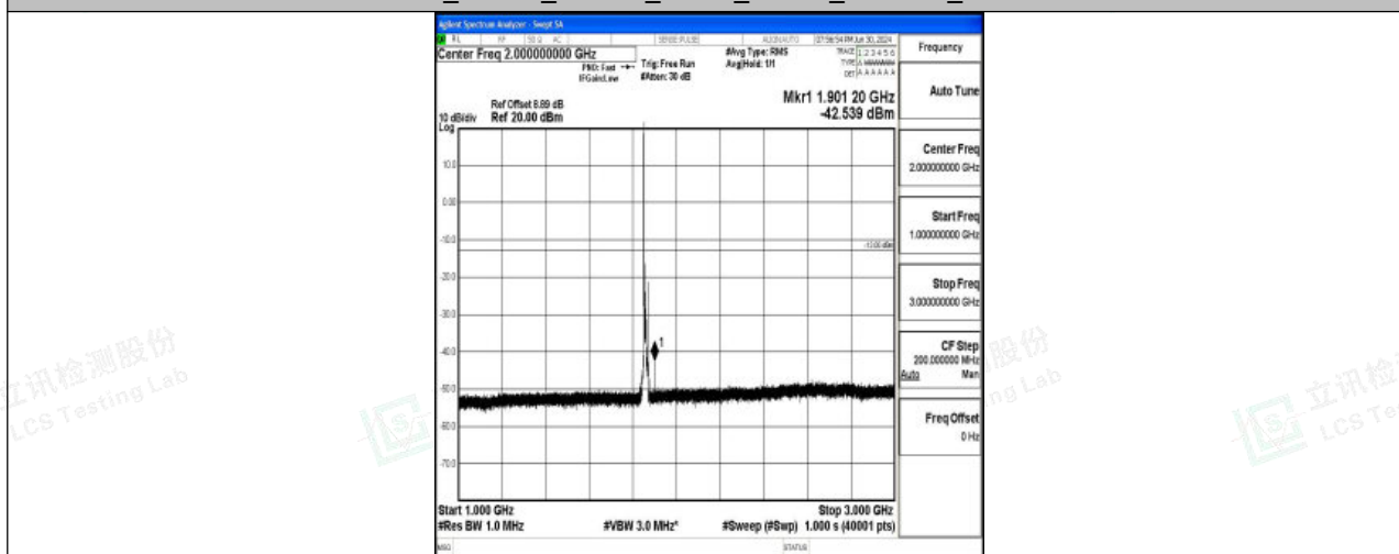
Band25_10MHz_16QAM_26090_1RB#0_1000~3000_1000~3000
