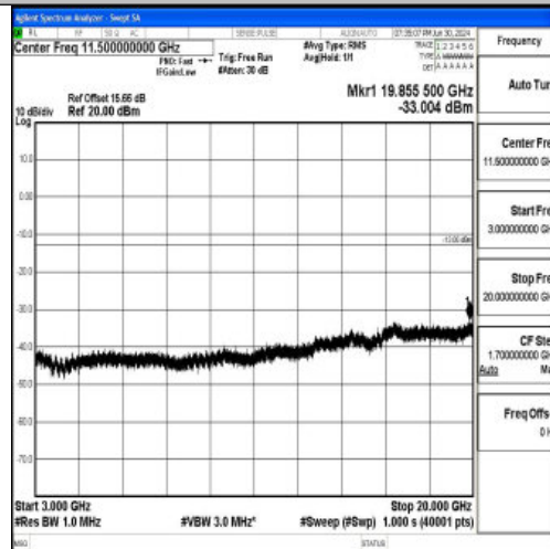
Band25_5MHz_QPSK_26665_1RB#0_3000~20000_3000~20000
