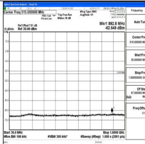
Band25_15MHz_16QAM_26365_1RB#0_30~1000_30~1000
