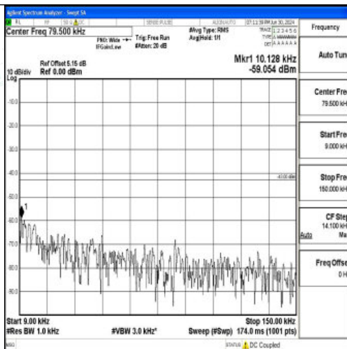
Band25_3MHz_16QAM_26675_1RB#0_0.009~0.15_0.009~0.15
