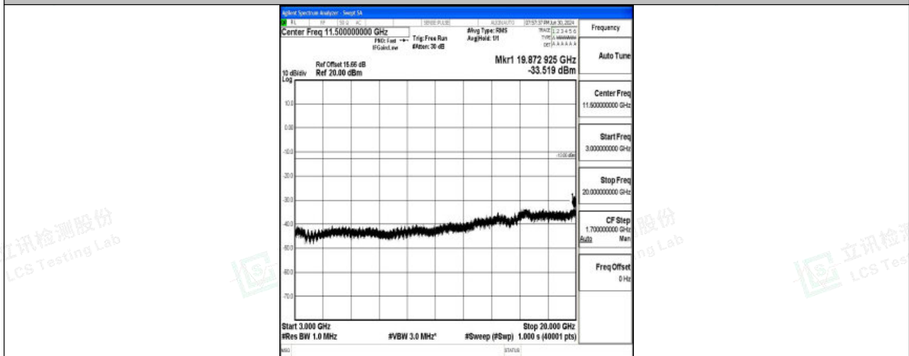
Band25_10MHz_QPSK_26365_1RB#0_3000~20000_3000~20000
