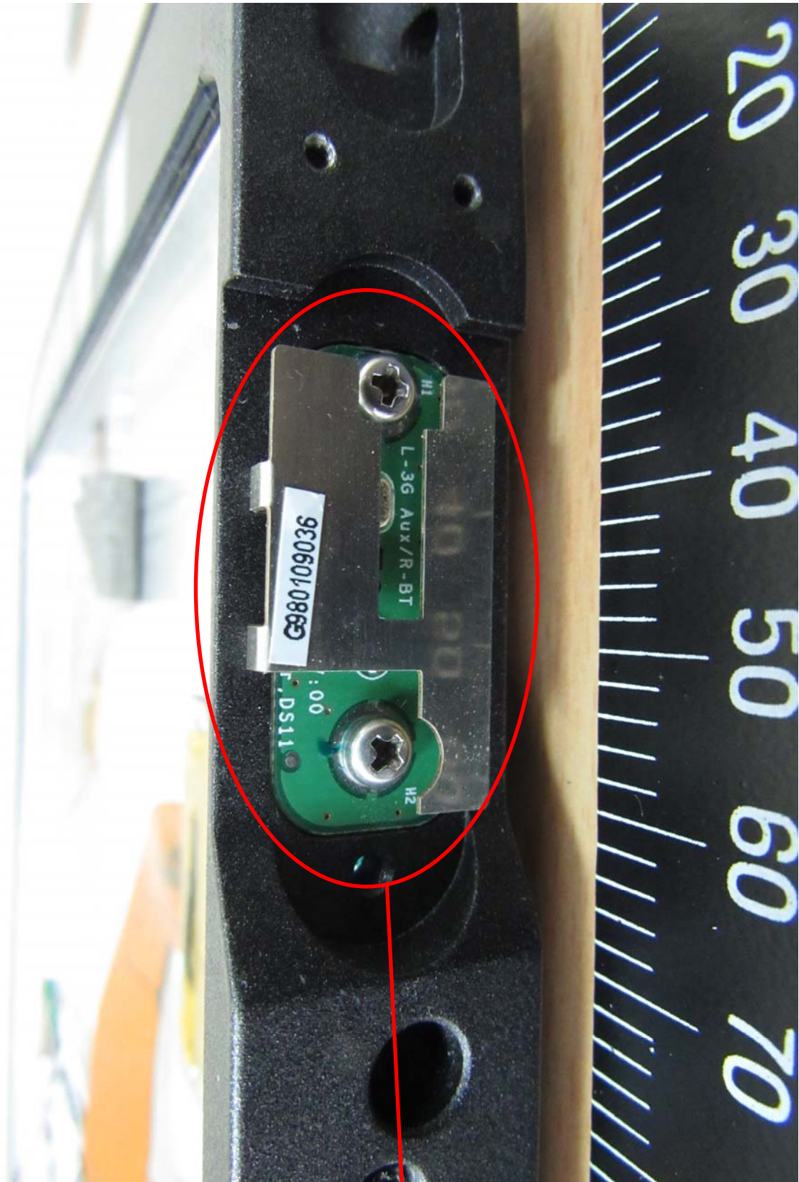
ANT B (2.4G_WLAN、BT): PIFA antenna / 3.49 dBi ANT B (5G_WLAN): PIFA antenna / 4.33 dBi
