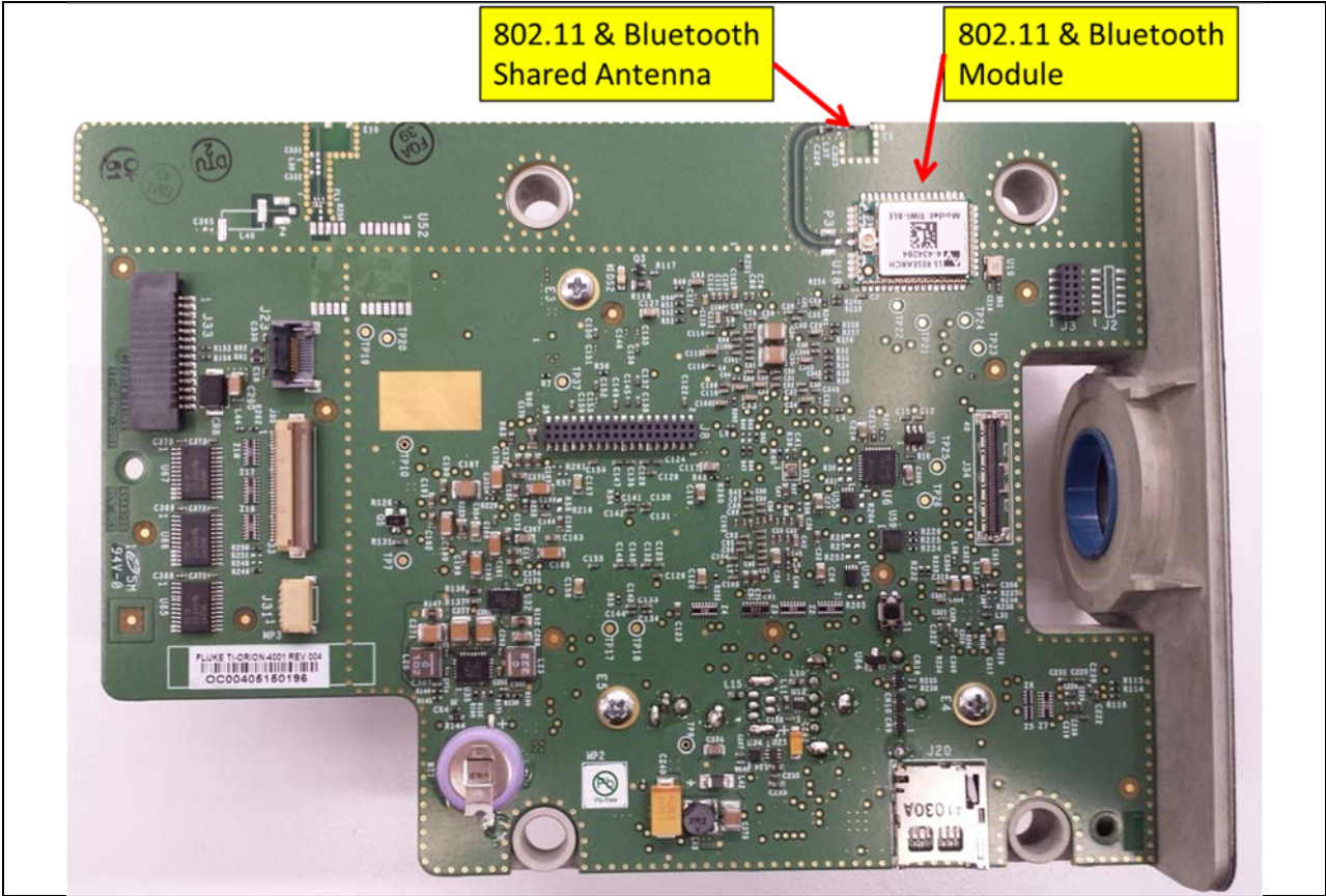
Figure 4 TiX560 Series Main Processing Circuit Board (Top Side with EMC Shield)
