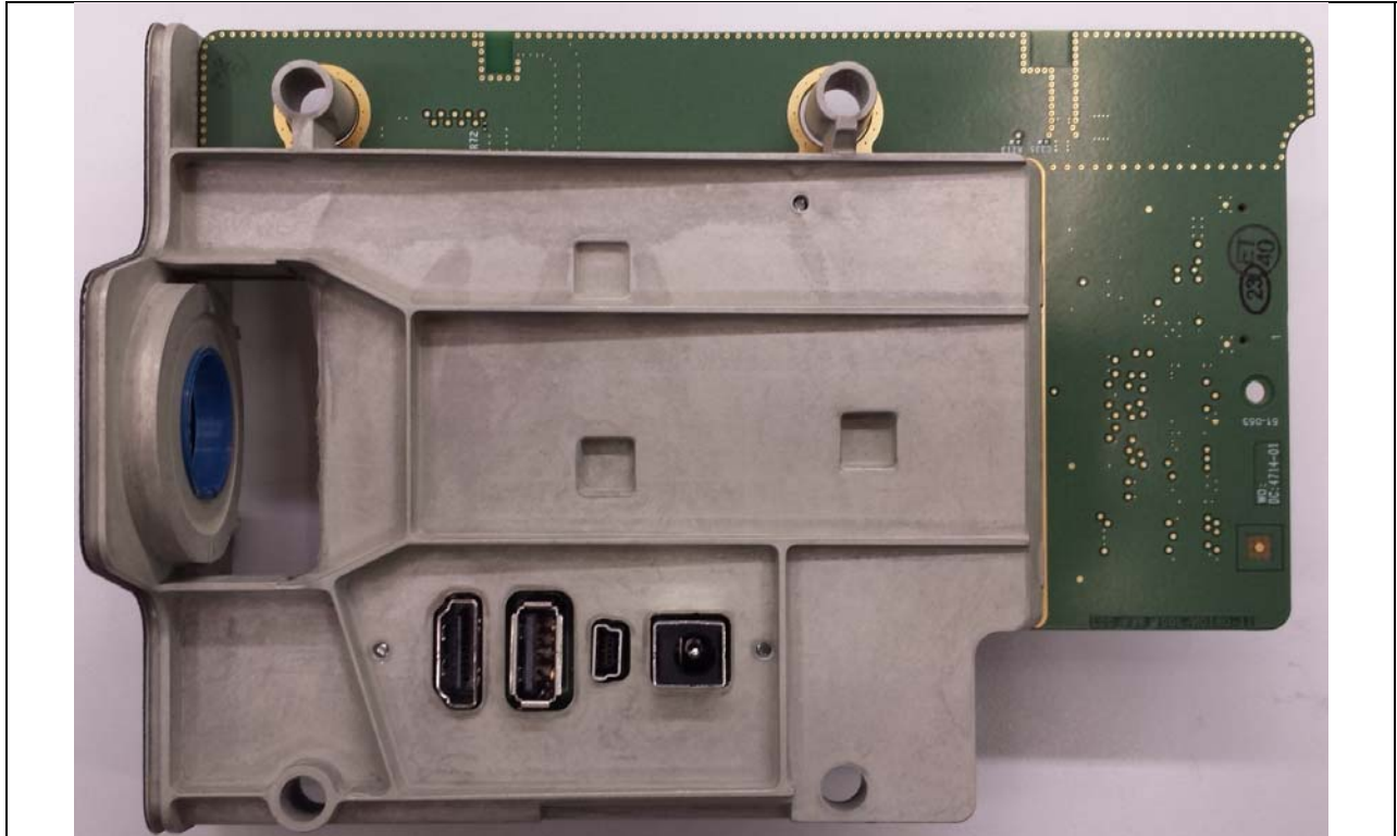
Figure 3 TiX560 Series Main Processing Circuit Board (Bottom Side with EMC Enclosure)
