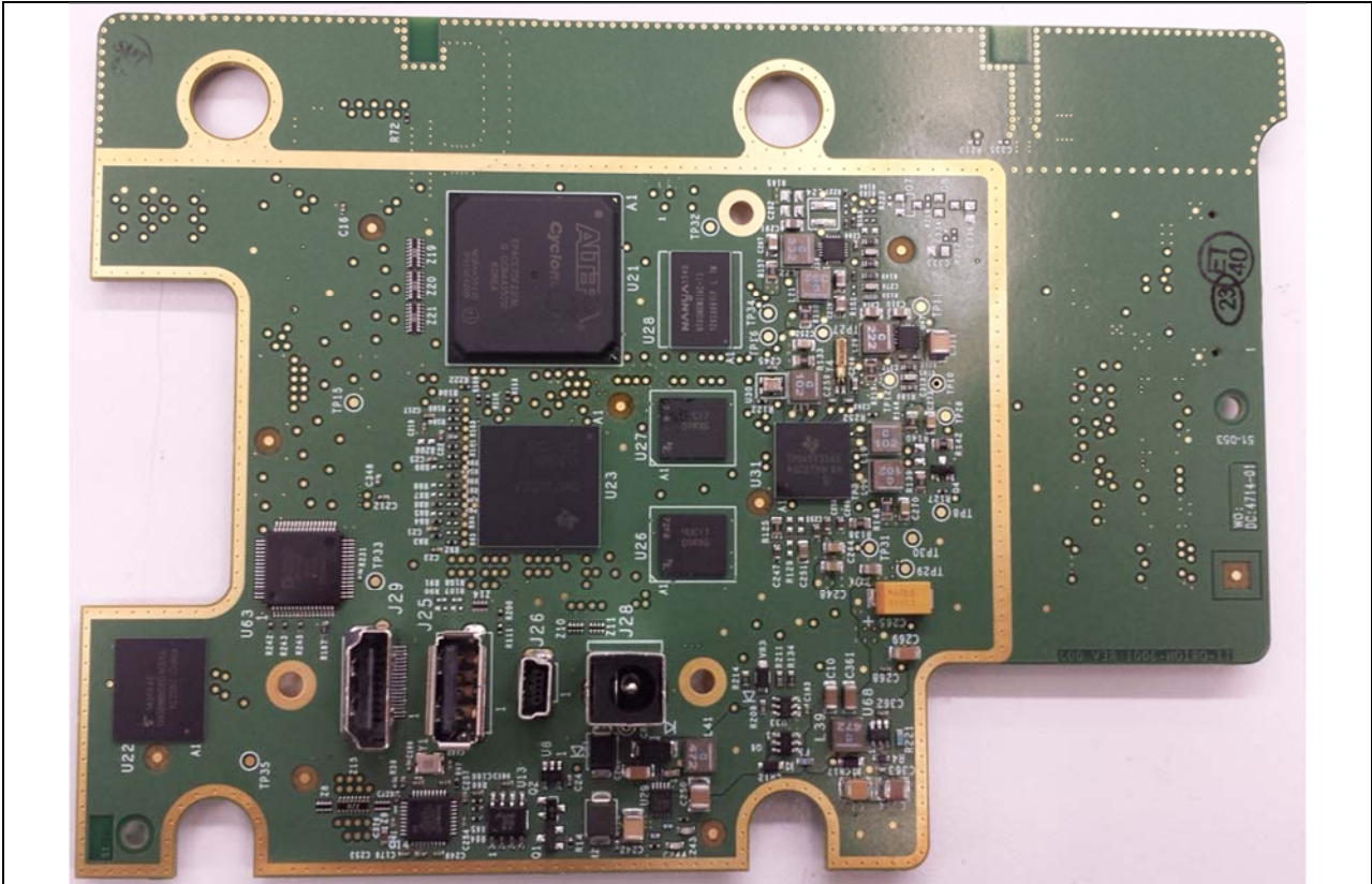
Figure 2 TiX560 Series Main Processing Circuit Board (Bottom Side)
