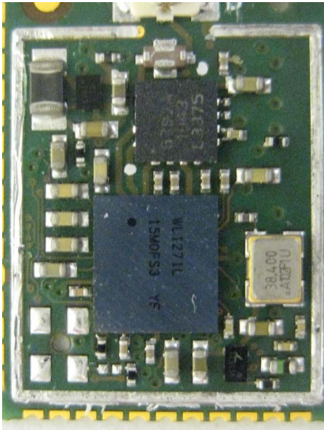
Figure 4 TiX560 Series Main Processing Circuit Board (Top Side with EMC Shield)
