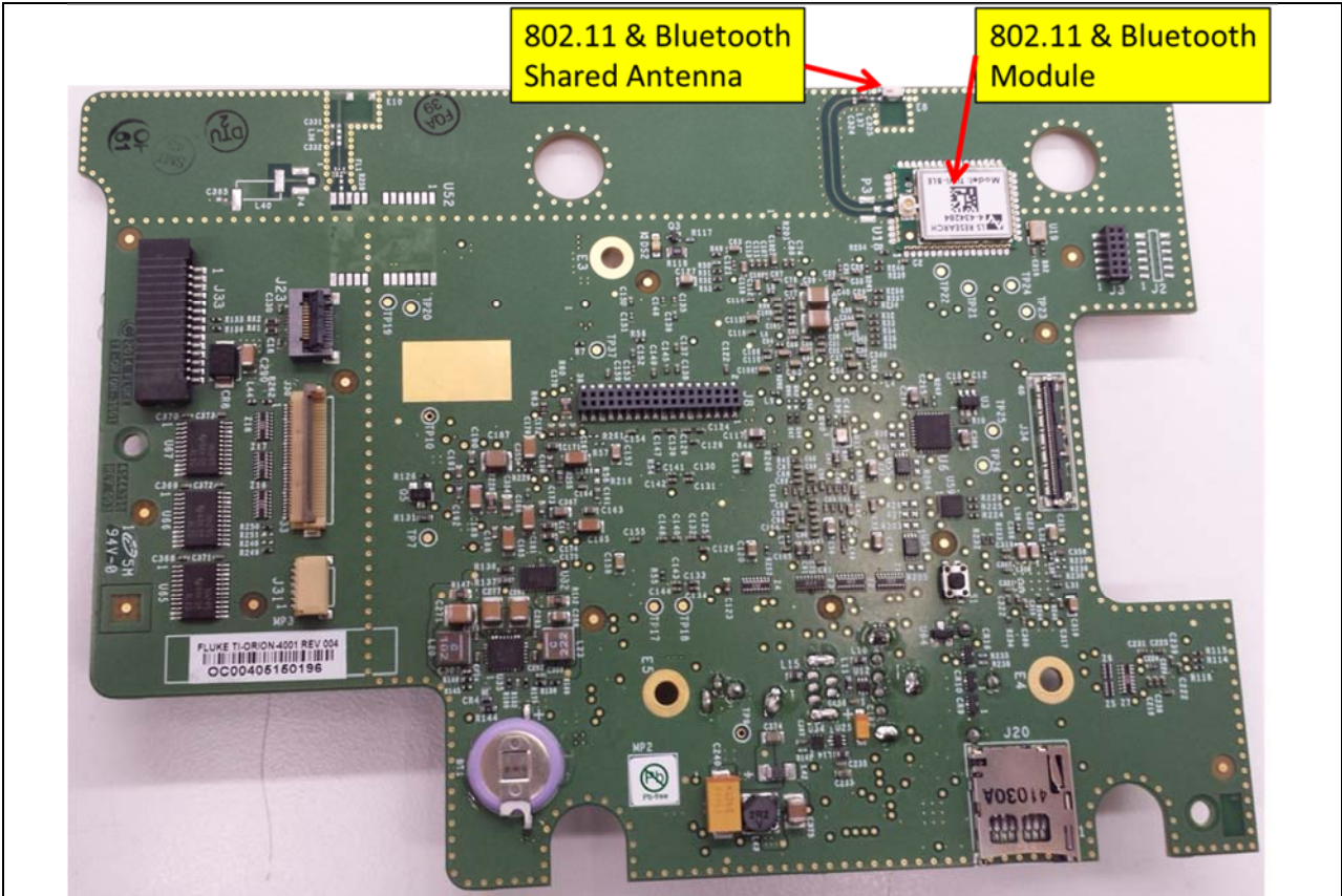
Figure 1 TiX560 Series Main Processing Circuit Board (Top Side)
