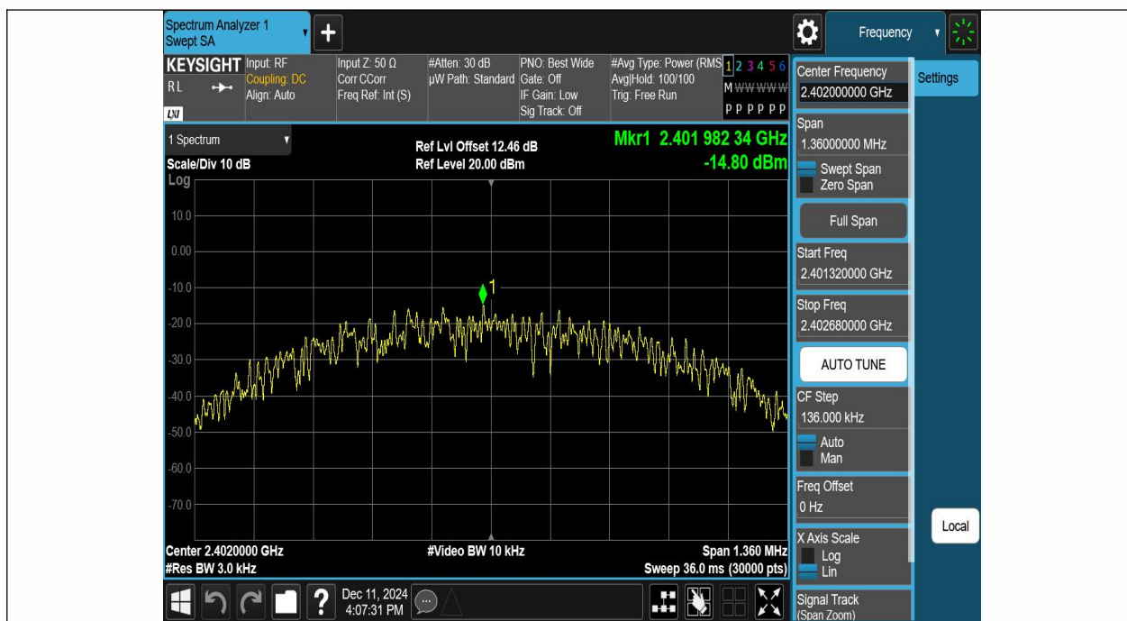
2.4G DTS MIMO-Ant1-2402-PASS
