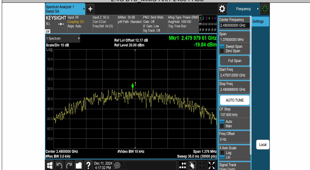
2.4G DTS MIMO-Ant2-2480-PASS
