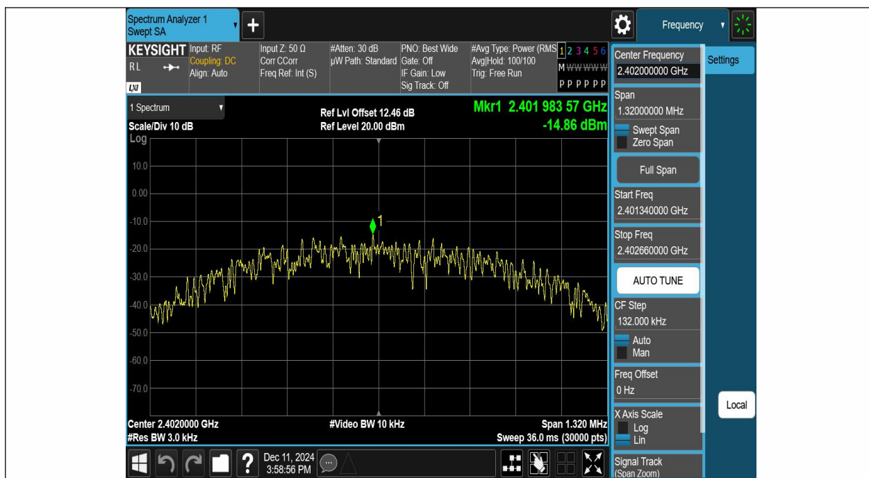
2.4G DTS-Ant1-2402-PASS
