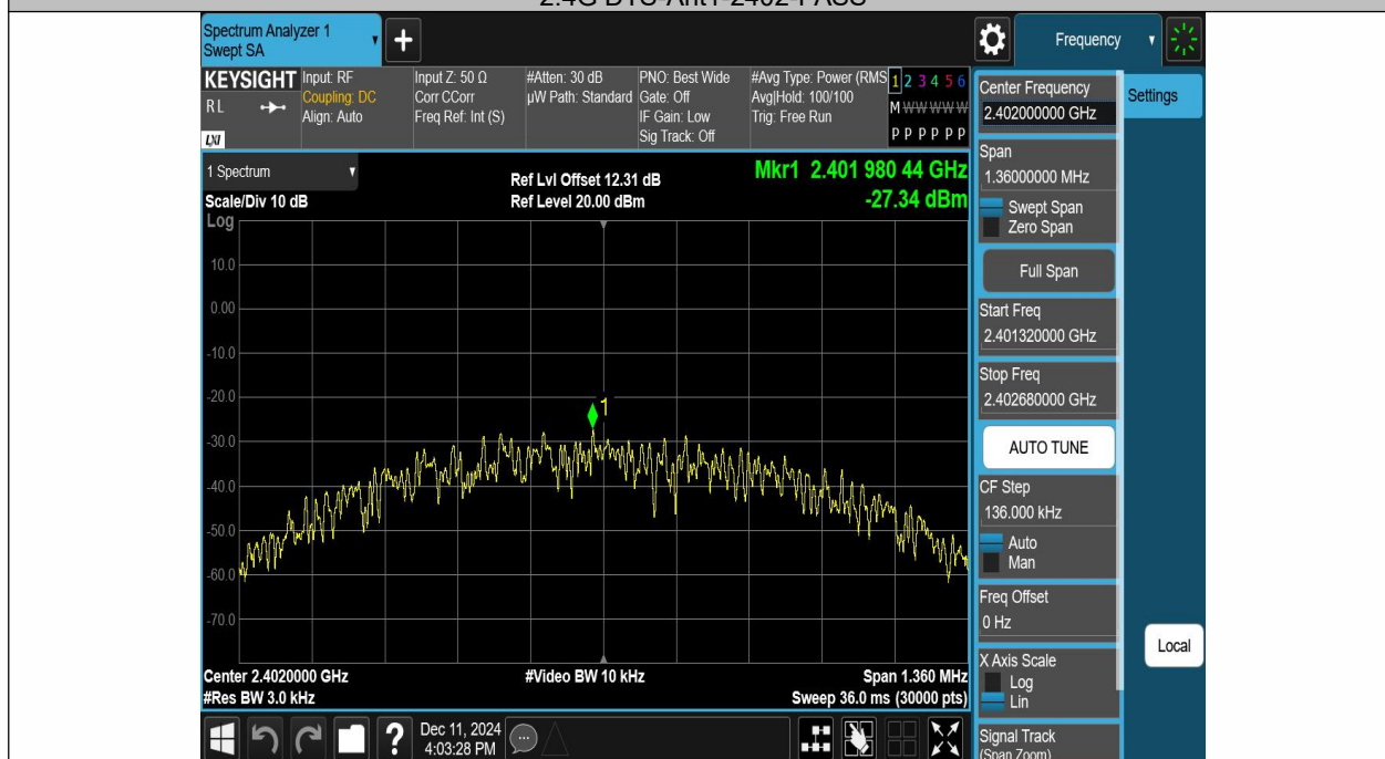
2.4G DTS-Ant2-2402-PASS
