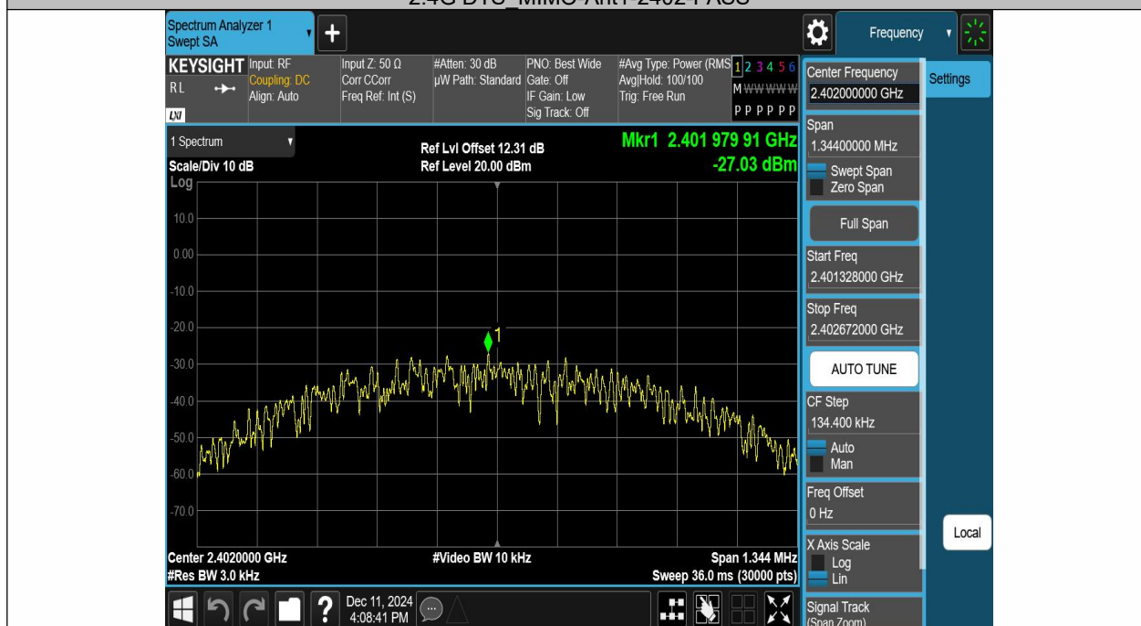
2.4G DTS MIMO-Ant2-2402-PASS
