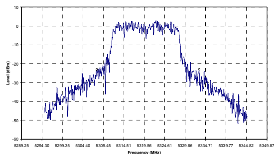
CISCO WLAN abg Setting: 14.0 & 0.54 Mbps, Frequency = 5320 MHz, Mode a, -26 dB Emission Bandwidth = 25.35 MHz with an RBW of 300 kHz
