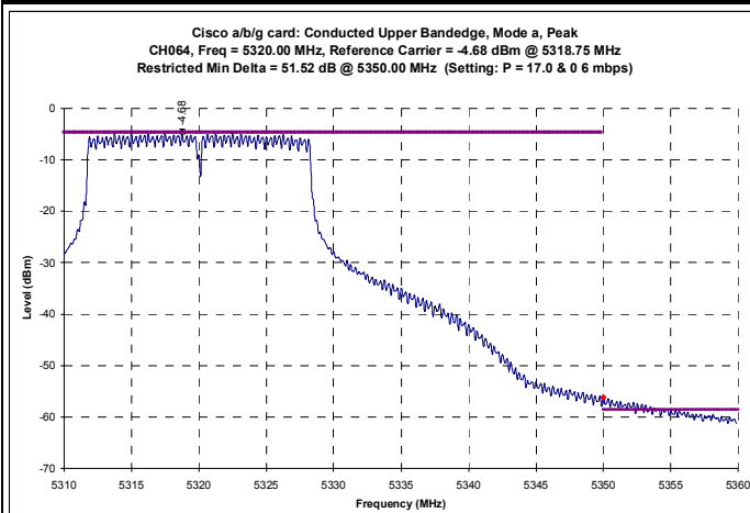
Channel 64 Mode a - Conducted Peak Band-edge Plots
