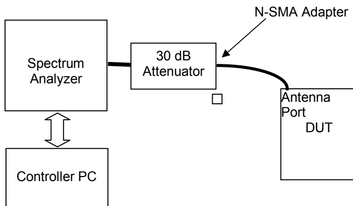
Figure I.6-1 - Setup Drawing
