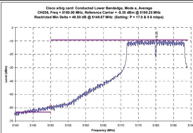
Channel 36 Mode a - Conducted Average Band-edge Plots
