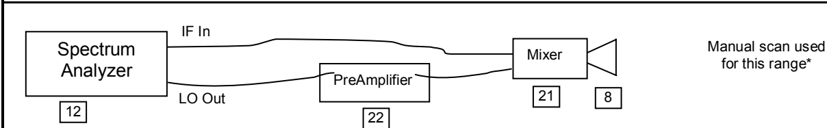
Figure G.6-2 - Setup Drawing ( \geq 26.5 GHz)
