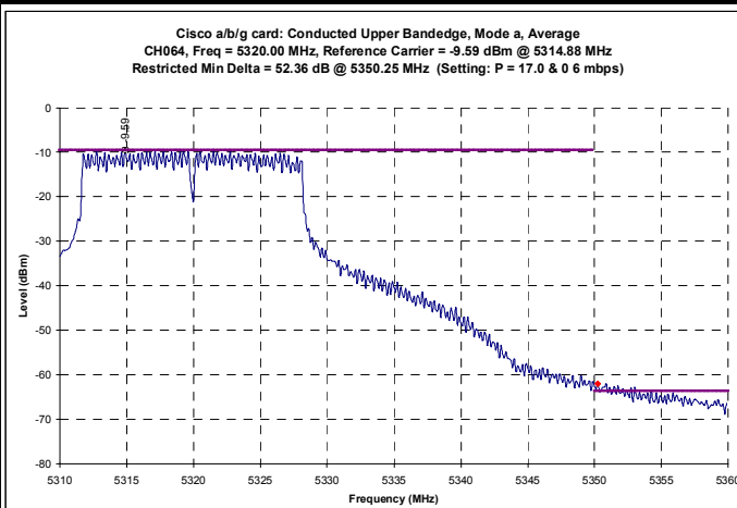
Channel 64 Mode a - Conducted Average Band-edge Plots
