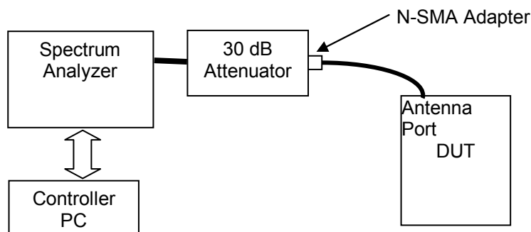
Figure D.6-1 - Setup Drawing
