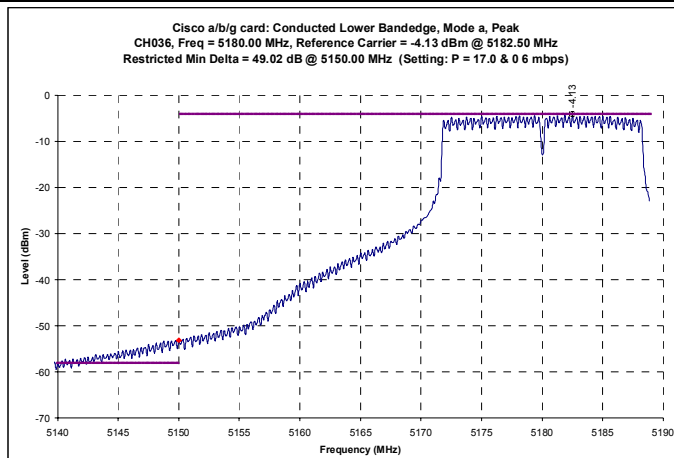
Channel 36 Mode a - Conducted Peak Band-edge Plots
