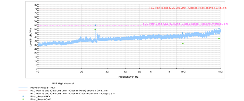
Figure 8.7-10: Radiated Spurious emissions 1 - 18 GHz, high channel
