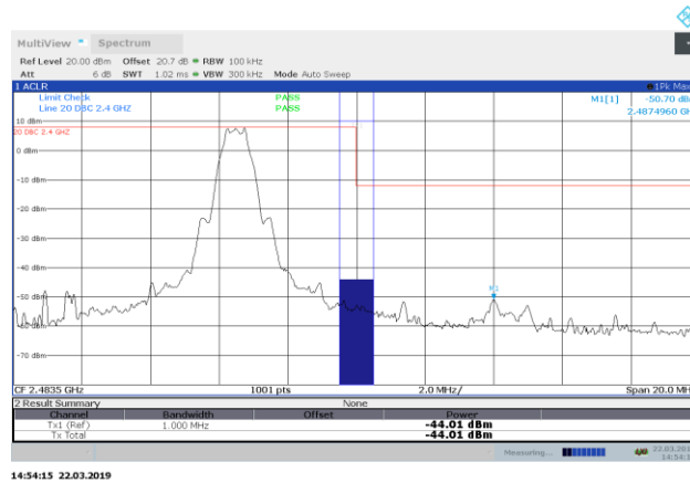
Figure 8.7-15: Conducted band edge emissions, high channel
