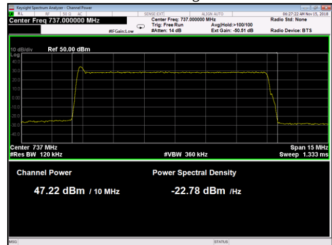
LTE10 Middle Channel Average Power
