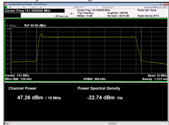
LTE10 Top Channel Average Power
