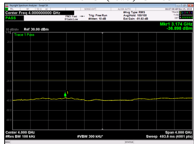
LTE10 Bottom+NB IoT GB (Lower) 2GHz-6GHz
