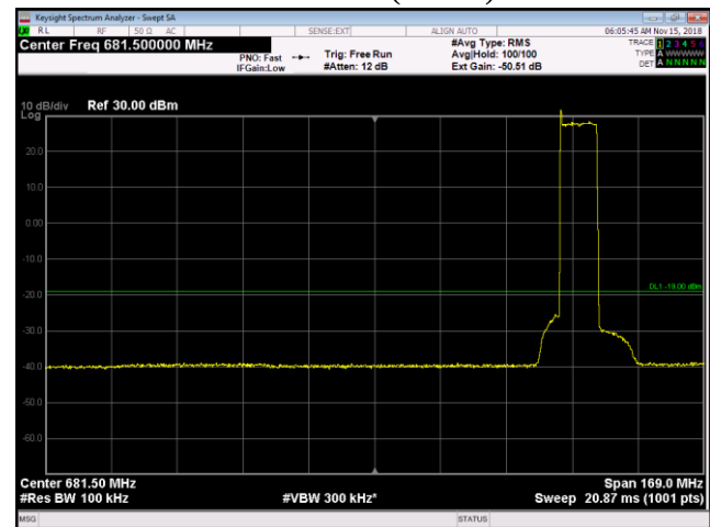
LTE10 Bottom+NB IoT GB (Lower) 597MHz-766MHz
