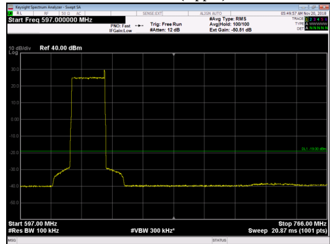
LTE20 Middle+NB IoT GB (Upper) 597MHz-766MHz
