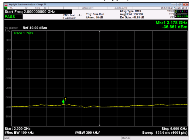
LTE20 Middle+NB IoT GB (Upper) 2GHz-6GHz
