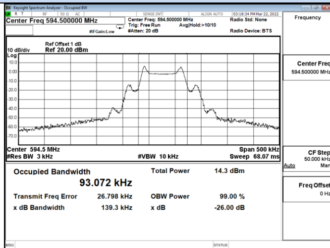
Channel 14/ 594.5 MHz
