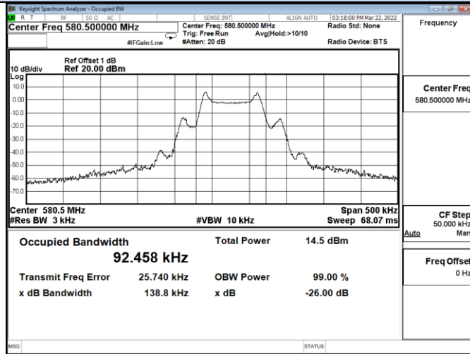
Channel 0 / 580.5MHz
