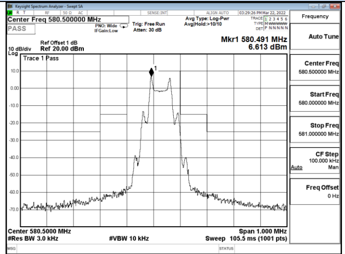
Channel 15 / 580.5MHz
