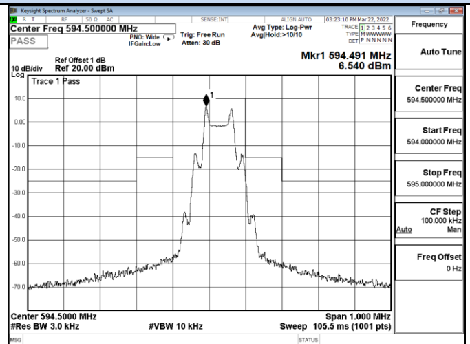
Channel 29 / 594.5 MHz
