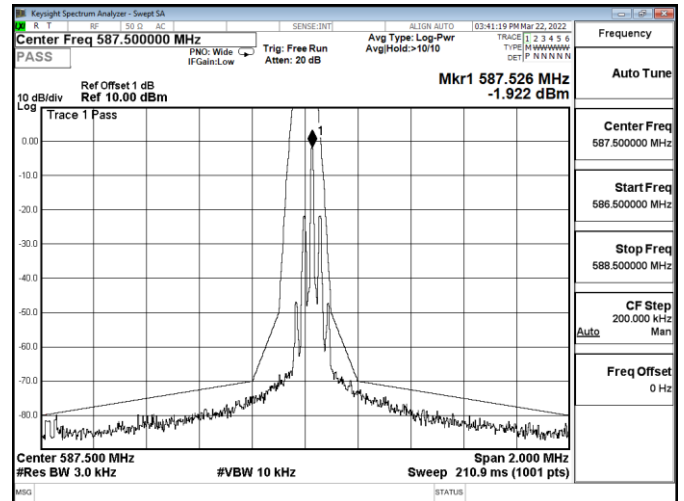
Channel 7/ 587.5 MHz
