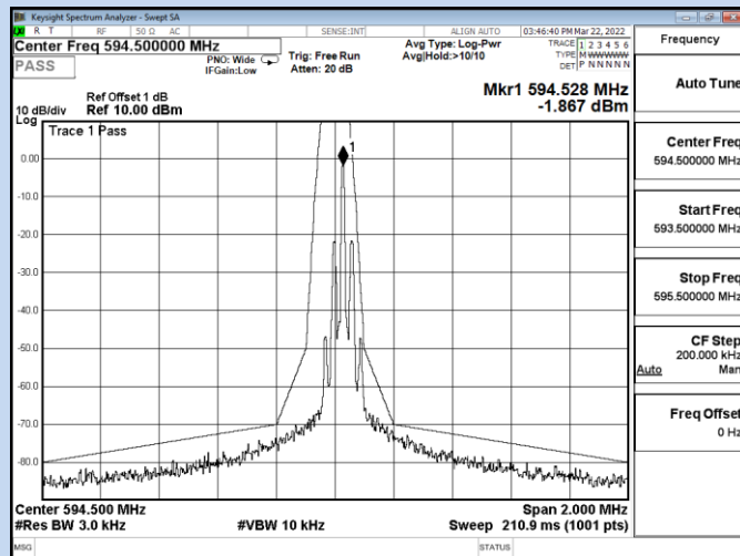
Channel 14/ 594.5 MHz
