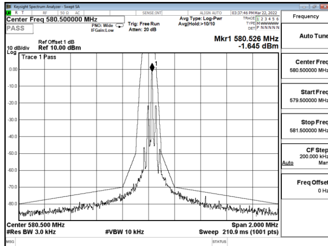
Channel 0/ 580.5 MHz
