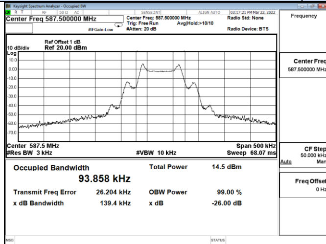
Channel 07 / 587.5 MHz
