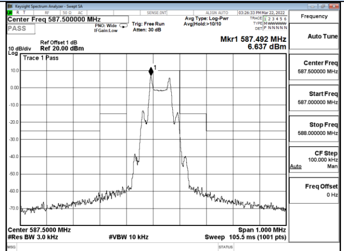
Channel 22 / 587.5 MHz
