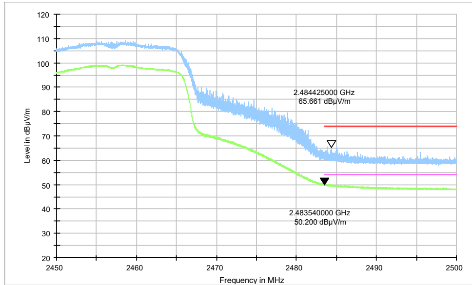
Fig.A.6.2.11 Transmitter Spurious Emission - Radiated (Power): 802.11n-HT20, ch10, 2.45 GHz - 2.50GHz
