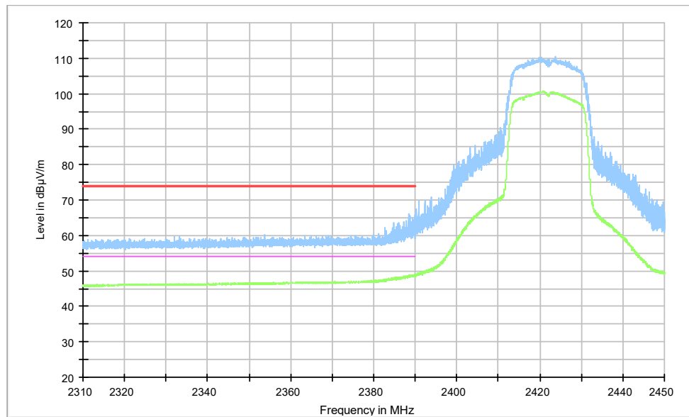
Fig.A.6.2.10 Transmitter Spurious Emission - Radiated (Power): 802.11n-HT20, ch3, 2.31 GHz - 2.45GHz
