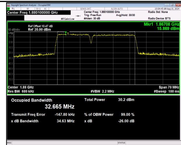
2-2-15MHz-20MHz-16QAM-16QAM-18803-18974-75RB#0 -100RB#0-PASS
