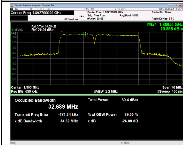
2-2-15MHz-20MHz-16QAM-16QAM-18929-19100-75RB#0 -100RB#0-PASS
