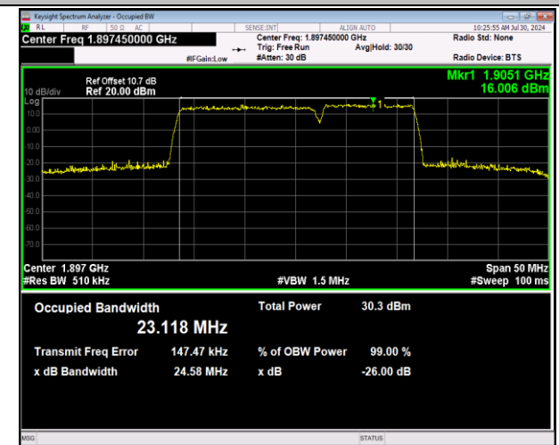
2-2-15MHz-10MHz-64QAM-64QAM-19027-19147-75RB#0-5 -50RB#0-PASS
