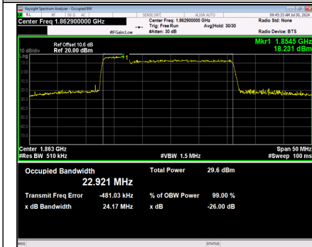
2-2-5MHz-20MHz-64QAM-64QAM-18633-18750-25RB#0-100RB#0-PASS
