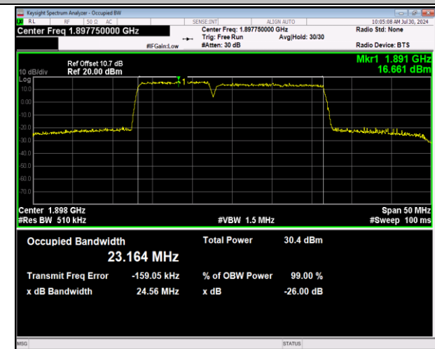
2-2-10MHz-15MHz-64QAM-64QAM-19005-19125-50RB#0-7 -75RB#0-PASS
