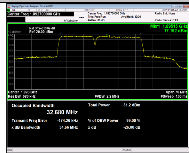
2-2-15MHz-20MHz-QPSK-QPSK-18929-19100-75RB#0-1 00RB#0-PASS
