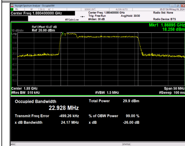
2-2-5MHz-20MHz-16QAM-16QAM-18808-18925-25RB#0-100RB#0-PASS
