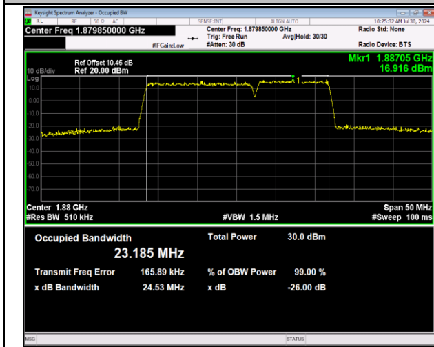
2-2-15MHz-10MHz-64QAM-64QAM-18851-18971-75RB#0-5 -50RB#0-PASS
