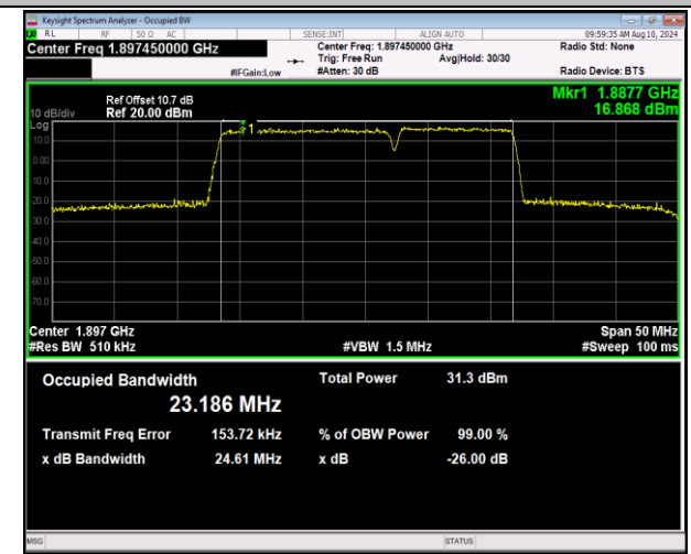
2-2-15MHz-10MHz-QPSK-QPSK-19027-19147-75RB#0-5 ORB#0-PASS
