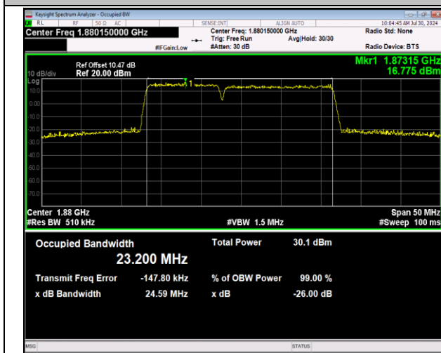
2-2-10MHz-15MHz-64QAM-64QAM-18829-18949-50RB#0-7 -75RB#0-PASS
