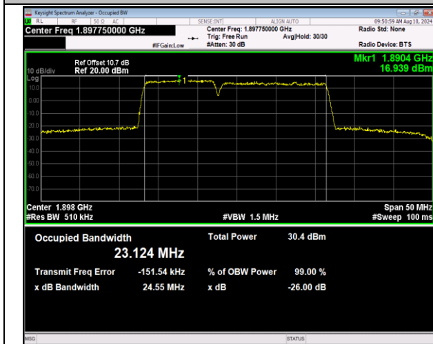
2-2-10MHz-15MHz-16QAM-16QAM-19005-19125-50RB#0-7 -75RB#0-PASS
