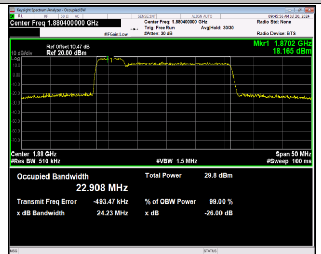
2-2-5MHz-20MHz-64QAM-64QAM-18808-18925-25RB#0-100RB#0-PASS
