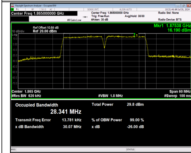
2-2-15MHz-15MHz-64QAM-64QAM-18675-18825-75RB#0-7 -75RB#0-PASS
