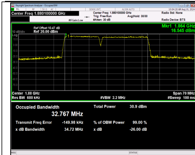
2-2-15MHz-20MHz-QPSK-QPSK-18803-18974-75RB#0-1 00RB#0-PASS
