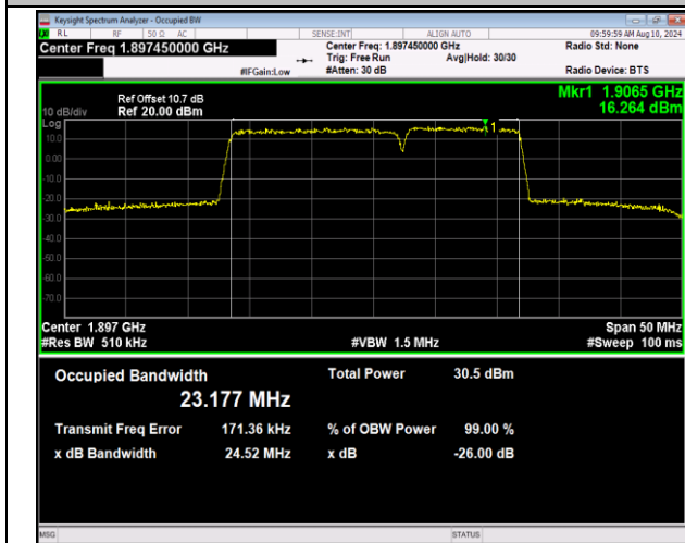
2-2-15MHz-10MHz-16QAM-16QAM-19027-19147-75RB#0-5 -50RB#0-PASS
