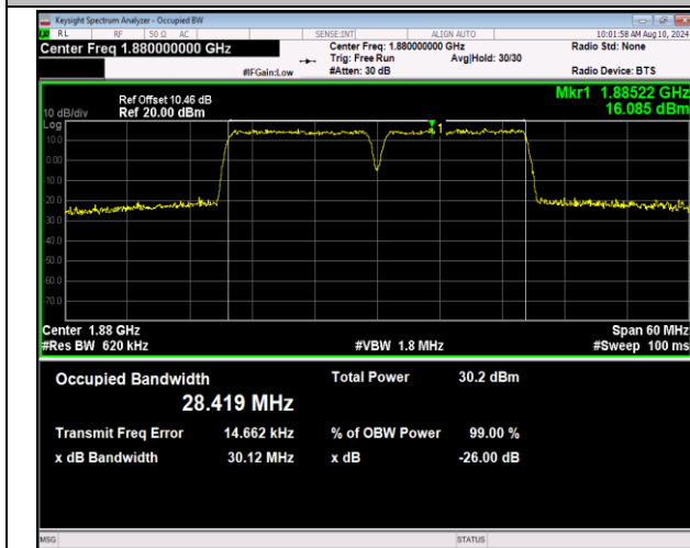
2-2-15MHz-15MHz-16QAM-16QAM-18825-18975-75RB#0-7 -75RB#0-PASS
