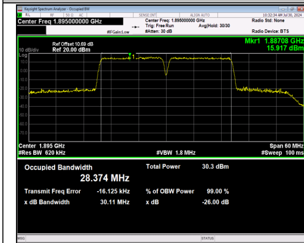
2-2-15MHz-15MHz-64QAM-64QAM-18975-19125-75RB#0-7 -75RB#0-PASS
