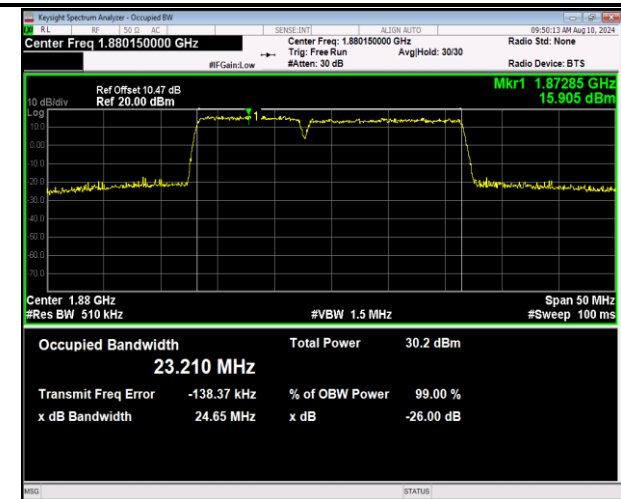
2-2-10MHz-15MHz-16QAM-16QAM-18829-18949-50RB#0-7 -75RB#0-PASS
