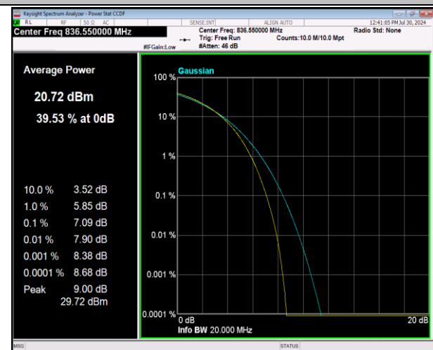
5-5-10MHz-10MHz-64QAM-64QAM-20476-20575-50RB#0-50RB#0-PASS
