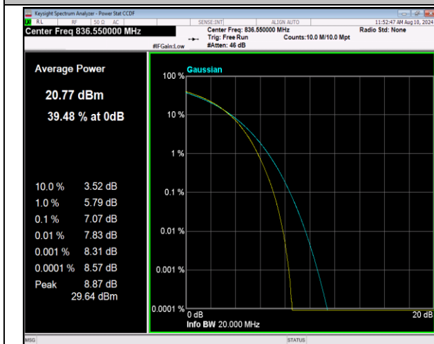
5-5-10MHz-10MHz-16QAM-16QAM-20476-20575-50RB#0-50RB#0-PASS
