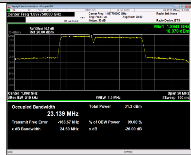
2-2-10MHz-15MHz-QPSK-QPSK-19005-19125-50RB#0-7 5RB#0-PASS
