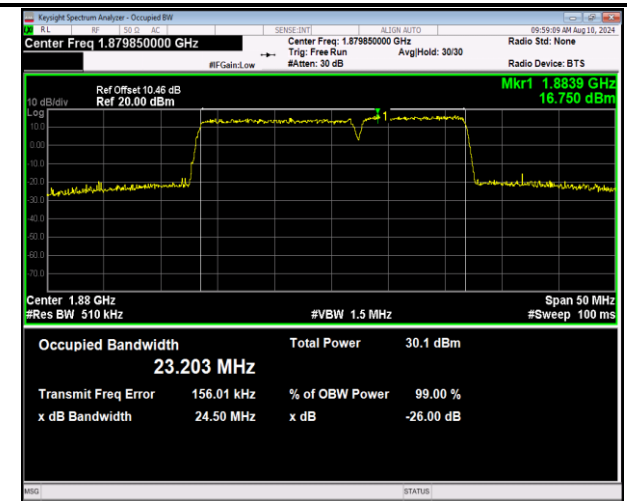
2-2-15MHz-10MHz-16QAM-16QAM-18851-18971-75RB#0-5 -50RB#0-PASS
