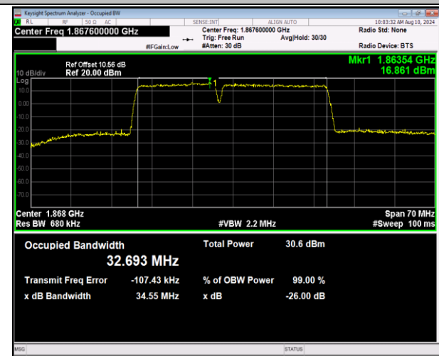
2-2-15MHz-20MHz-QPSK-QPSK-18678-18849-75RB#0-1 00RB#0-PASS
