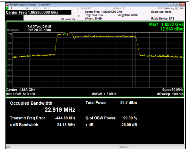
2-2-5MHz-20MHz-16QAM-16QAM-18633-18750-25RB#0-100RB#0-PASS
