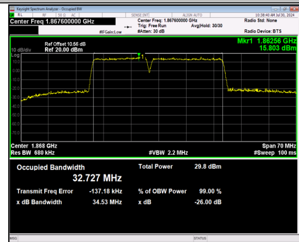
2-2-15MHz-20MHz-64QAM-64QAM-18678-18849-75RB#0-1 -100RB#0-PASS
