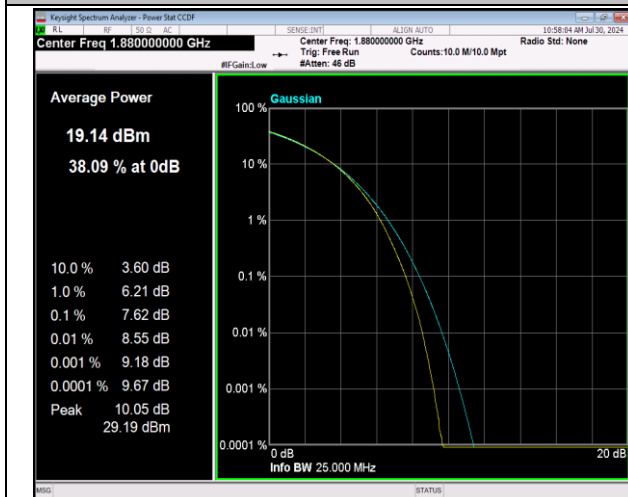
2-2-20MHz-20MHz-64QAM-64QAM-18801-18999-100RB#0-100RB#0-PASS
