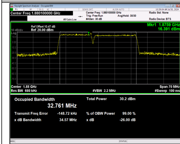
2-2-15MHz-20MHz-64QAM-64QAM-18803-18974-75RB#0 -100RB#0-PASS
