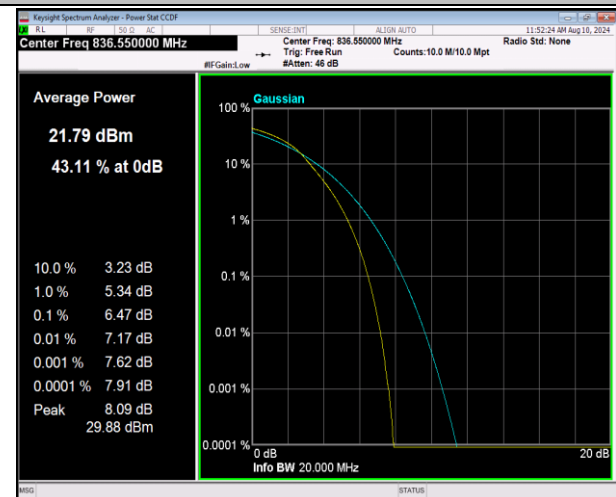
5-5-10MHz-10MHz-QPSK-QPSK-20476-20575-50RB#0-50RB#0-PASS
