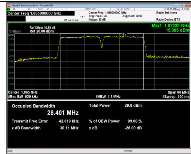
2-2-15MHz-15MHz-16QAM-16QAM-18675-18825-75RB#0-7 -75RB#0-PASS
