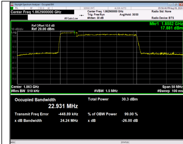
2-2-5MHz-20MHz-QPSK-QPSK-18633-18750-25RB#0-10 ORB#0-PASS
