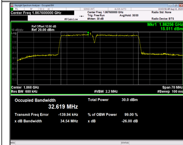
2-2-15MHz-20MHz-16QAM-16QAM-18678-18849-75RB#0-1 -100RB#0-PASS
