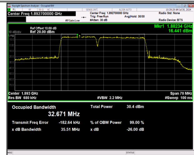
2-2-15MHz-20MHz-64QAM-64QAM-18929-19100-75RB#0 -100RB#0-PASS
