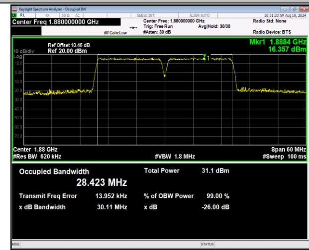
2-2-15MHz-15MHz-QPSK-QPSK-18825-18975-75RB#0-7 5RB#0-PASS
