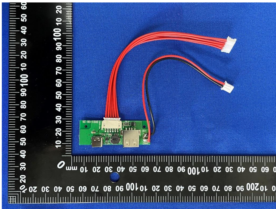
SMWDA POWER BOARD TOP VIEW
