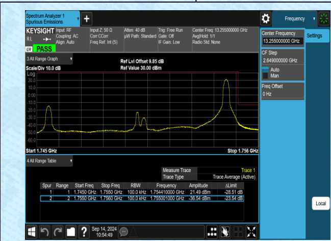
Band4-10MHz-16QAM-20350-1RB#49-PASS
