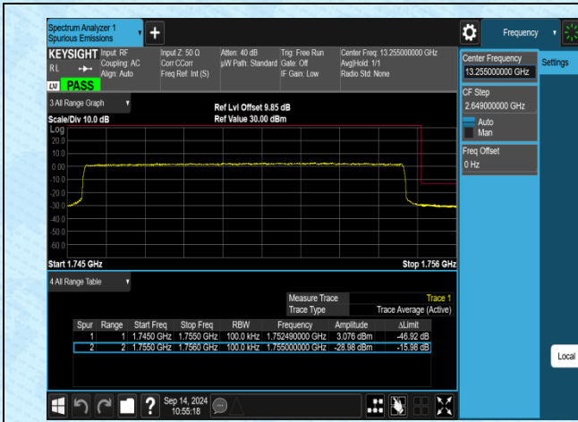
Band4-10MHz-16QAM-20350-50RB#0-PASS
