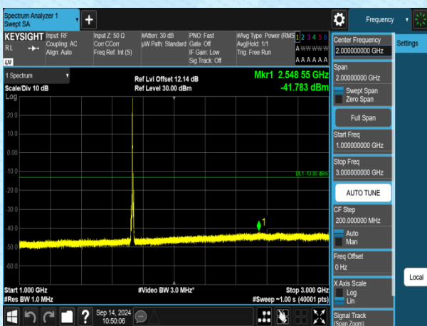
Band4-5MHz-QPSK-20175-1RB#0-1000~3000-PASS
