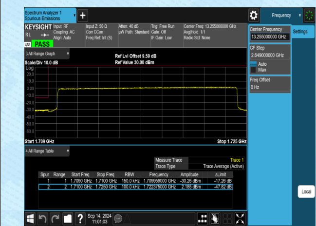
Band4-15MHz-QPSK-20025-75RB#0-PASS
