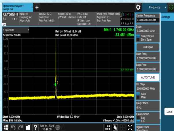
Band4-3MHz-QPSK-20385-1RB#0-1000~3000-PASS
