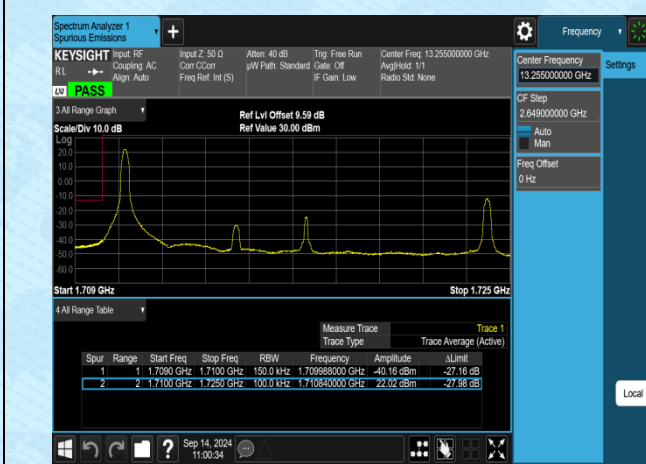
Band4-15MHz-QPSK-20025-1RB#0-PASS
