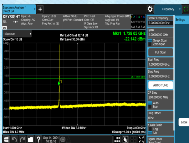
Band4-1.4MHz-QPSK-20175-1RB#0-1000~3000-PASS
