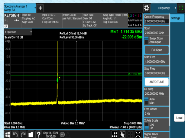
Band4-1.4MHz-QPSK-19957-1RB#0-1000~3000-PASS
