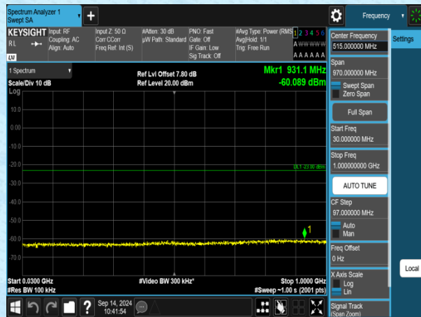
Band4-3MHz-QPSK-19965-1RB#0-30~1000-PASS
