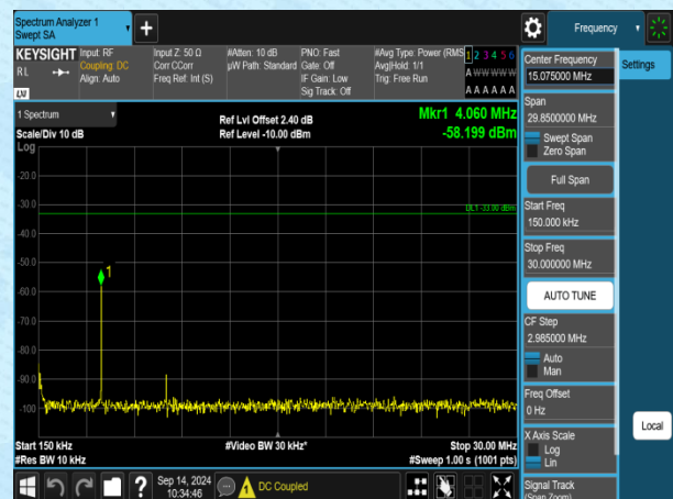
Band4-1.4MHz-QPSK-19957-1RB#0-0.15~30-PASS
