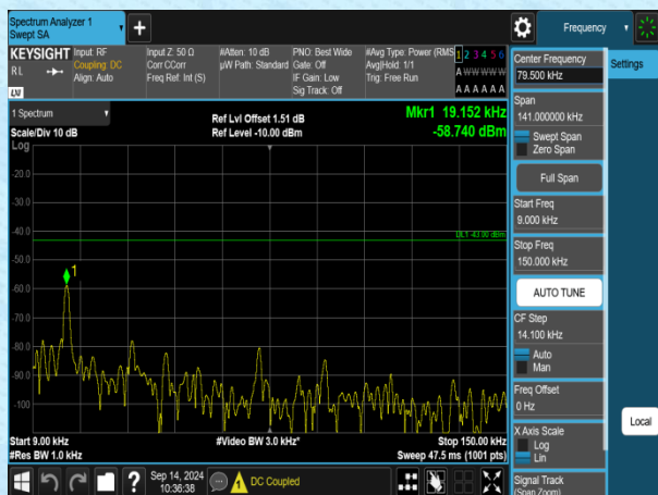
Band4-1.4MHz-QPSK-20393-1RB#0-0.009~0.15-PASS
