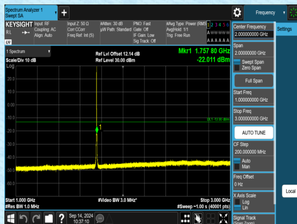
Band4-1.4MHz-QPSK-20393-1RB#0-1000~3000-PASS
