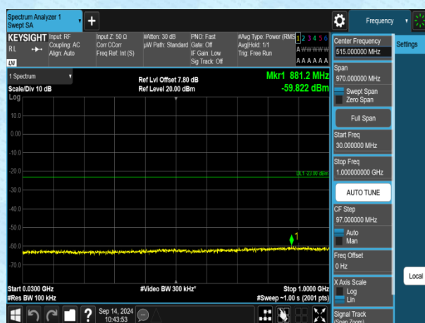
Band4-3MHz-QPSK-20385-1RB#0-30~1000-PASS
