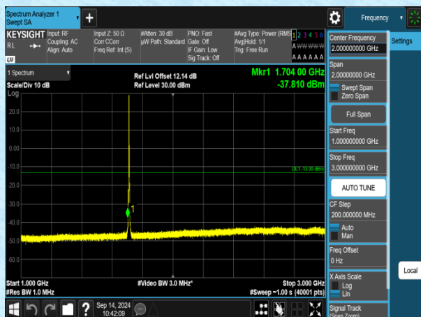
Band4-3MHz-QPSK-19965-1RB#0-1000~3000-PASS
