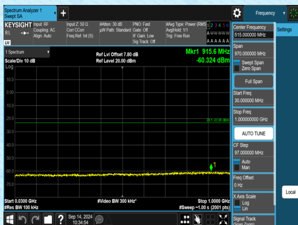
Band4-1.4MHz-QPSK-19957-1RB#0-30~1000-PASS
