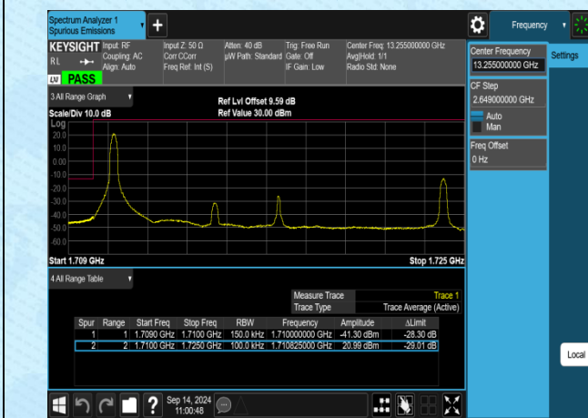
Band4-15MHz-16QAM-20025-1RB#0-PASS
