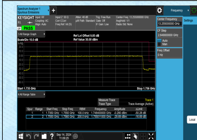
Band4-20MHz-16QAM-20300-100RB#0-PASS
