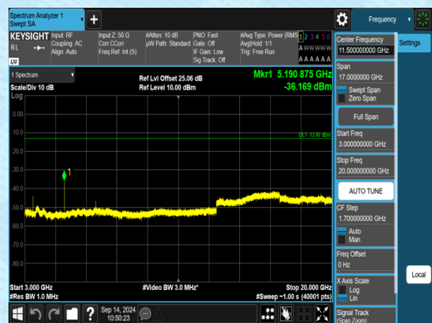
Band4-5MHz-QPSK-20175-1RB#0-3000~20000-PASS
