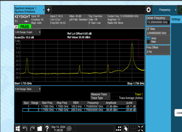
Band4-20MHz-16QAM-20300-1RB#99-PASS
