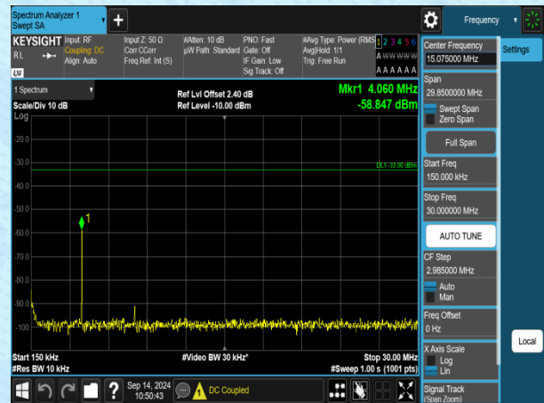
Band4-5MHz-QPSK-20375-1RB#0-0.15~30-PASS
