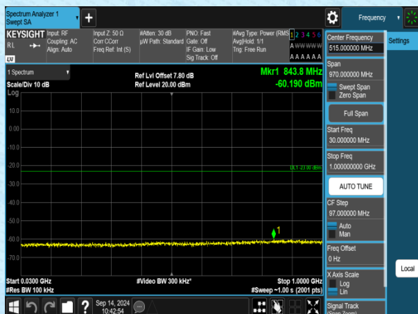
Band4-3MHz-QPSK-20175-1RB#0-30~1000-PASS
