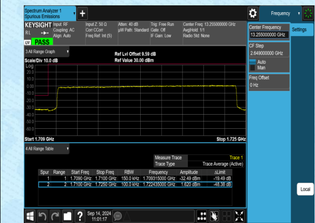
Band4-15MHz-16QAM-20025-75RB#0-PASS
