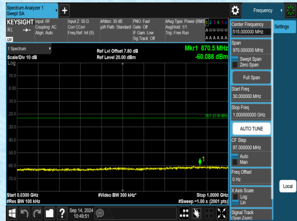
Band4-5MHz-QPSK-20175-1RB#0-30~1000-PASS
