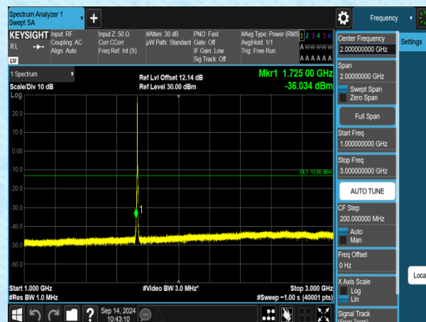
Band4-3MHz-QPSK-20175-1RB#0-1000~3000-PASS
