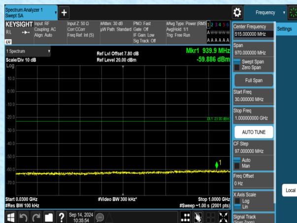
Band4-1.4MHz-QPSK-20175-1RB#0-30~1000-PASS
