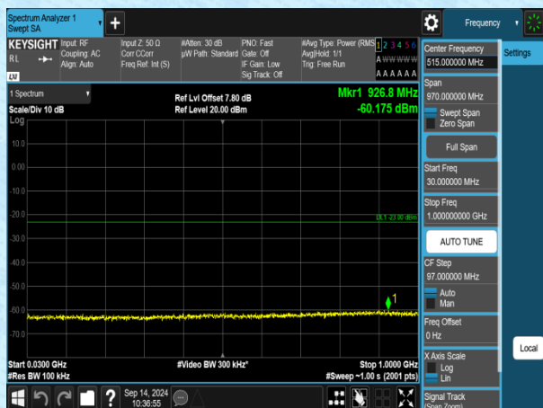
Band4-1.4MHz-QPSK-20393-1RB#0-30~1000-PASS
