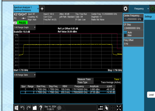
Band4-20MHz-QPSK-20300-100RB#0-PASS
