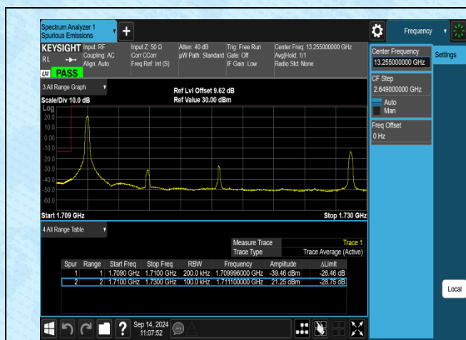
Band4-20MHz-16QAM-20050-1RB#0-PASS
