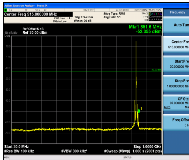
Band5_5MHz_QPSK_20525_1RB#0_30~1000_30~1000
