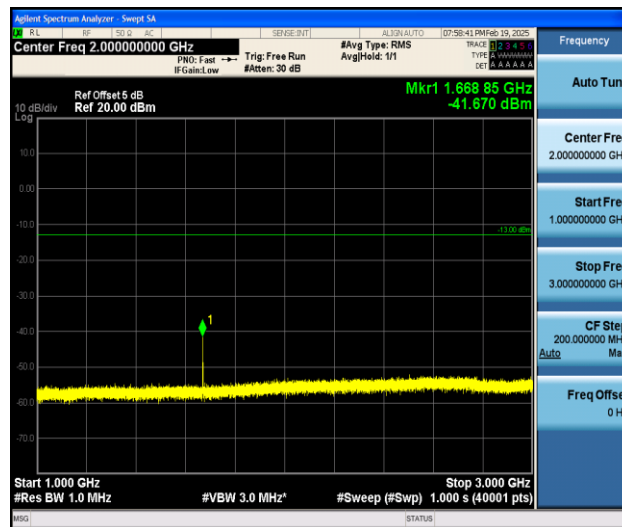
Band5_5MHz_16QAM_20525_1RB#0_1000~3000_1000~3000
