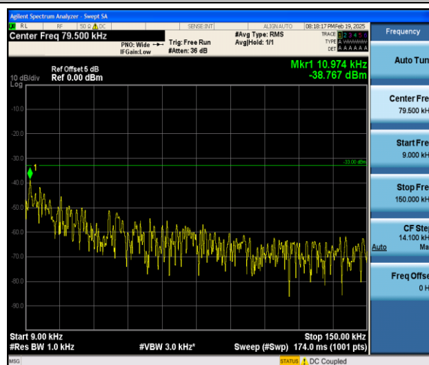
Band5_10MHz_16QAM_20450_1RB#0_0.009~0.15_0.009~0.15
