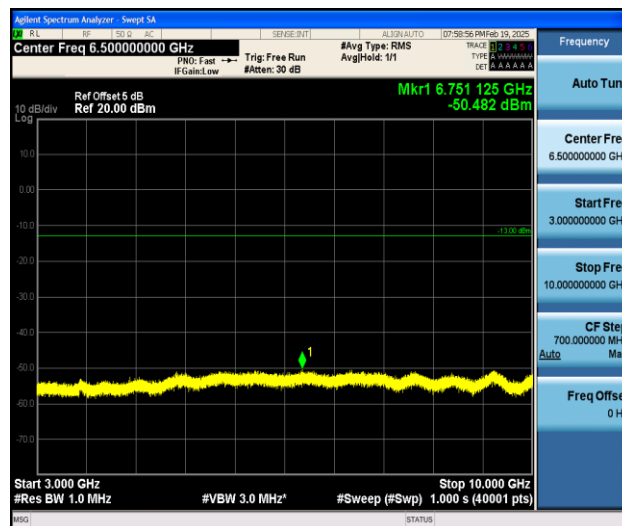
Band5_5MHz_16QAM_20525_1RB#0_3000~10000_3000~10000
