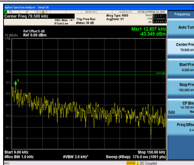
Band5_5MHz_16QAM_20425_1RB#0_0.009~0.15_0.009~0.15
