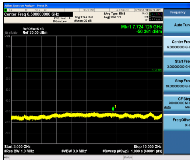
Band5_5MHz_QPSK_20625_1RB#0_3000~10000_3000~10000
