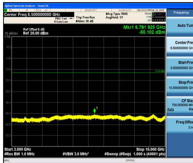
Band5_10MHz_16QAM_20450_1RB#0_3000~10000_3000~10000
