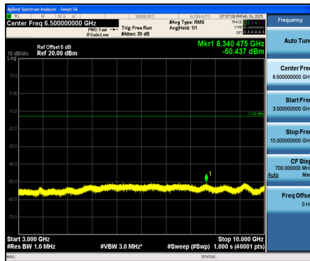
Band5_5MHz_16QAM_20425_1RB#0_3000~10000_3000~10000
