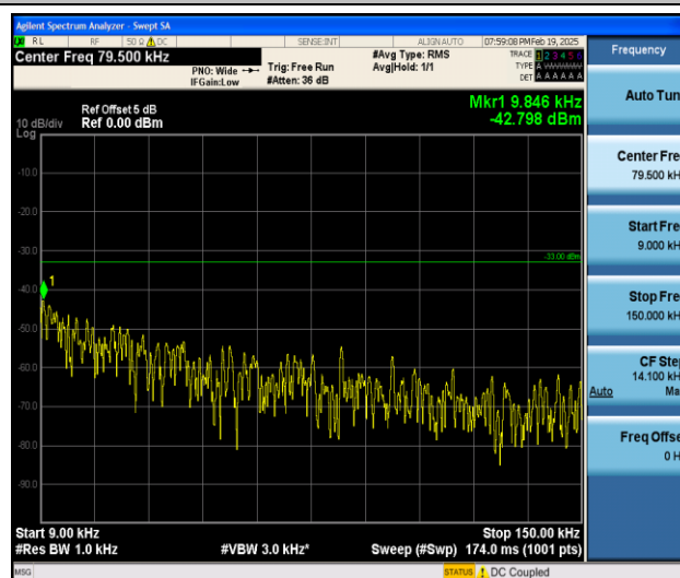
Band5_5MHz_QPSK_20625_1RB#0_0.009~0.15_0.009~0.15
