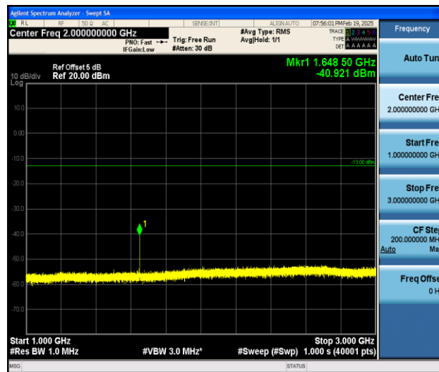
Band5_5MHz_QPSK_20425_1RB#0_1000~3000_1000~3000
