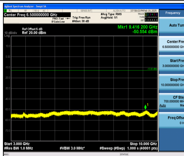
Band5_5MHz_QPSK_20525_1RB#0_3000~10000_3000~10000
