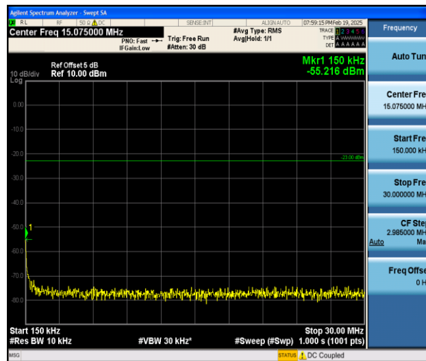
Band5_5MHz_QPSK_20625_1RB#0_0.15~30_0.15~30
