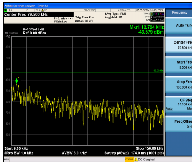
Band5_5MHz_QPSK_20425_1RB#0_0.009~0.15_0.009~0.15
