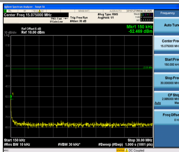
Band5_5MHz_QPSK_20525_1RB#0_0.15~30_0.15~30
