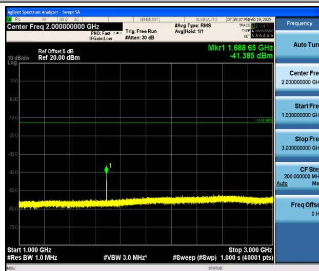
Band5_5MHz_QPSK_20625_1RB#0_1000~3000_1000~3000
