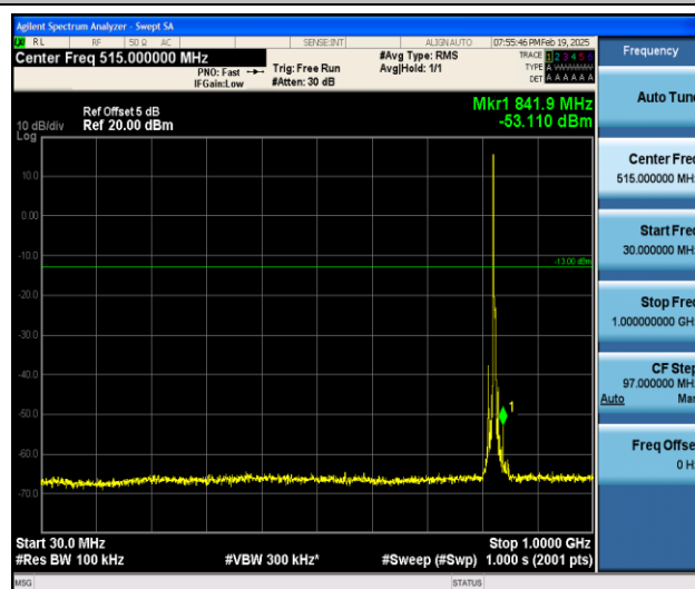
Band5_5MHz_QPSK_20425_1RB#0_30~1000_30~1000
