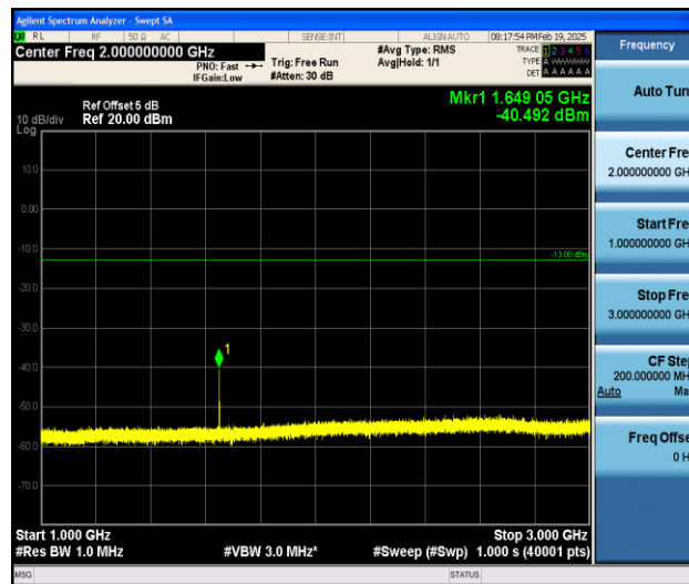
Band5_10MHz_QPSK_20450_1RB#0_1000~3000_1000~3000
