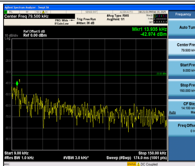
Band5_10MHz_QPSK_20600_1RB#0_0.009~0.15_0.009~0.15
