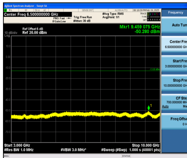
Band5_10MHz_QPSK_20450_1RB#0_3000~10000_3000~10000
