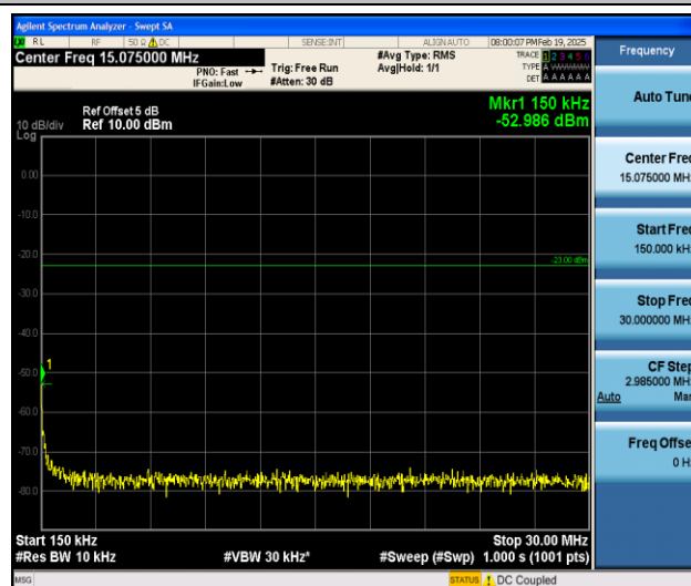
Band5_5MHz_16QAM_20625_1RB#0_0.15~30_0.15~30
