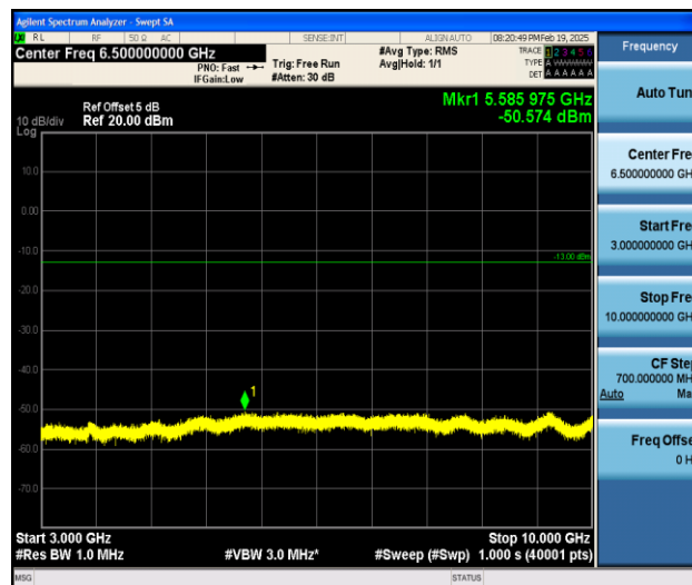
Band5_10MHz_16QAM_20525_1RB#0_3000~10000_3000~10000
