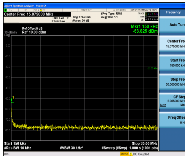
Band5_5MHz_QPSK_20425_1RB#0_0.15~30_0.15~30
