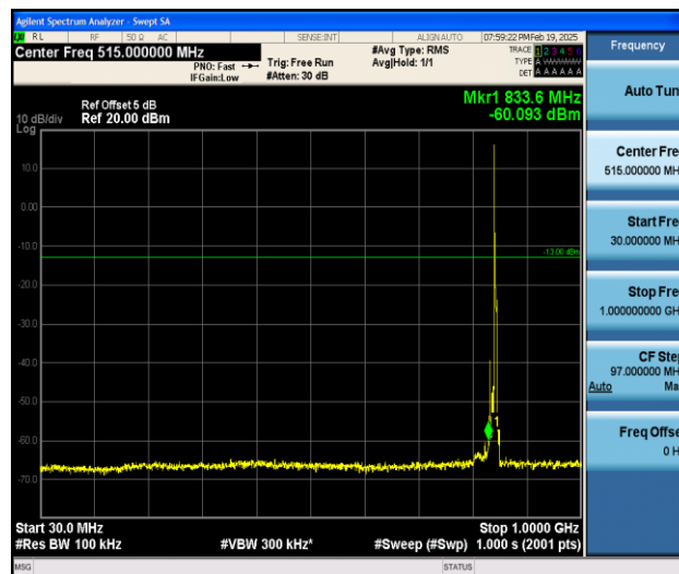
Band5_5MHz_QPSK_20625_1RB#0_30~1000_30~1000
