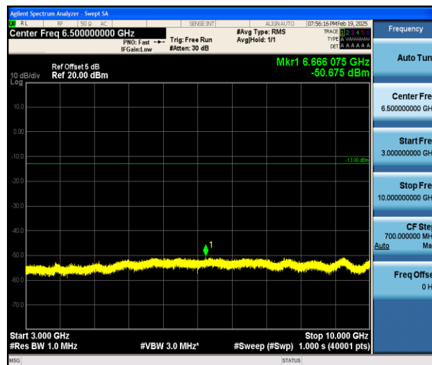
Band5_5MHz_QPSK_20425_1RB#0_3000~10000_3000~10000
