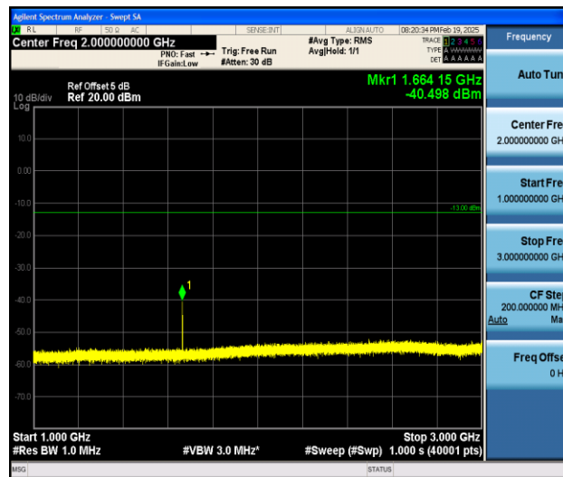
Band5_10MHz_16QAM_20525_1RB#0_1000~3000_1000~3000
