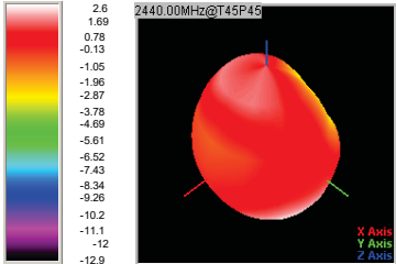
◎ 3D Gain Pattern (2440 MHz)
