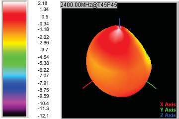
◎ 3D Gain Pattern (2400 MHz)
