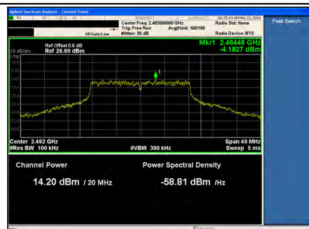
11g-PSD-High-54Mbps
