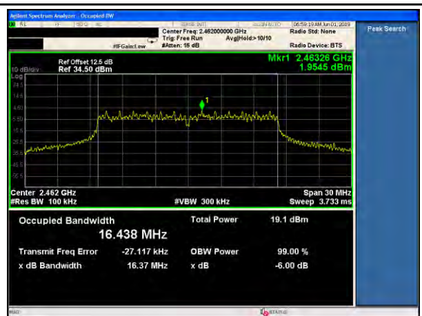
11g-6dB BW-High-54Mbps
