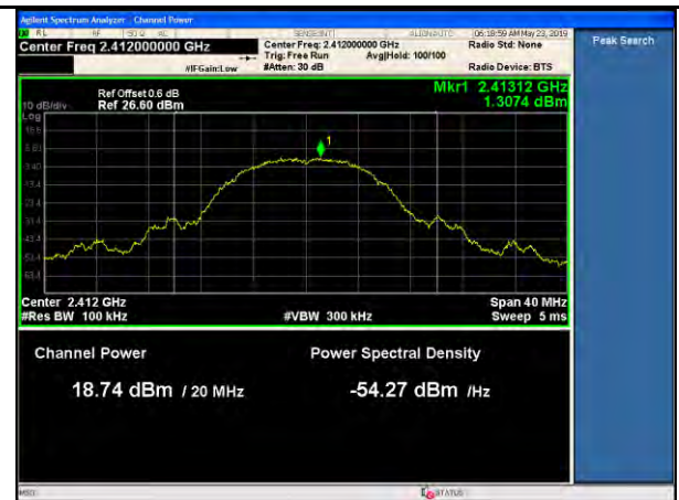
11b-PSD-Low-11Mbps
