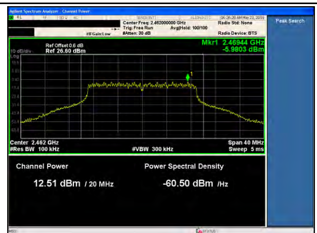
11n-20MHz-PSD-High-MCS7
