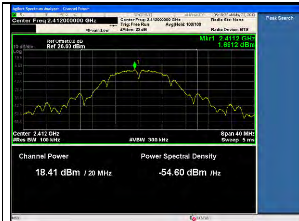
11b-PSD-Low-1Mbps
