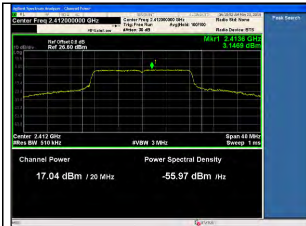
11g-PWR-Low-6Mbps
