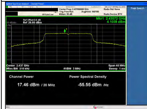
11g-PWR-Mid-6Mbps
