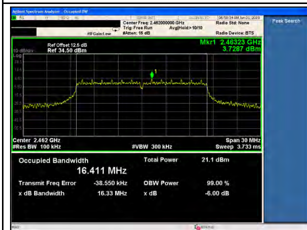
11g-6dB BW-High-6Mbps
