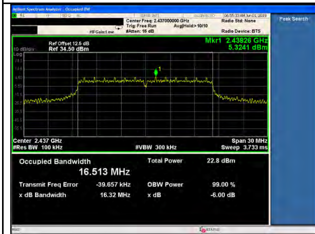
11g-6dB BW-Mid-6Mbps
