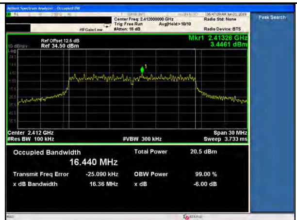
11g-6dB BW-Low-54Mbps
