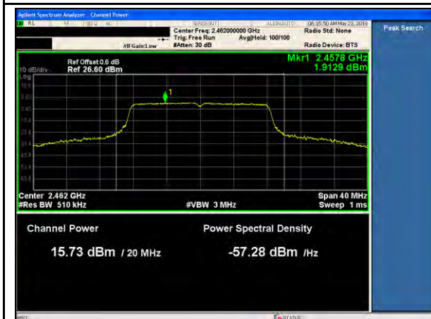
11g-PWR-High-6Mbps
