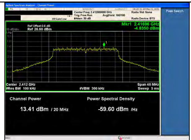
11n-20MHz-PSD-Low-MCS7
