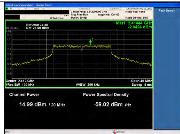
11g-PSD-Low-54Mbps
