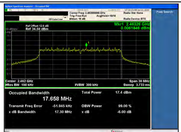
11n-20MHz-6dB BW-High-MCS7
