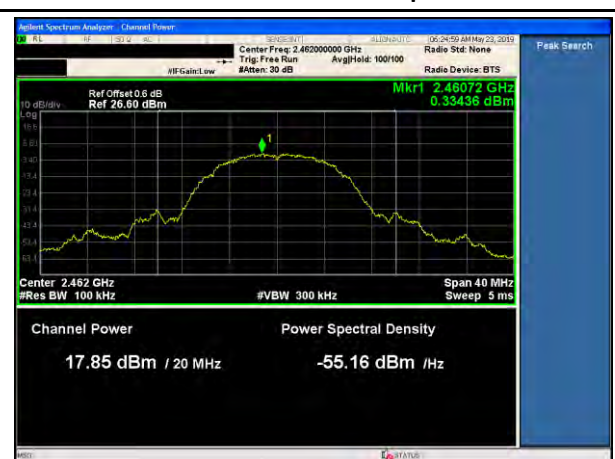
11b-PSD-High-11Mbps
