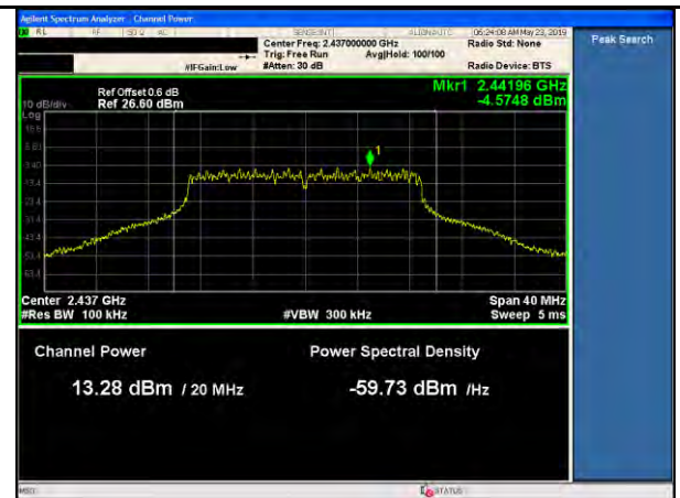
11n-20MHz-PSD-Mid-MCS7
