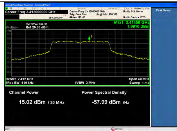
11g-PWR-Low-54Mbps
