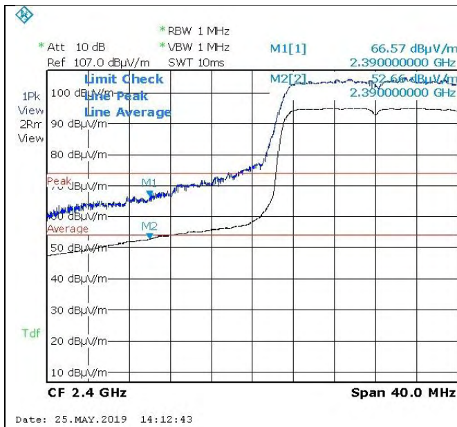
802.11n 2412M-Low
