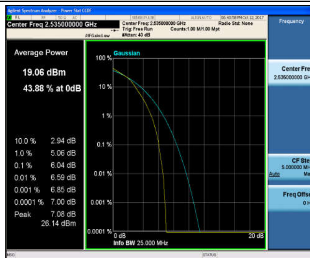
Band7_15MHz_QPSK_21375_1RB#0_5.25_13_PASS
