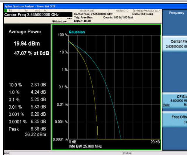
Band7_20MHz_16QAM_21100_100RB#0_6.07_13_PASS
