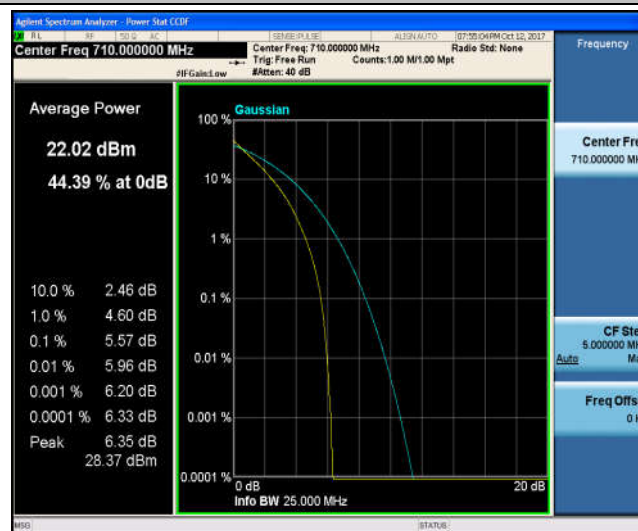
Band17_10MHz_16QAM_23790_50RB#0_6.42_13_PASS
