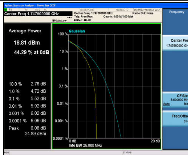
Band4_15MHz_16QAM_20325_1RB#0_6.41_13_PASS
