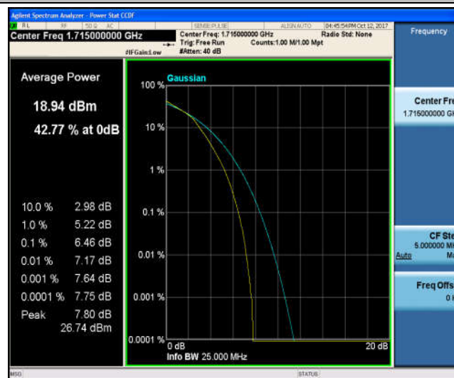
Band4_10MHz_QPSK_20175_1RB#0_5.04_13_PASS
