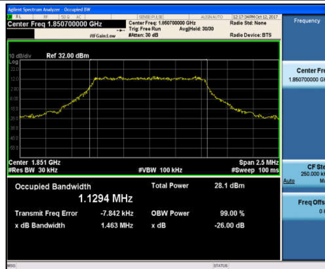
Band2_1.4MHz_QPSK_18900_6RB#0_1.1053_1.422_PASS
