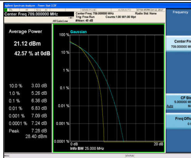
Band17_10MHz_QPSK_23790_1RB#0_5.16_13_PASS
