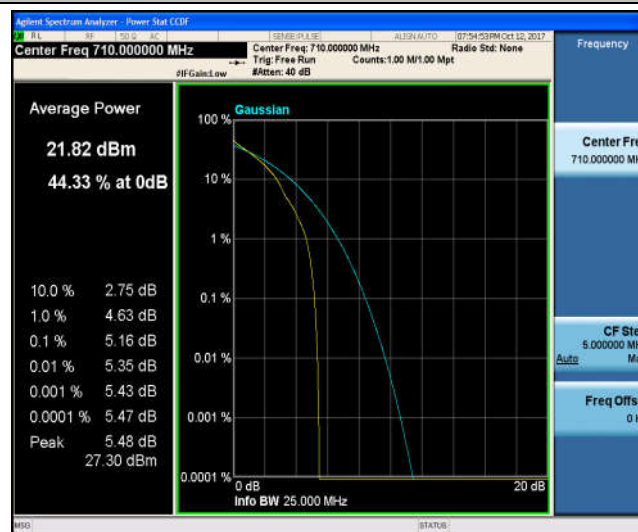
Band17_10MHz_16QAM_23790_1RB#0_5.21_13_PASS
