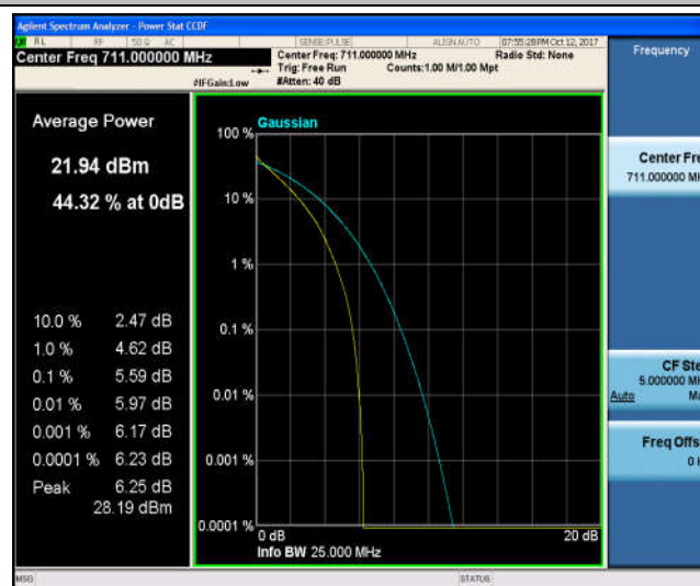
Band17_10MHz_16QAM_23800_50RB#0_6.46_13_PASS
