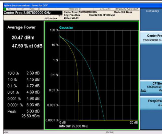
Band7_5MHz_16QAM_21425_25RB#0_5.62_13_PASS
