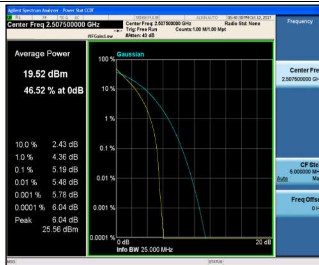
Band7_15MHz_16QAM_20825_75RB#0_5.89_13_PASS
