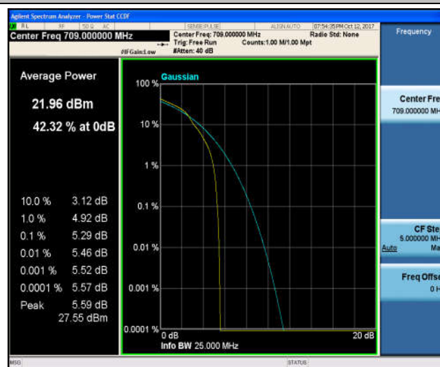
Band17_10MHz_QPSK_23780_50RB#0_5.50_13_PASS
