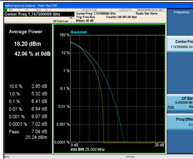
Band4_15MHz_QPSK_20325_75RB#0_5.78_13_PASS
