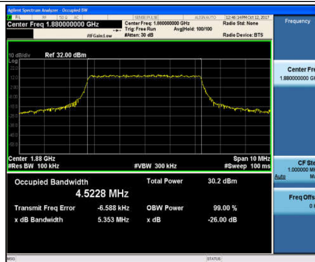
Band2_5MHz_16QAM_18900_25RB#0_4.5309_5.423_PASS
