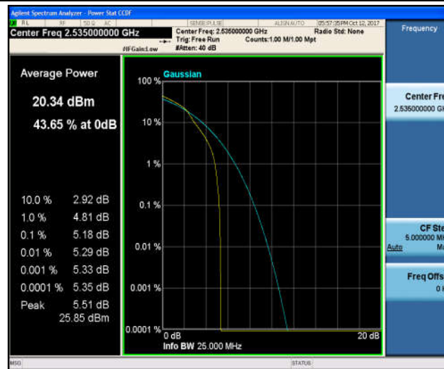
Band7_5MHz_QPSK_21100_25RB#0_4.94_13_PASS
