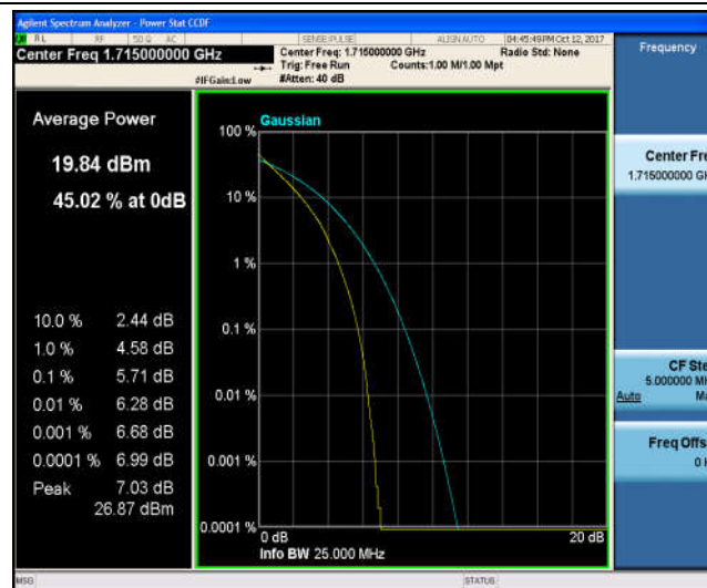
Band4_10MHz_16QAM_20000_50RB#0_6.46_13_PASS
