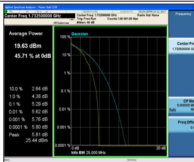
Band4_15MHz_16QAM_20175_1RB#0_6.13_13_PASS
