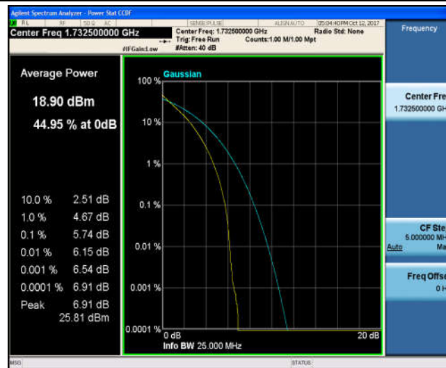
Band4_15MHz_16QAM_20175_75RB#0_6.33_13_PASS
