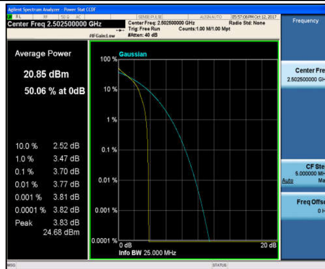
Band7_5MHz_16QAM_20775_1RB#0_4.11_13_PASS
