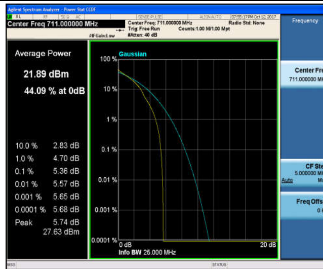
Band17_10MHz_16QAM_23800_1RB#0_5.47_13_PASS
