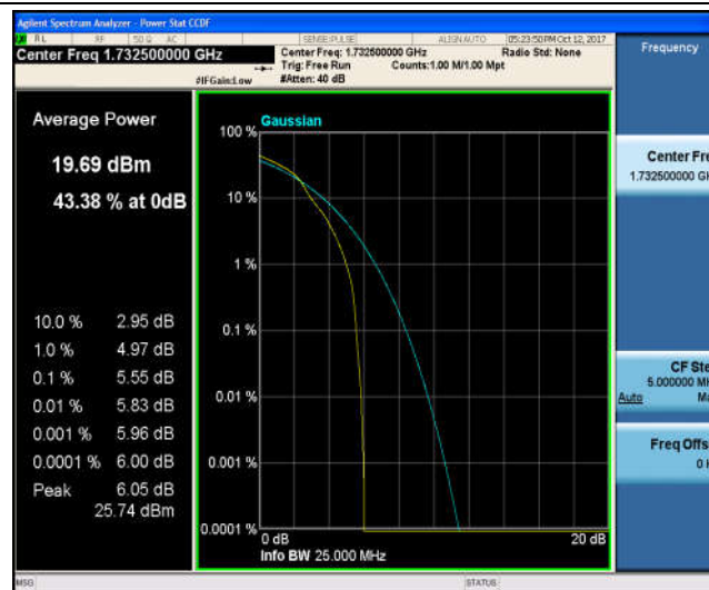
Band4_20MHz_QPSK_20175_100RB#0_5.49_13_PASS
