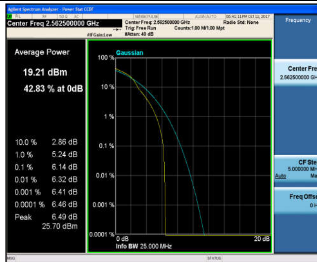
Band7_15MHz_QPSK_21375_75RB#0_5.46_13_PASS
