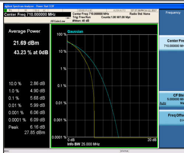
Band17_5MHz_16QAM_23790_1RB#0_5.46_13_PASS
