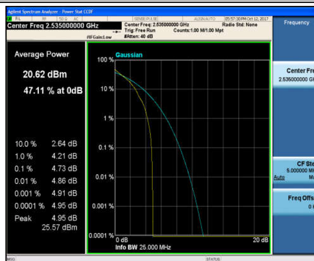
Band7_5MHz_16QAM_21100_1RB#0_5.18_13_PASS
