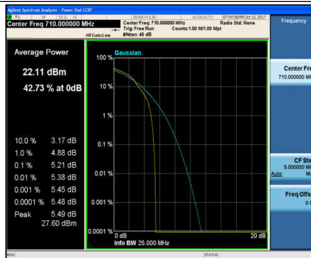
Band17_10MHz_QPSK_23790_50RB#0_5.57_13_PASS
