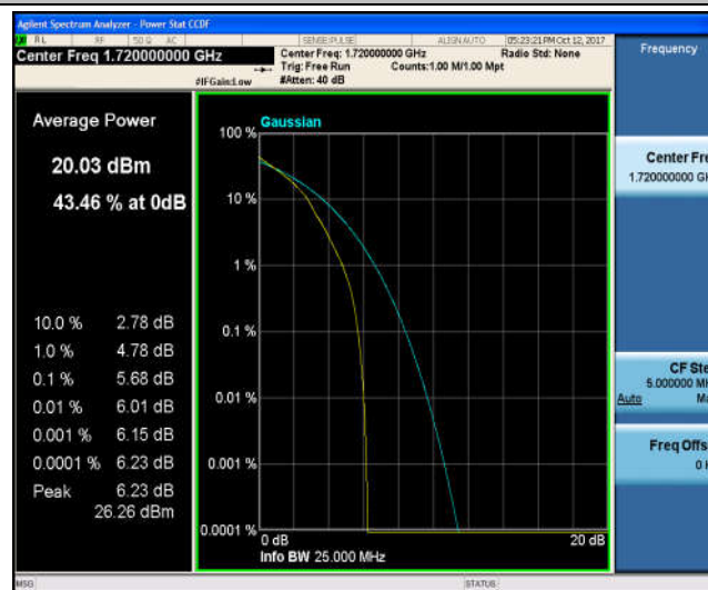
Band4_20MHz_16QAM_20050_1RB#0_6.05_13_PASS
