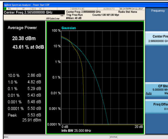
Band7_10MHz_QPSK_21400_50RB#0_4.90_13_PASS
