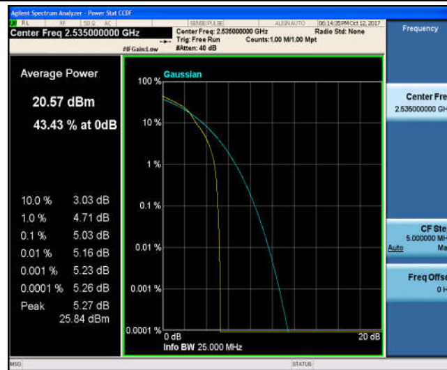
Band7_10MHz_QPSK_21100_50RB#0_4.99_13_PASS
