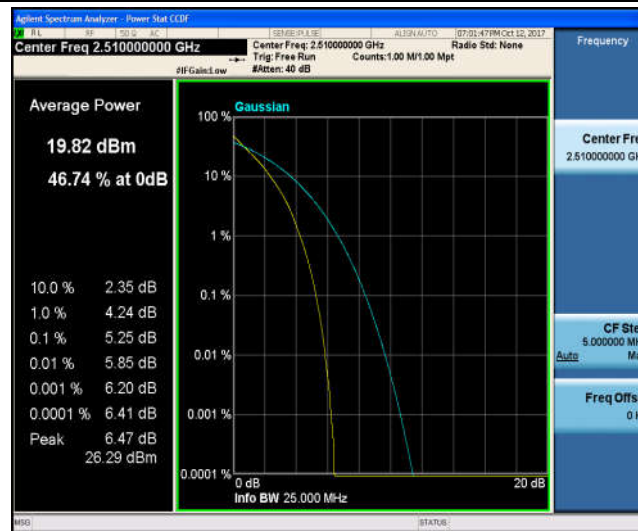
Band7_20MHz_16QAM_20850_100RB#0_5.96_13_PASS
