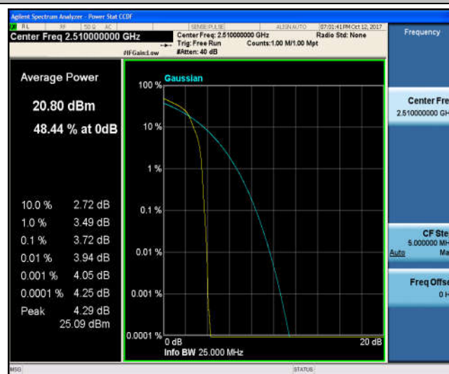
Band7_20MHz_QPSK_20850_100RB#0_5.25_13_PASS
