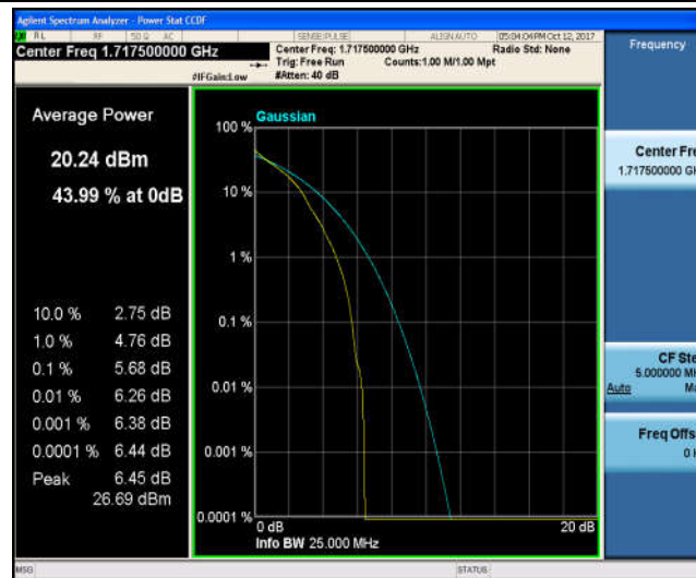
Band4_15MHz_16QAM_20025_1RB#0_6.64_13_PASS
