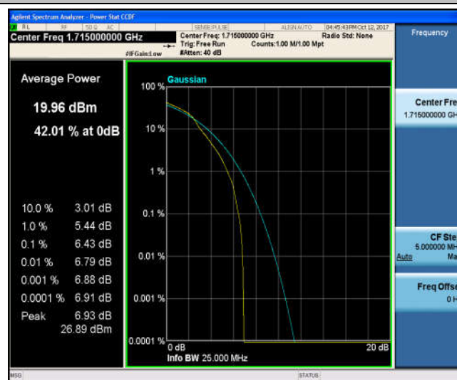
Band4_10MHz_QPSK_20000_50RB#0_5.71_13_PASS
