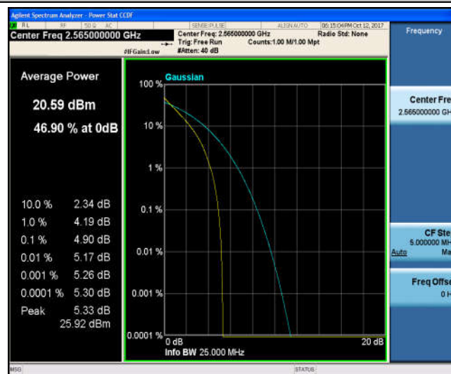
Band7_10MHz_16QAM_21400_50RB#0_5.79_13_PASS
