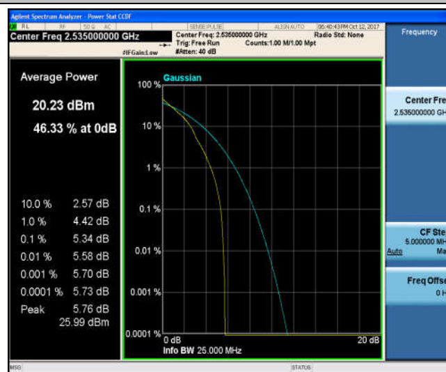
Band7_15MHz_16QAM_21100_1RB#0_5.91_13_PASS
