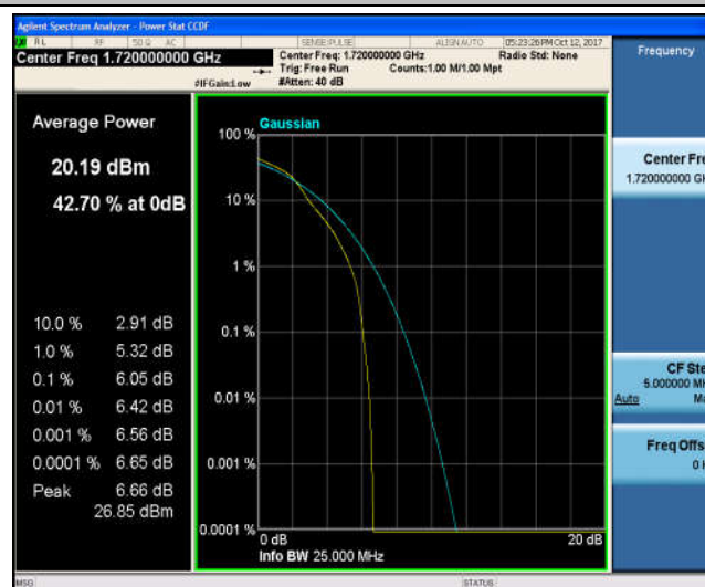
Band4_20MHz_QPSK_20050_100RB#0_5.63_13_PASS
