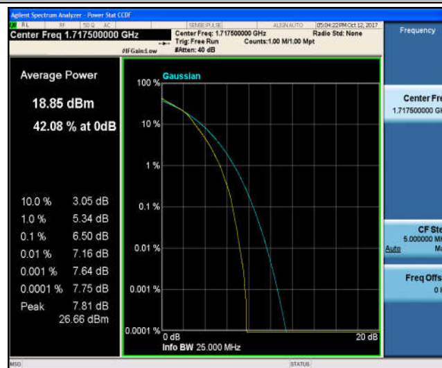
Band4_15MHz_QPSK_20175_1RB#0_5.29_13_PASS
