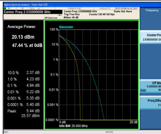
Band7_5MHz_16QAM_21100_25RB#0_5.82_13_PASS
