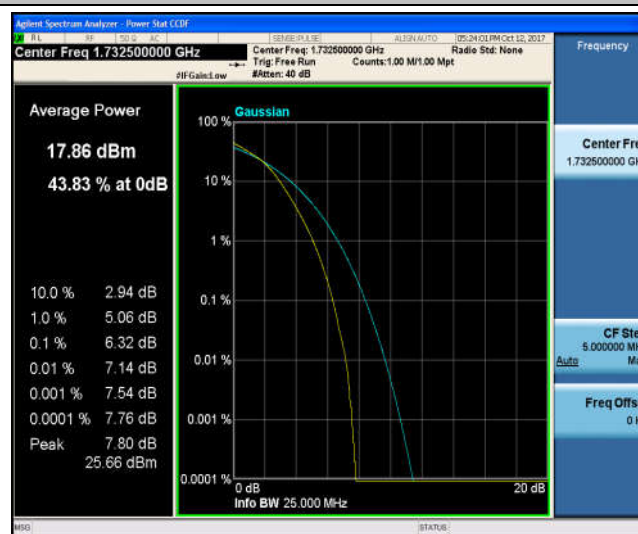
Band4_20MHz_QPSK_20300_1RB#0_5.49_13_PASS
