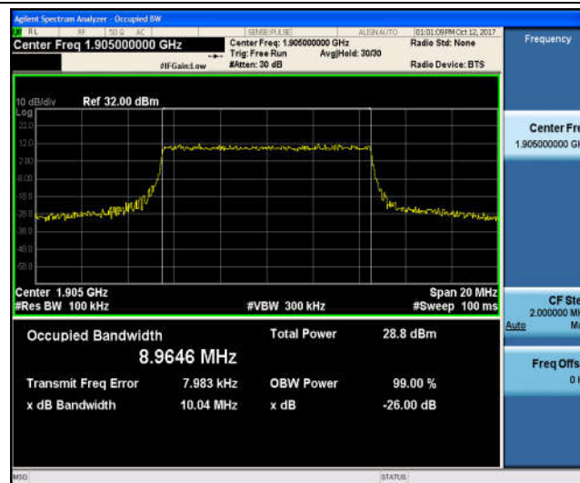
Band2_15MHz_QPSK_18675_75RB#0_13.512_15.10_PASS
