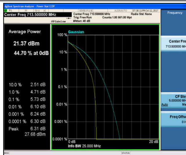
Band17_5MHz_16QAM_23825_25RB#0_6.52_13_PASS
