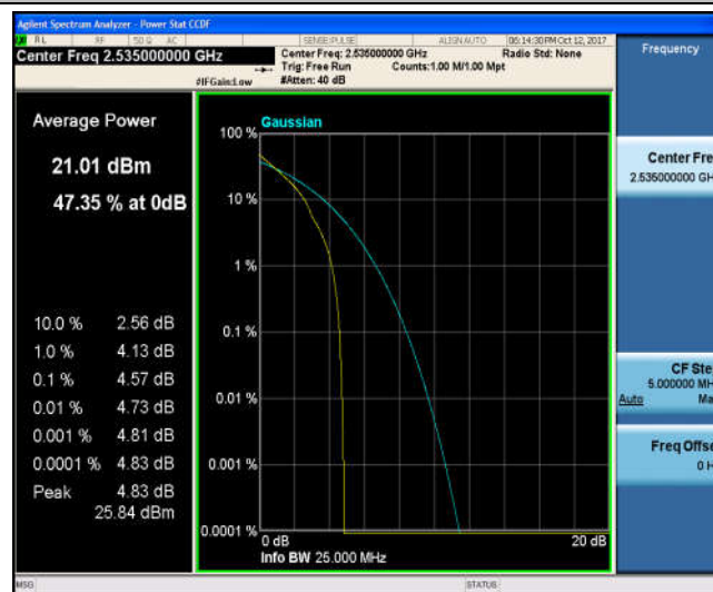
Band7_10MHz_16QAM_21100_1RB#0_5.03_13_PASS
