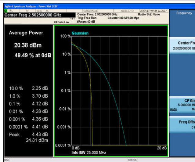
Band7_5MHz_16QAM_20775_25RB#0_5.00_13_PASS
