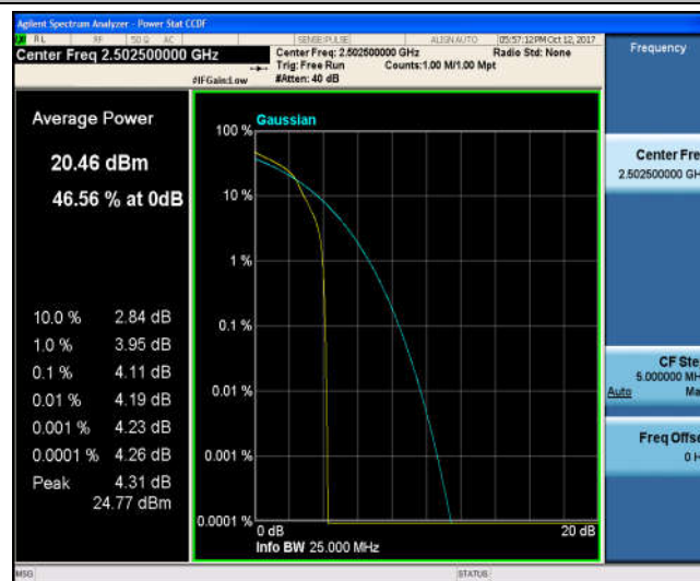
Band7_5MHz_QPSK_20775_25RB#0_4.12_13_PASS
