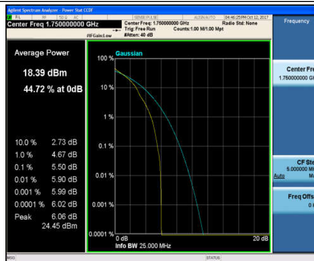
Band4_10MHz_16QAM_20350_1RB#0_6.27_13_PASS
