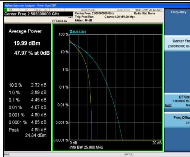
Band7_10MHz_16QAM_20800_50RB#0_5.46_13_PASS
