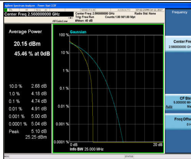
Band7_20MHz_16QAM_21350_1RB#0_5.12_13_PASS
