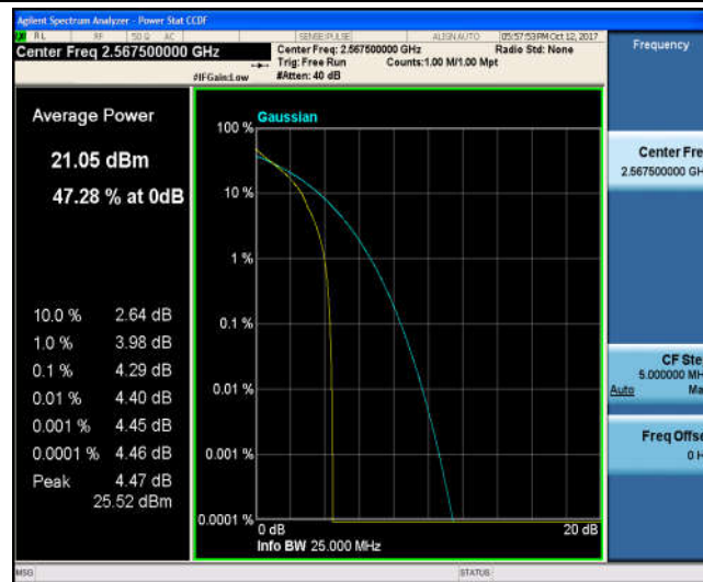
Band7_5MHz_16QAM_21425_1RB#0_4.75_13_PASS
