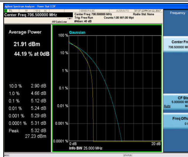
Band17_5MHz_16QAM_23755_1RB#0_5.42_13_PASS
