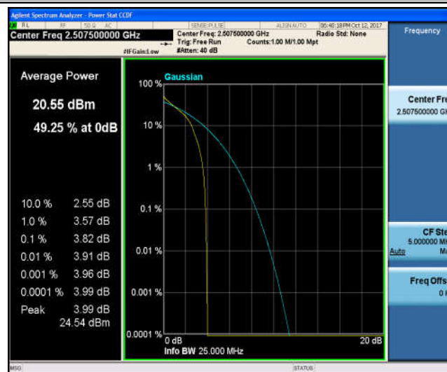
Band7_15MHz_16QAM_20825_1RB#0_4.35_13_PASS
