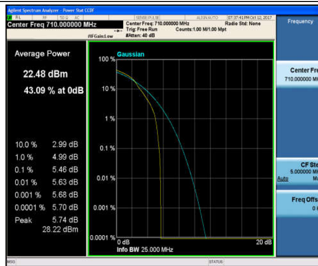
Band17_5MHz_QPSK_23790_25RB#0_5.81_13_PASS
