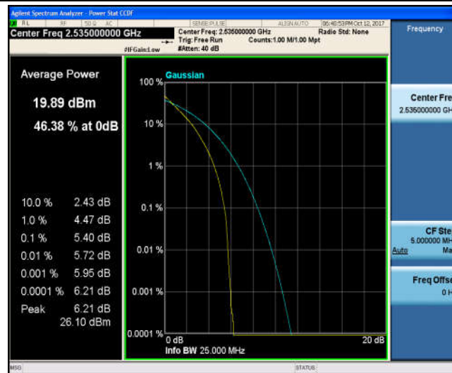
Band7_15MHz_16QAM_21100_75RB#0_6.04_13_PASS
