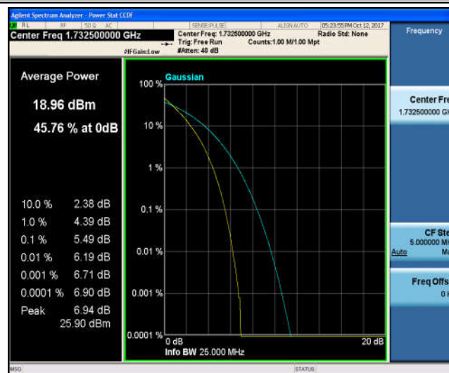
Band4_20MHz_16QAM_20175_100RB#0_6.32_13_PASS
