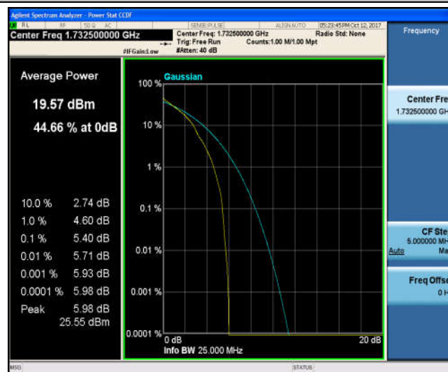
Band4_20MHz_16QAM_20175_1RB#0_5.55_13_PASS
