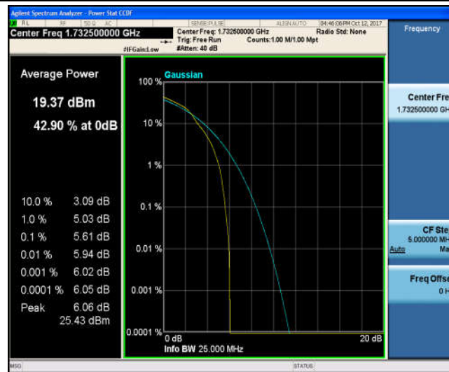
Band4_10MHz_QPSK_20175_50RB#0_5.41_13_PASS
