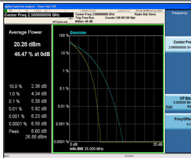
Band7_20MHz_16QAM_21350_100RB#0_6.12_13_PASS
