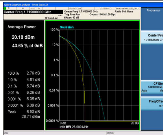
Band4_10MHz_16QAM_20000_1RB#0_6.43_13_PASS
