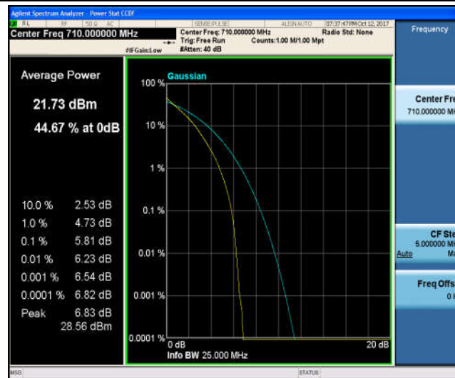
Band17_5MHz_16QAM_23790_25RB#0_6.64_13_PASS
