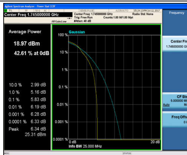
Band4_20MHz_QPSK_20300_100RB#0_5.50_13_PASS
