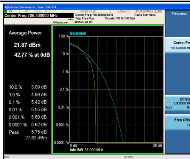
Band17_5MHz_QPSK_23755_25RB#0_5.46_13_PASS
