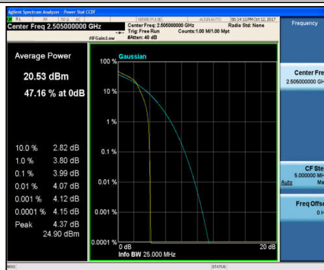
Band7_10MHz_QPSK_20800_50RB#0_4.45_13_PASS
