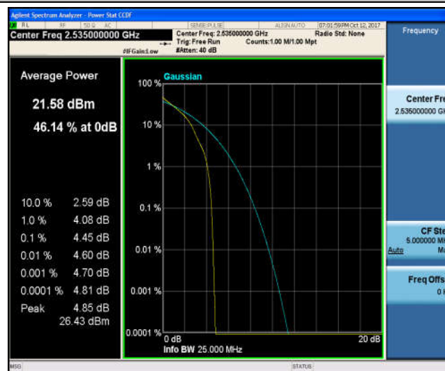
Band7_20MHz_16QAM_21100_1RB#0_4.93_13_PASS
