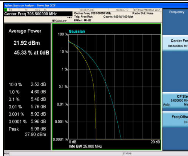
Band17_5MHz_16QAM_23755_25RB#0_6.29_13_PASS
