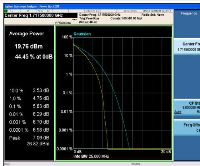
Band4_15MHz_16QAM_20025_75RB#0_6.50_13_PASS
