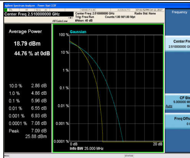
Band7_20MHz_QPSK_21100_1RB#0_4.45_13_PASS
