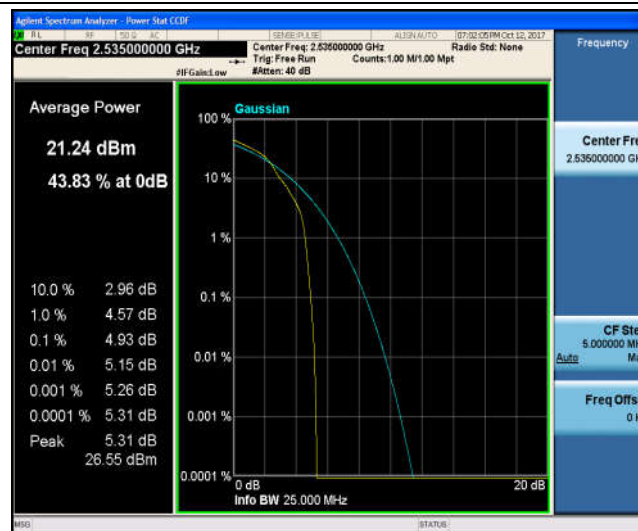
Band7_20MHz_QPSK_21100_100RB#0_5.25_13_PASS
