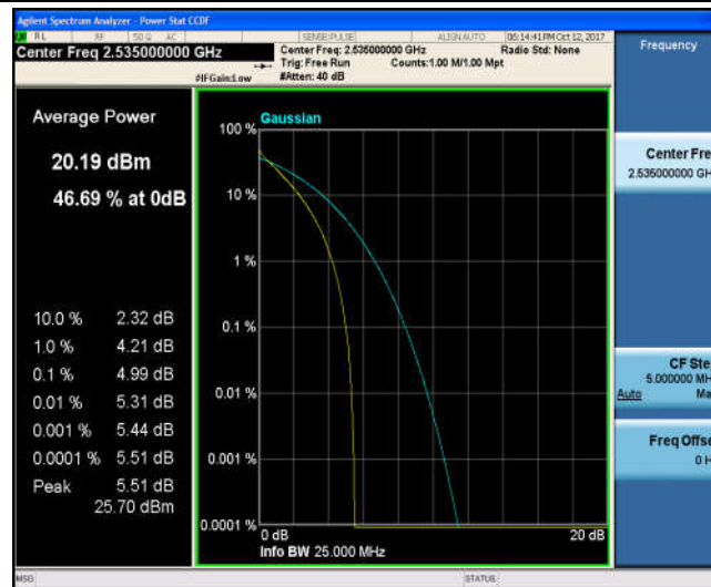
Band7_10MHz_16QAM_21100_50RB#0_5.81_13_PASS
