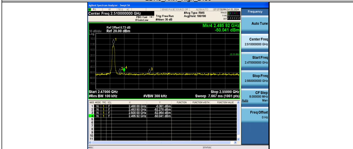
2DH5 Ant2_High_2480
