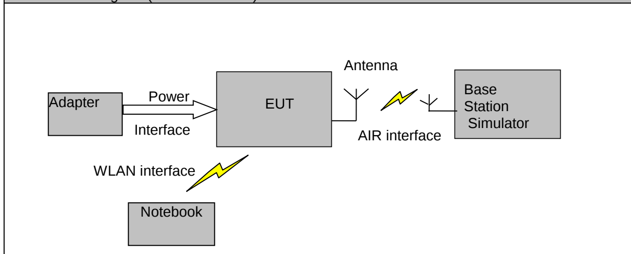
Connection Diagram (Mode 1-Mode 2)
