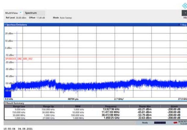
NB-IoT Band 25 CH-Middle 9kHz~27GHz
