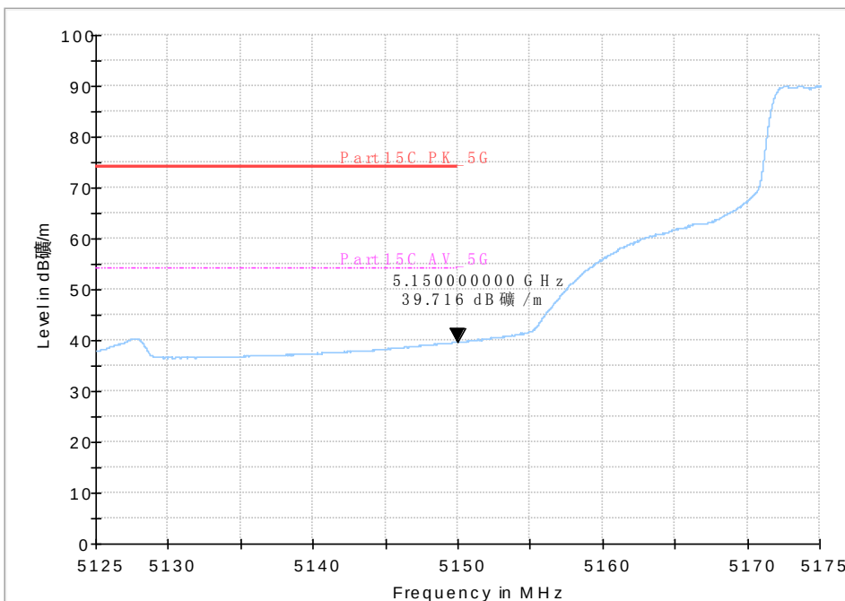
Fig. 37 Band Edges (802.11a, 5180MHz)
