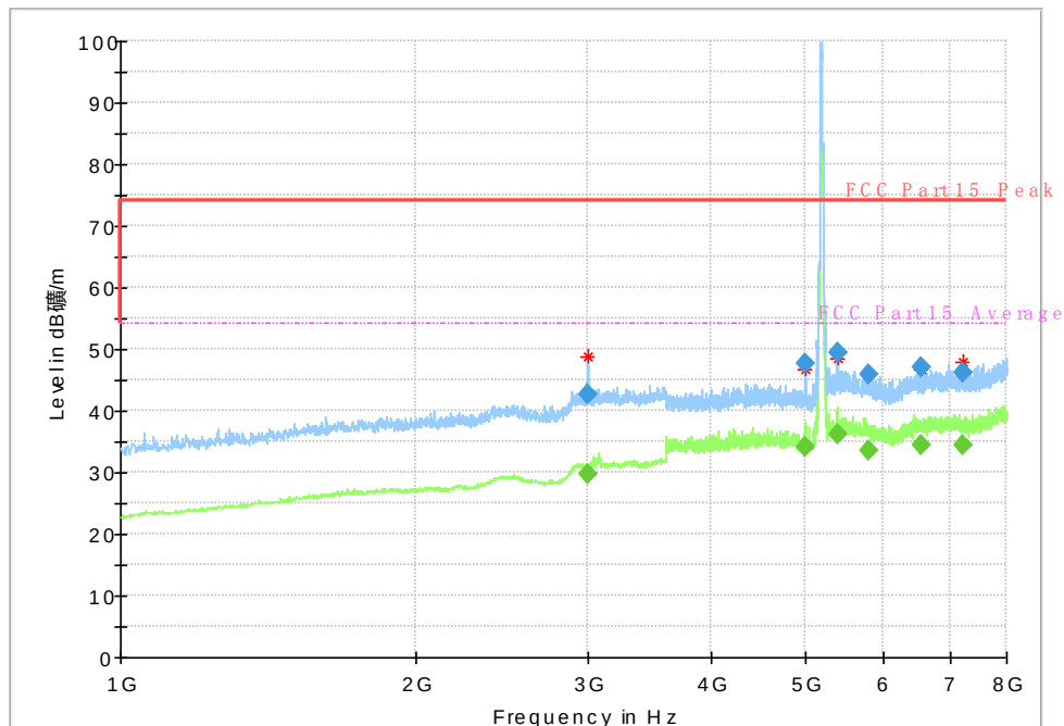
Fig. 63 Radiated Spurious Emission (802.11a, ch36, 1 GHz-8 GHz)
