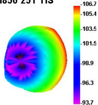
GSM850 251 TIS
