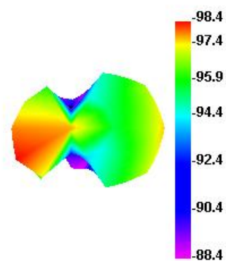
LTE2 1150 TIS
