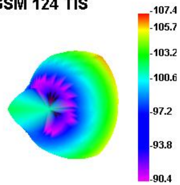
EGSM 124 TIS
