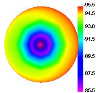
LTE12 5130 TIS
