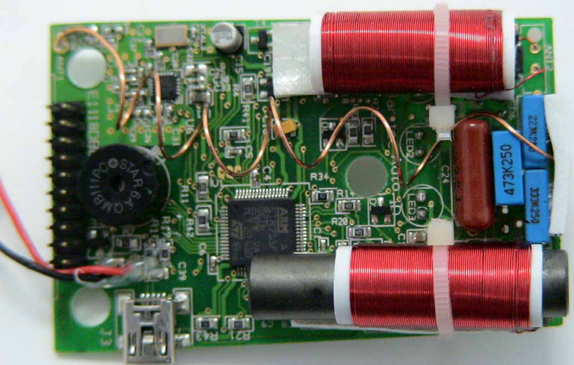
PCB (bottom)
