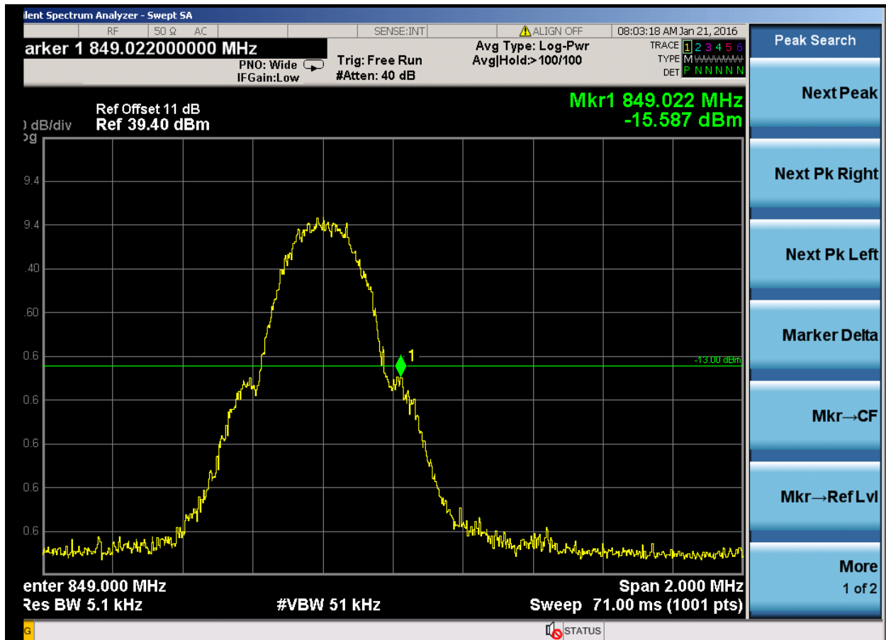
(Plot 4.4.1 B: Channel 251: 848.80MHz @ GSM850)
