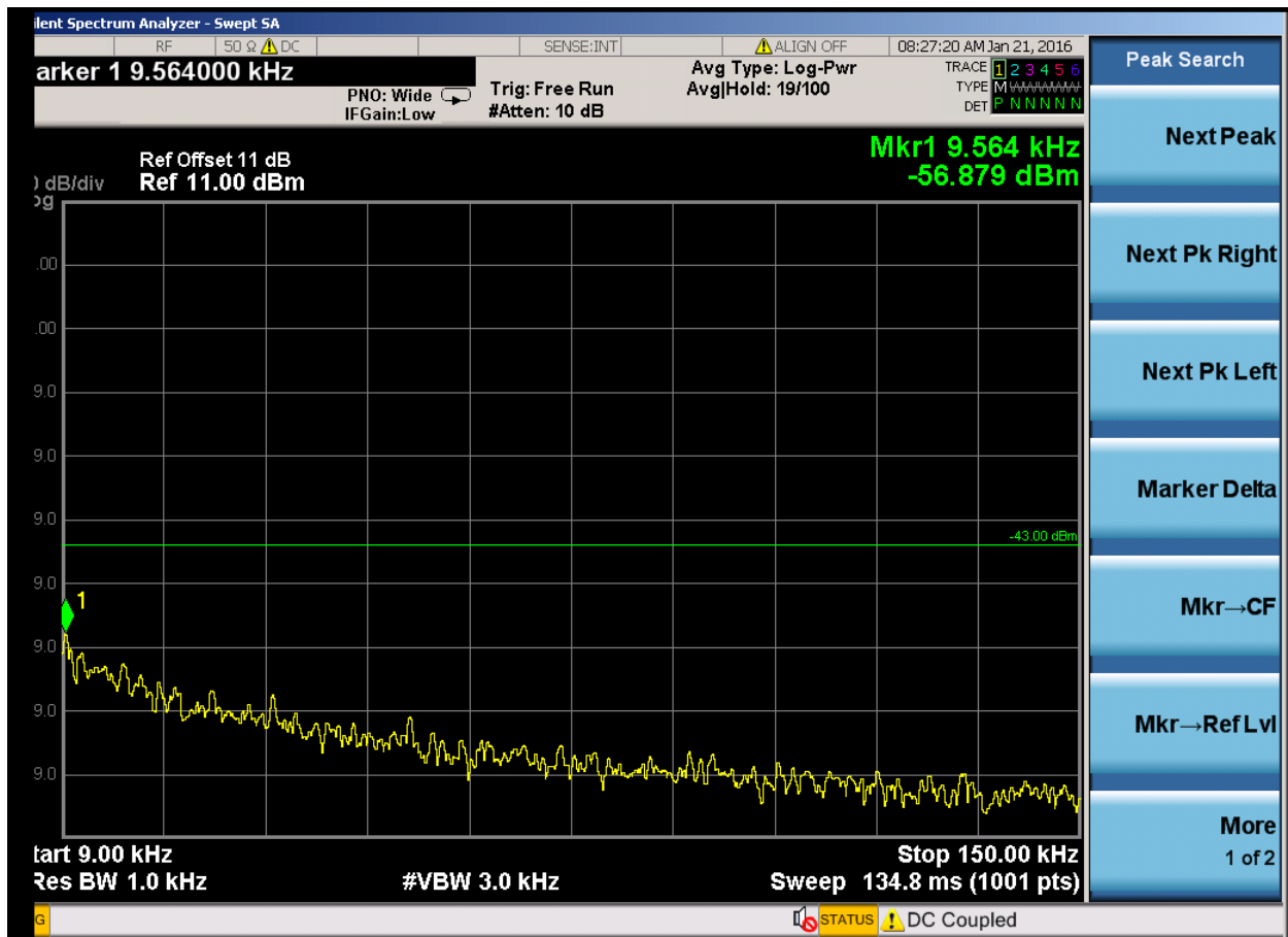
(Plot 4.5.2 B1: Channel 661: 1880.00MHz @ Traffic @ PCS1900)
