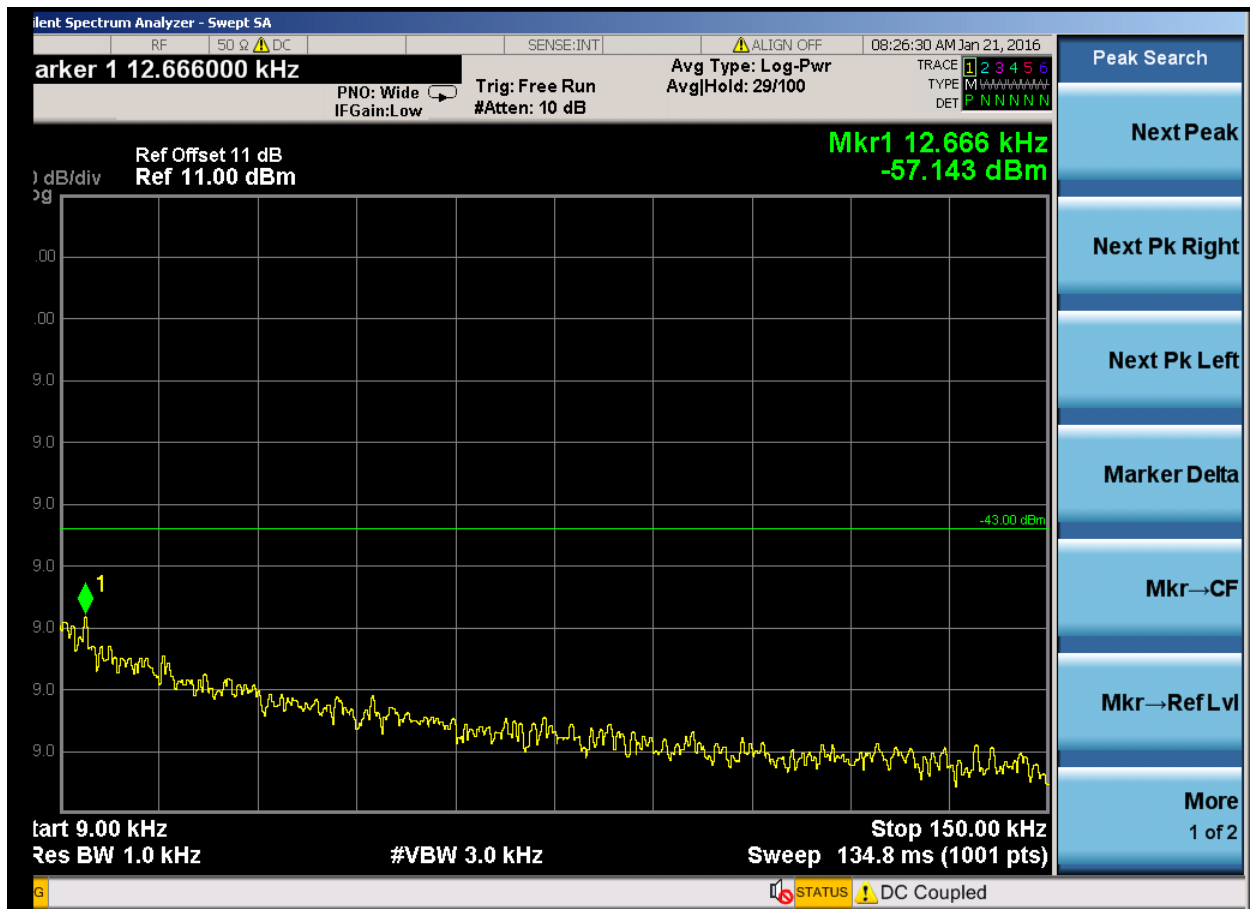
(Plot 4.5.1 B1: Channel 190: 836.60MHz @ Traffic @ GSM850)
