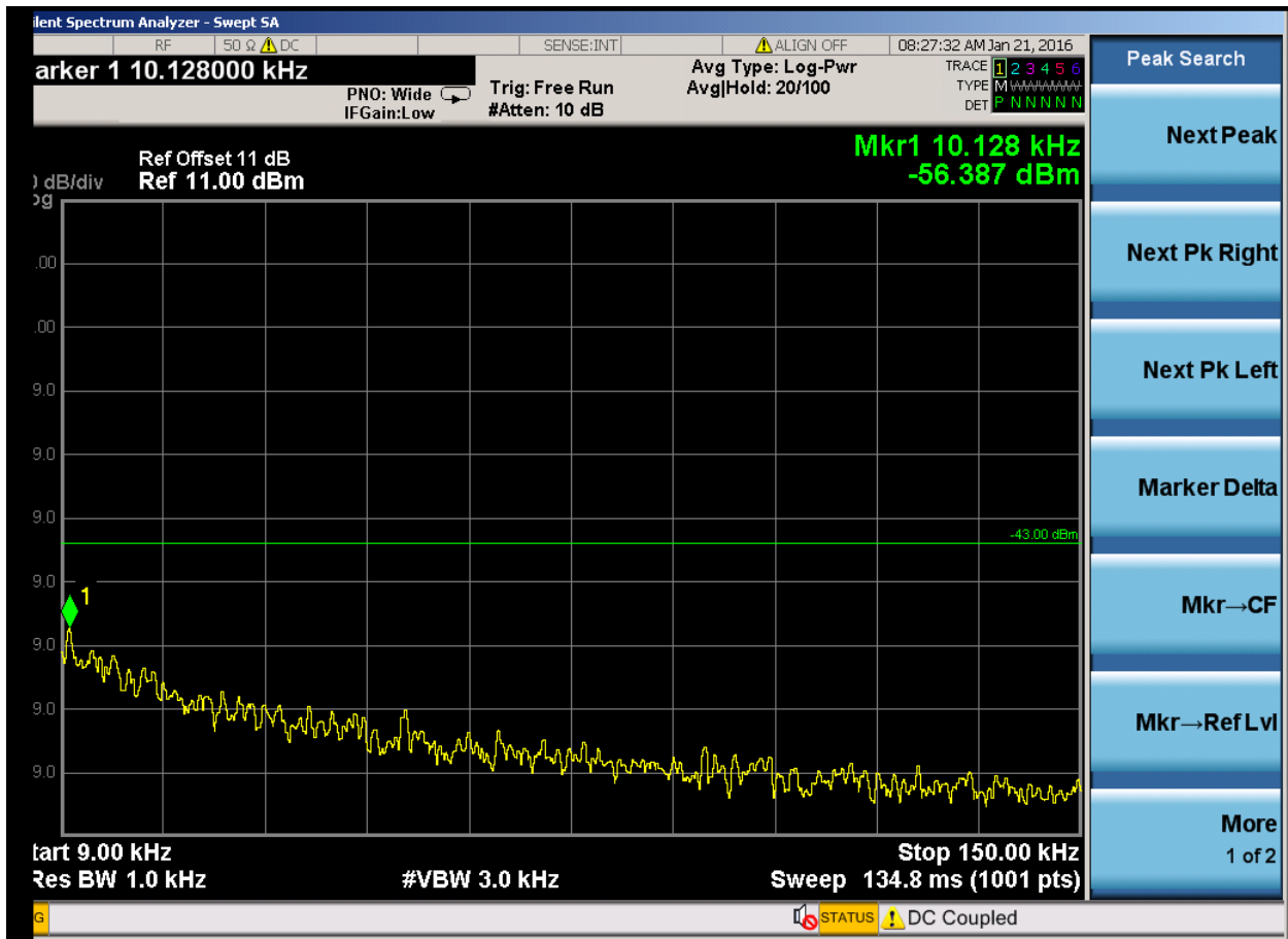
(Plot 4.5.2 C1: Channel 810: 1909.80MHz @ Traffic @ PCS1900)
