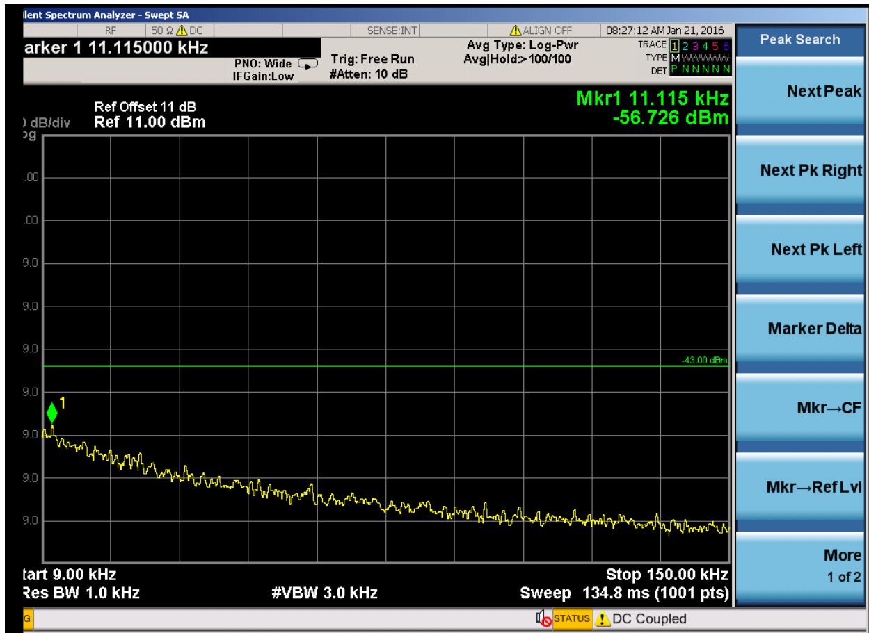
(Plot 4.5.2 A1: Channel 512: 1850.20MHz @ Traffic @ PCS1900)
