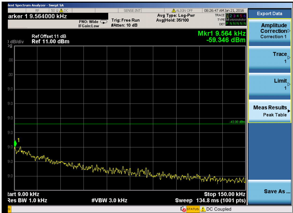
(Plot 4.5.1 C1: Channel 251: 848.80MHz @ Traffic @ GSM850)
