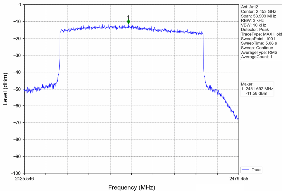
40MHz BW_HCH_2452.5MHz_Ant2_NTNV
