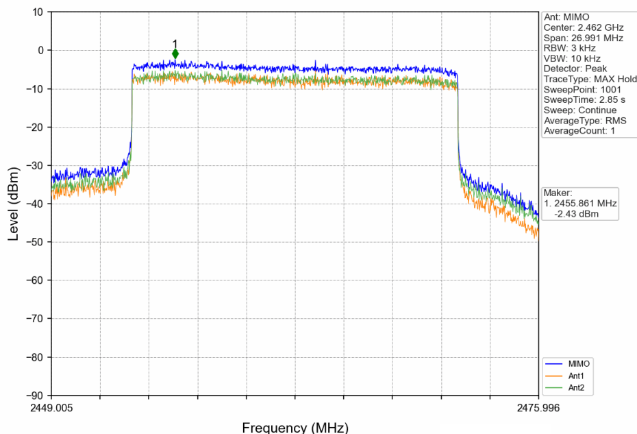
20MHz BW_HCH_2462.5MHz_MIMO_NTNV
