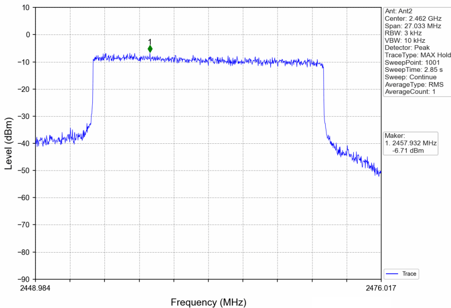
20MHz BW_HCH_2462.5MHz_Ant2_NTNV
