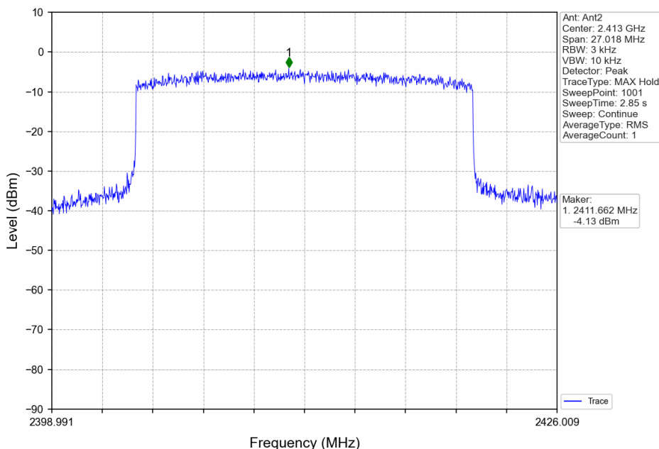
20MHz BW_LCH_2412.5MHz_MIMO_NTNV
