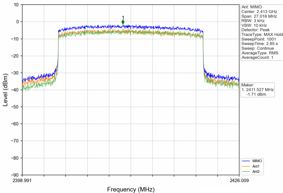
20MHz BW_LCH_2412.5MHz_MIMO_NTNV
