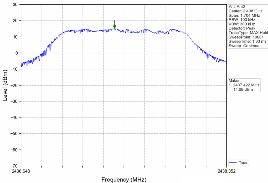
1.4MHz BW_MCH_2437.5MHz_Ant2_NTNV
