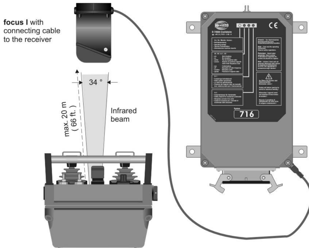
Function of infrakey (schematic view), e.g. spectrum 1 M radio transmitter and FSE 716 radio receiver
