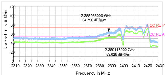
802.11ax HE20-Channel 1 Peak &amp; Average
