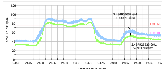
802.11ax HE20-Channel 11 Peak &amp; Average
