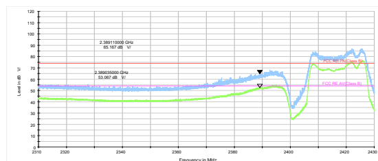
802.11ax HE20-Channel 2 Peak &amp; Average
