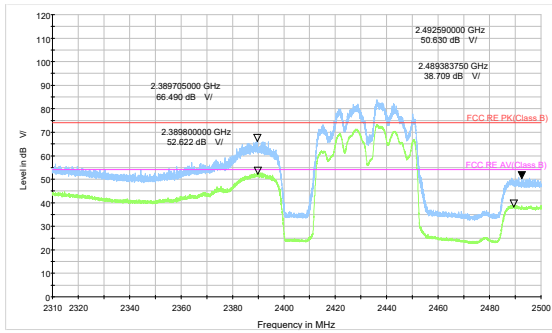
802.11ax HE40-Channel 5 Peak & Average
