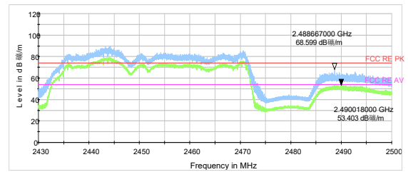
802.11ax HE40-Channel 9 Peak & Average
