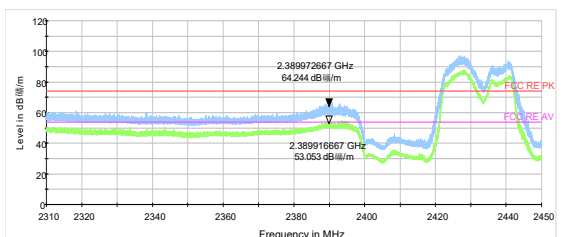
802.11ax HE20-Channel 5 Peak &amp; Average
