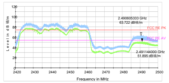
802.11ax HE40-Channel 7 Peak & Average
