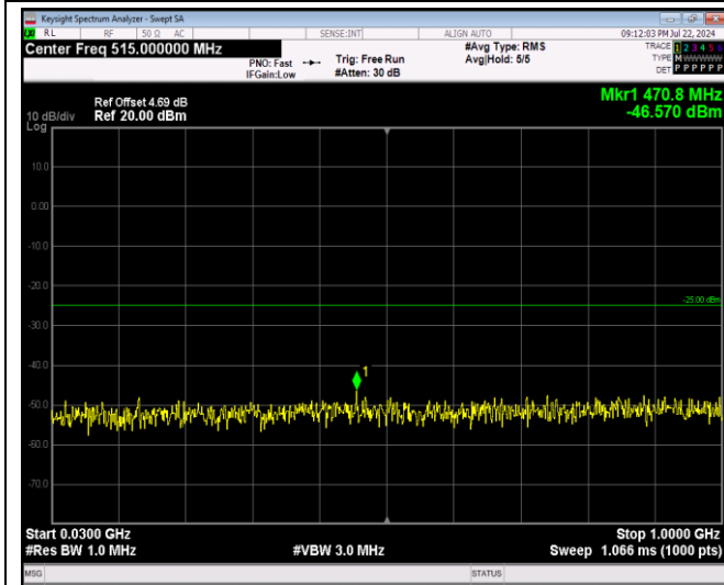
Band41-5MHz-64QAM-40640-1RB#0-Range1:30~1000MHz
