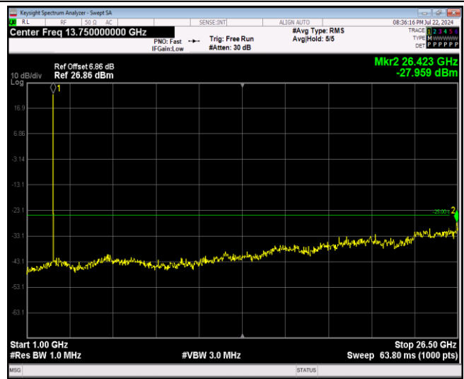
Band7-5MHz-16QAM-21425-1RB#0-Range2:1000~265 00MHz
