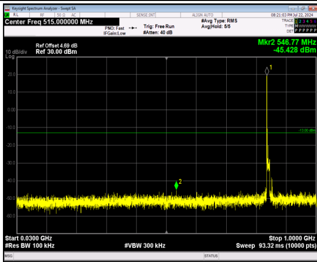
Band7-5MHz-QPSK-20775-1RB#0-Range1:30~1000MHz
