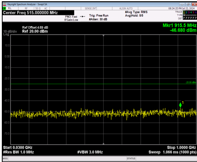
Band7-5MHz-64QAM-21100-1RB#0-Range1:30~100 00MHz
