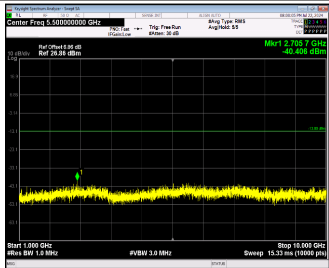
Band5-1.4MHz-64QAM-20407-1RB#0-Range2:1000~10 000MHz
