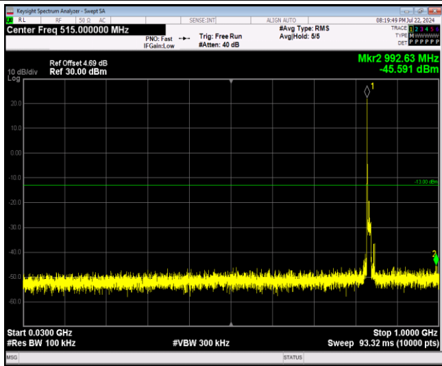
Band5-10MHz-16QAM-20525-1RB#0-Range1:30~1000MHz
