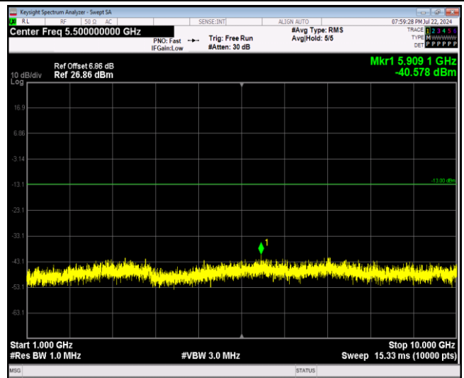
Band5-1.4MHz-64QAM-20643-1RB#0-Range2:1000~10000MHz
