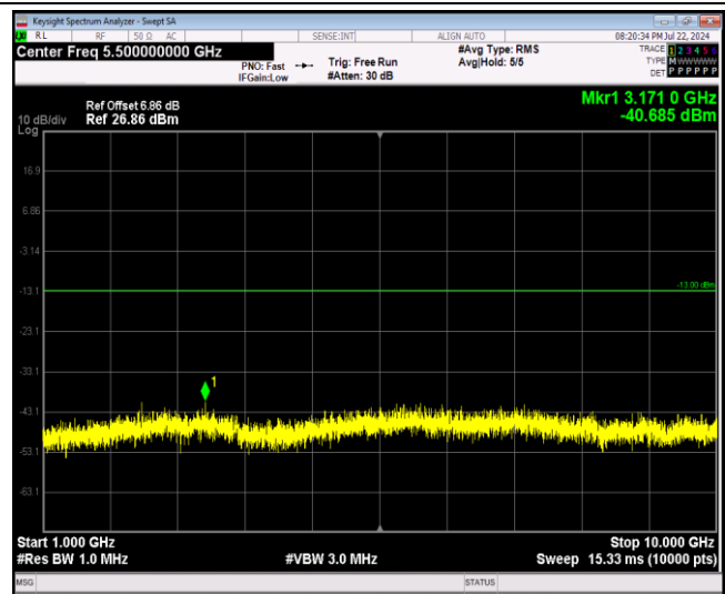
Band5-10MHz-16QAM-20450-1RB#0-Range2:1000~10000MHz
