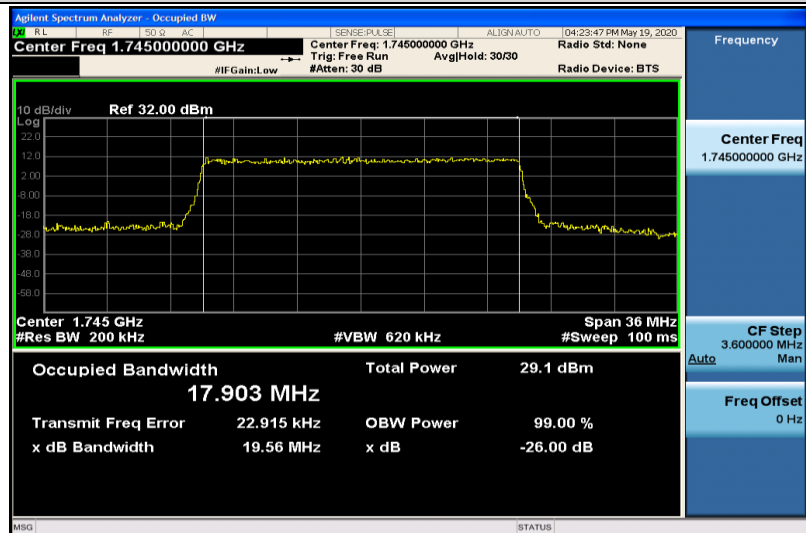
Band4-20MHz-16QAM-20300-100RB#0-17.903
