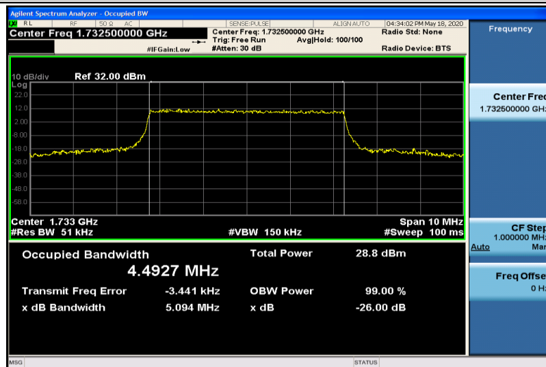
Band4-5MHz-16QAM-20175-25RB#0-4.4927
