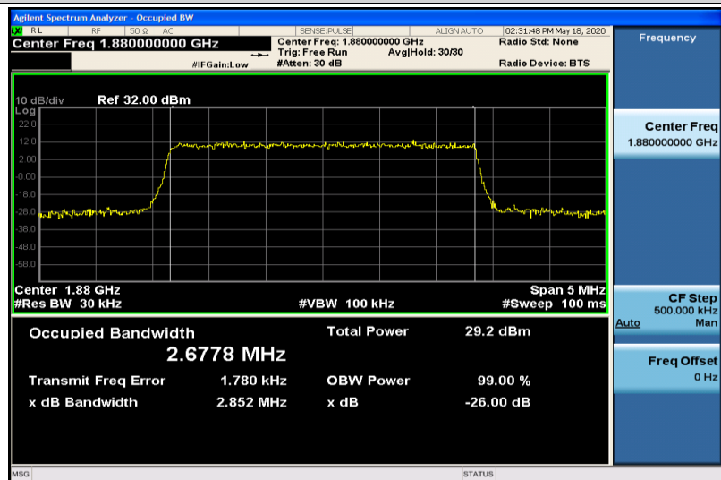
Band2-3MHz-QPSK-18900-15RB#0-2.6778
