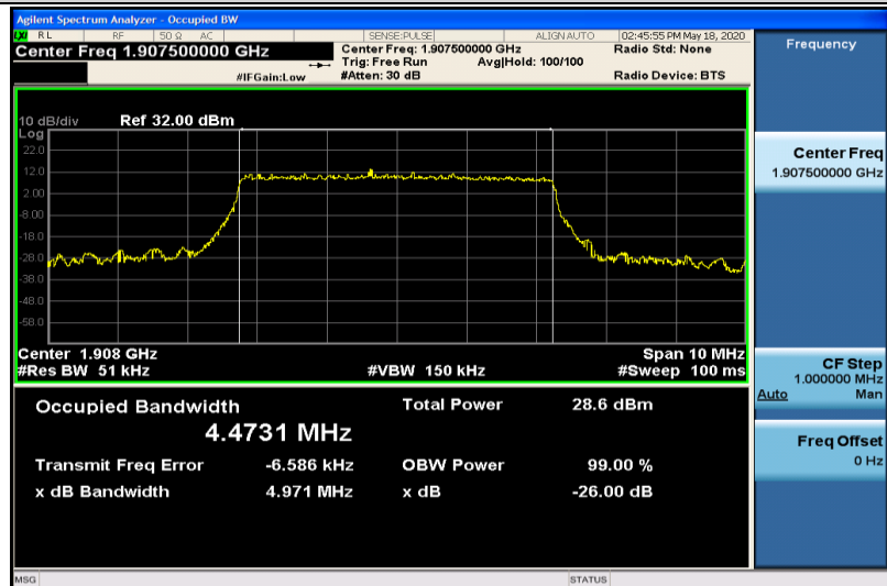
Band2-5MHz-16QAM-19175-25RB#0-4.4731
