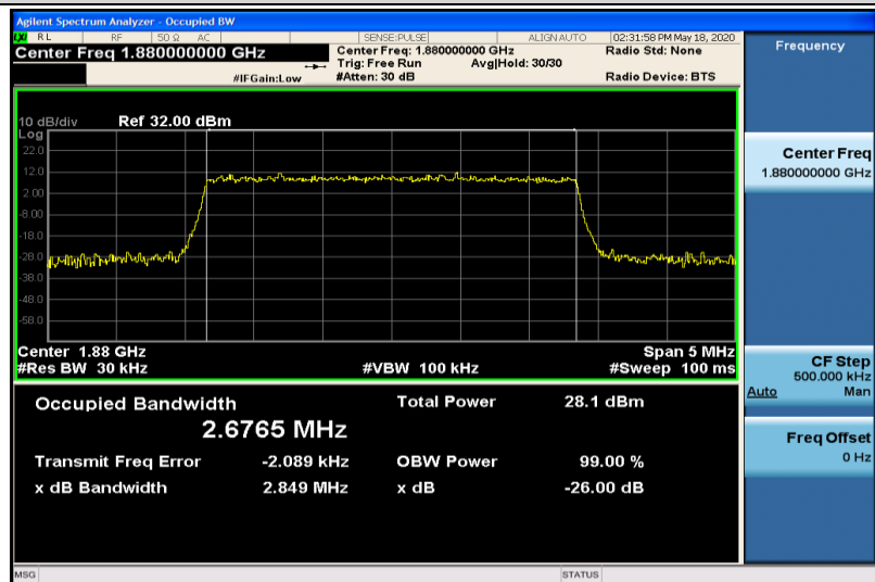
Band2-3MHz-16QAM-18900-15RB#0-2.6765
