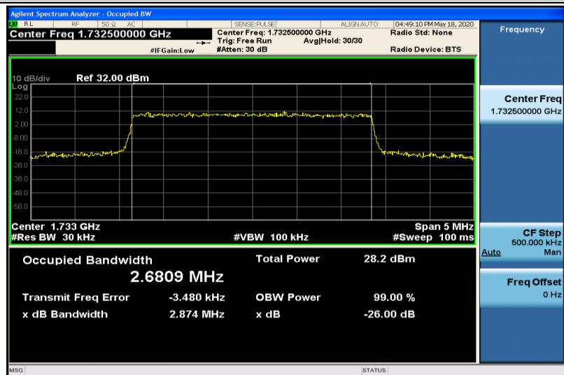
Band4-3MHz-16QAM-20175-15RB#0-2.6809
