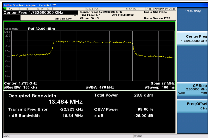
Band4-15MHz-16QAM-20175-75RB#0-13.484
