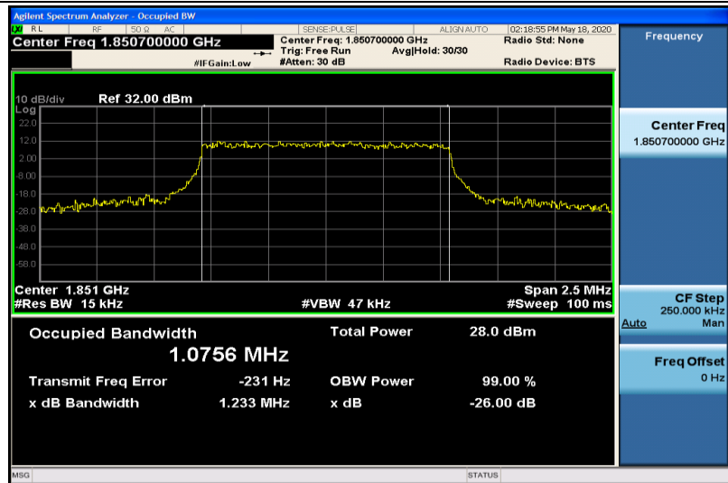
Band2-1.4MHz-16QAM-18607-6RB#0-1.0756
