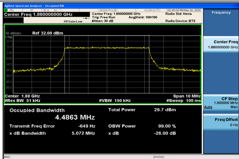
Band2-5MHz-QPSK-18900-25RB#0-4.4863
