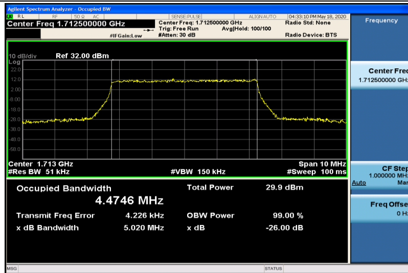
Band4-5MHz-QPSK-19975-25RB#0-4.4746
