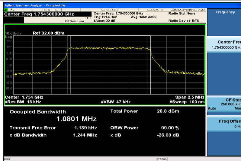
Band4-1.4MHz-QPSK-20393-6RB#0-1.0801
