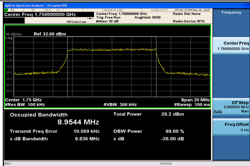
Band4-10MHz-16QAM-20350-50RB#0-8.9544
