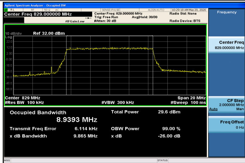
Band5-10MHz-QPSK-20450-50RB#0-8.9393
