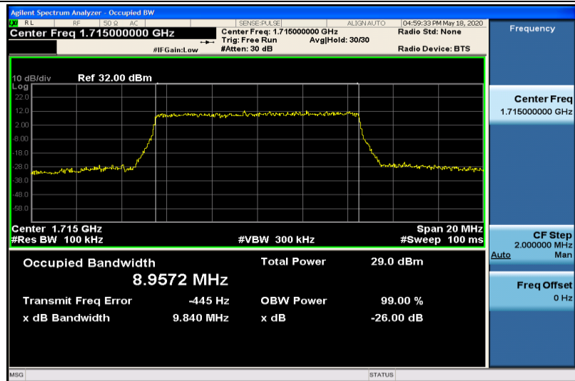
Band4-10MHz-16QAM-20000-50RB#0-8.9572
