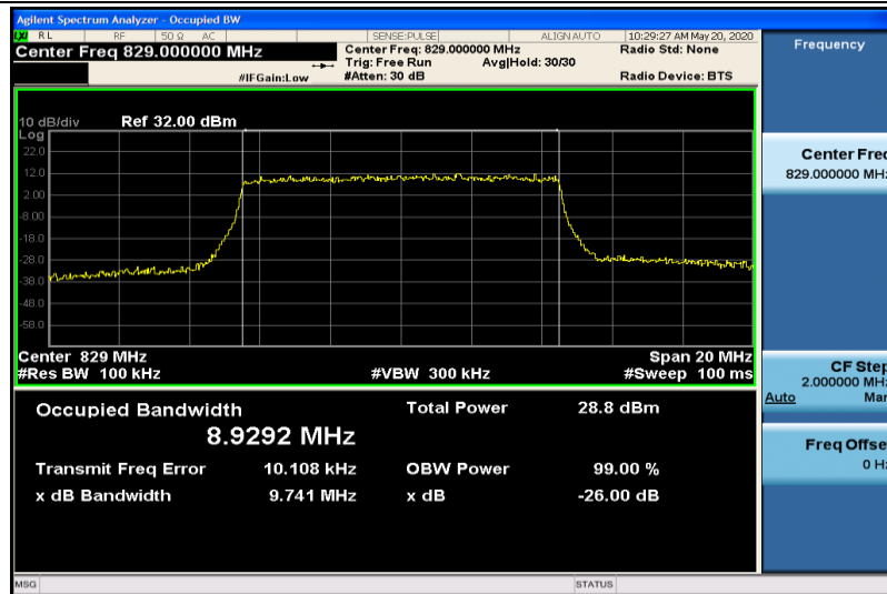
Band5-10MHz-16QAM-20450-50RB#0-8.9292
