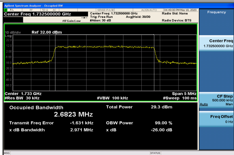
Band4-3MHz-QPSK-20175-15RB#0-2.6823
