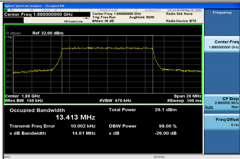
Band2-15MHz-QPSK-18900-75RB#0-13.413
