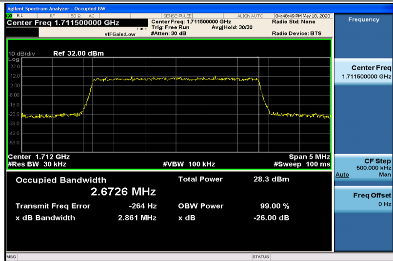
Band4-3MHz-16QAM-19965-15RB#0-2.6726
