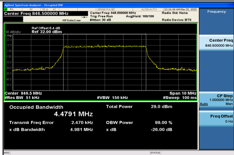
Band5-5MHz-16QAM-20625-25RB#0-4.4791
