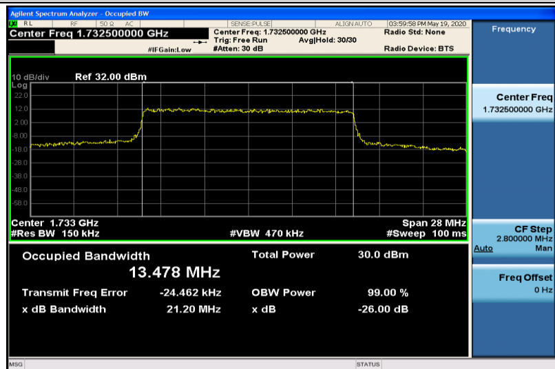
Band4-15MHz-QPSK-20175-75RB#0-13.478
