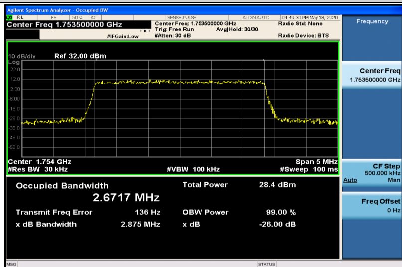
Band4-3MHz-16QAM-20385-15RB#0-2.6717
