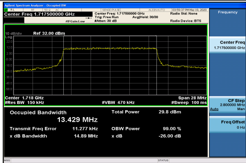
Band4-15MHz-QPSK-20025-75RB#0-13.429
