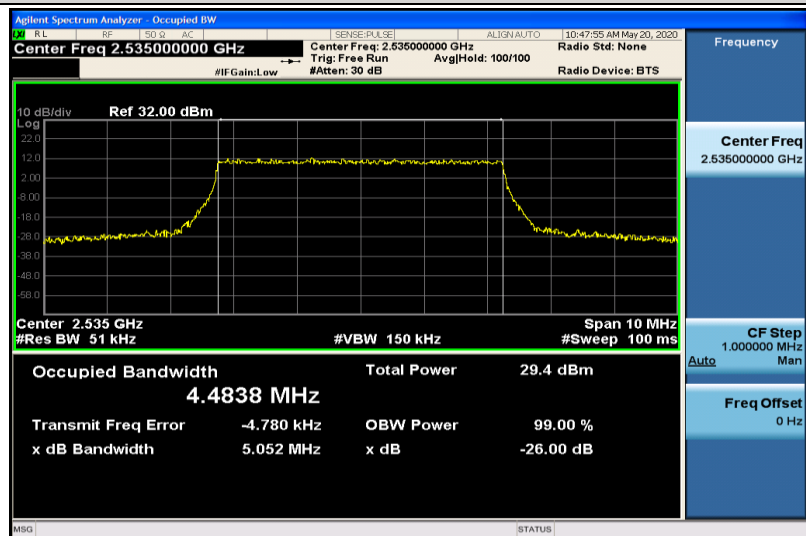
Band7-5MHz-QPSK-21100-25RB#0-4.4838
