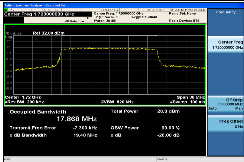
Band4-20MHz-16QAM-20050-100RB#0-17.868
