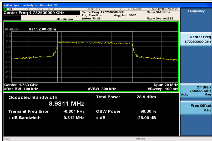
Band4-10MHz-16QAM-20175-50RB#0-8.9811
