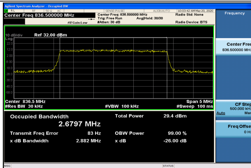
Band5-3MHz-QPSK-20525-15RB#0-2.6797
