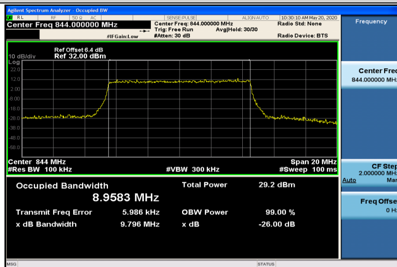
Band5-10MHz-16QAM-20600-50RB#0-8.9583
