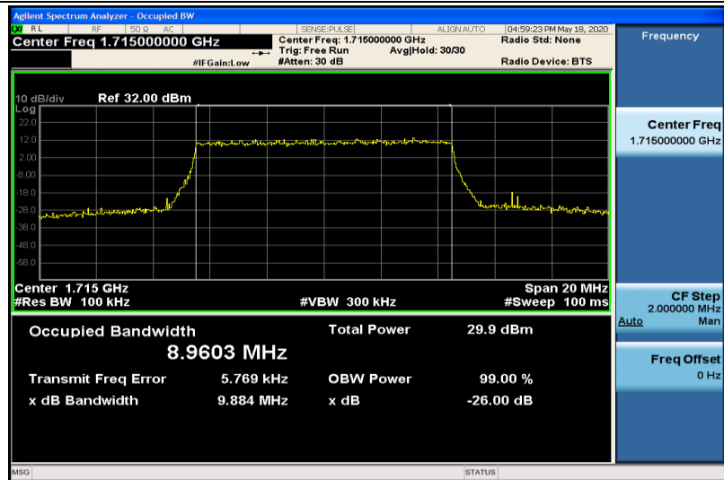
Band4-10MHz-QPSK-20000-50RB#0-8.9603
