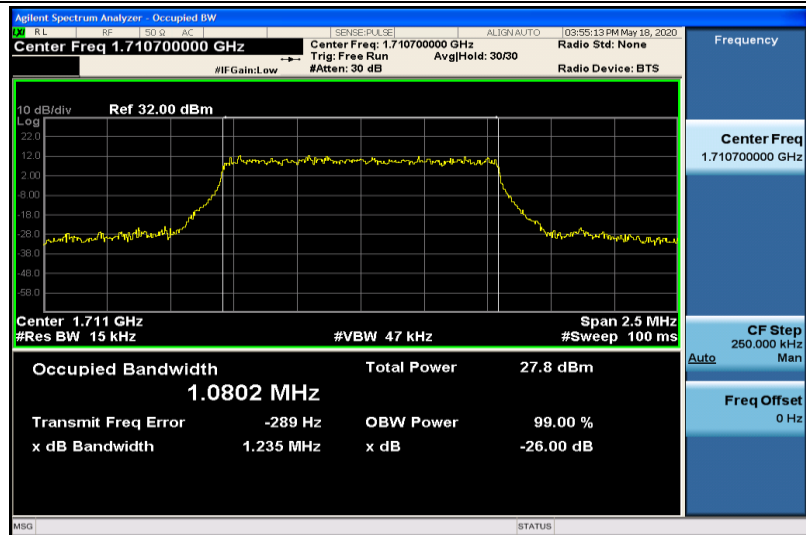
Band4-1.4MHz-16QAM-19957-6RB#0-1.0802
