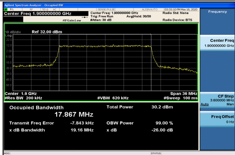
Band2-20MHz-QPSK-19100-100RB#0-17.867
