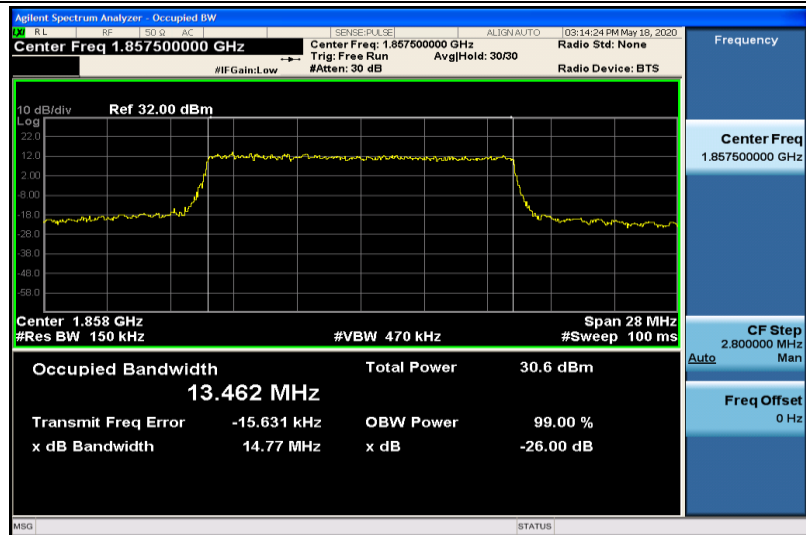
Band2-15MHz-QPSK-18675-75RB#0-13.462
