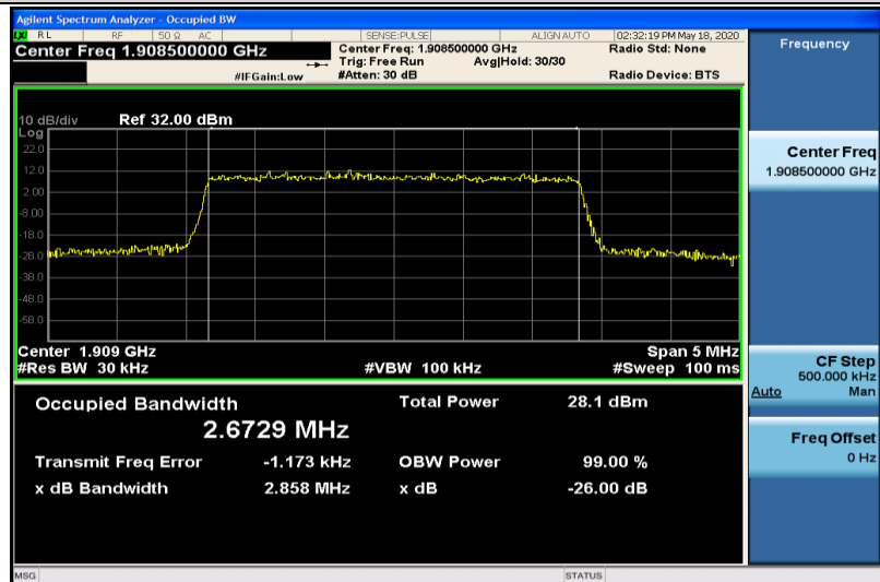
Band2-3MHz-16QAM-19185-15RB#0-2.6729
