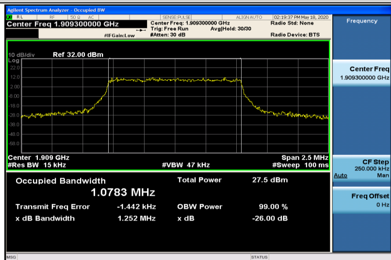
Band2-1.4MHz-16QAM-19193-6RB#0-1.0783
