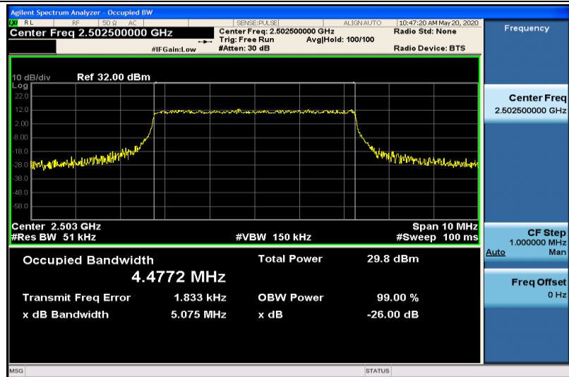
Band7-5MHz-QPSK-20775-25RB#0-4.4772
