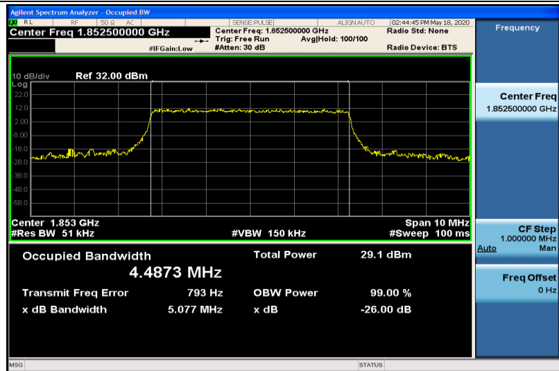
Band2-5MHz-16QAM-18625-25RB#0-4.4873
