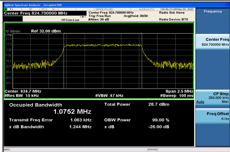
Band5-1.4MHz-QPSK-20407-6RB#0-1.0752
