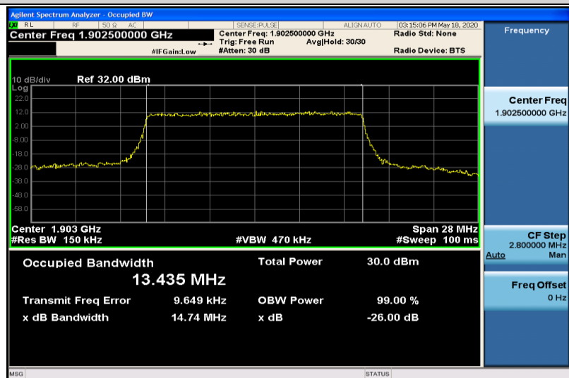
Band2-15MHz-QPSK-19125-75RB#0-13.435
