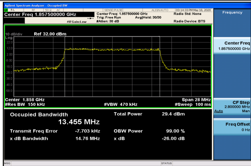
Band2-15MHz-16QAM-18675-75RB#0-13.455
