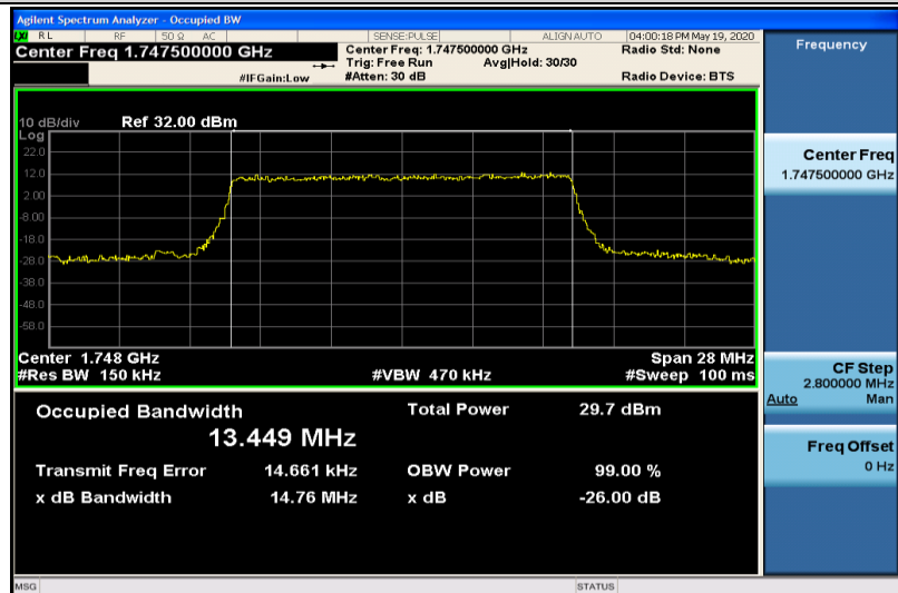
Band4-15MHz-QPSK-20325-75RB#0-13.449
