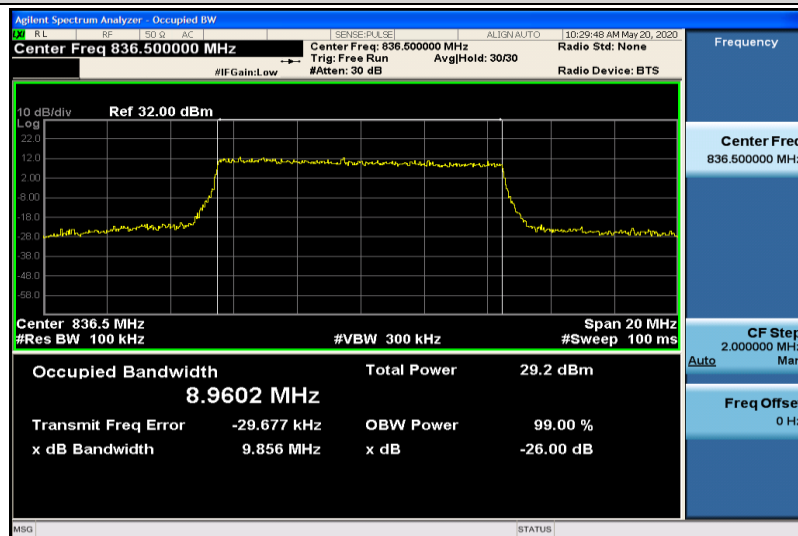
Band5-10MHz-16QAM-20525-50RB#0-8.9602
