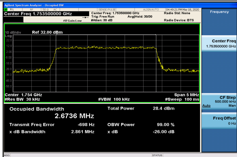
Band4-3MHz-QPSK-20385-15RB#0-2.6736
