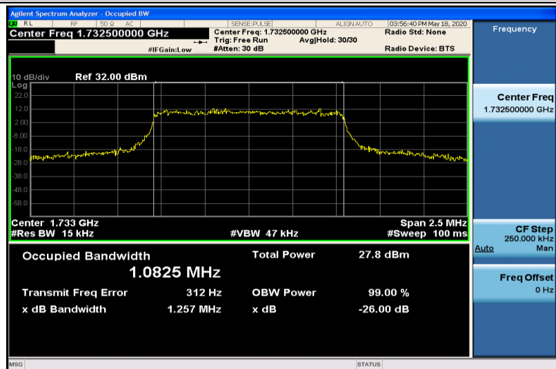
Band4-1.4MHz-16QAM-20175-6RB#0-1.0825
