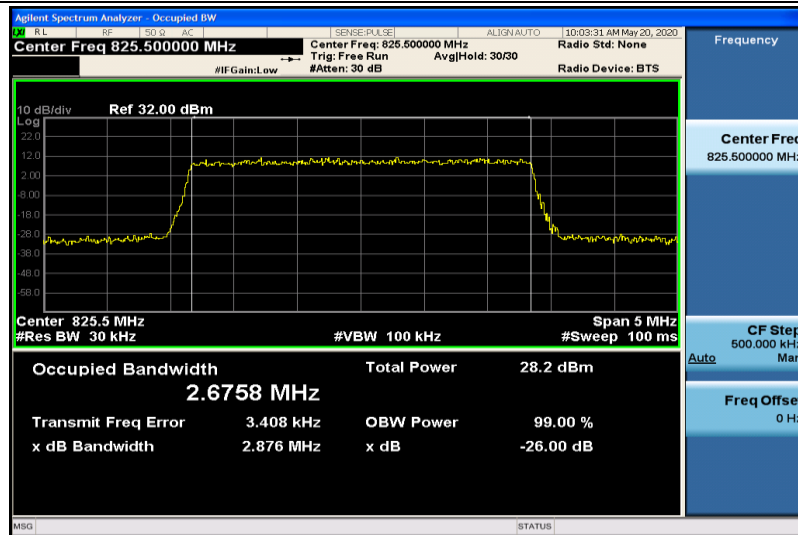
Band5-3MHz-16QAM-20415-15RB#0-2.6758
