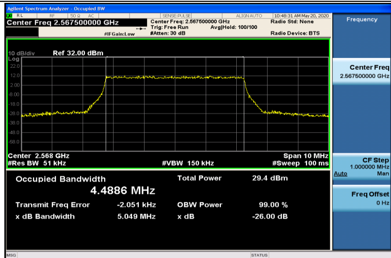
Band7-5MHz-QPSK-21425-25RB#0-4.4886
