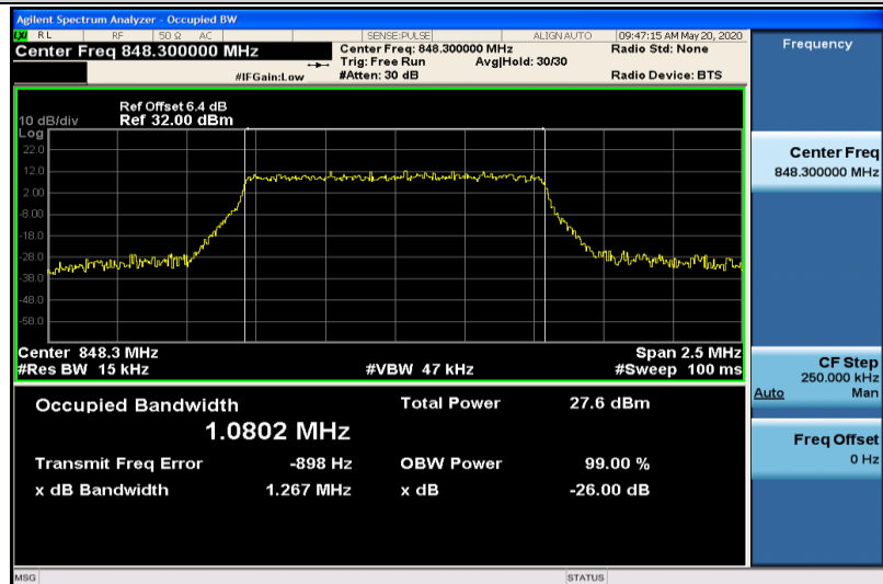
Band5-1.4MHz-16QAM-20643-6RB#0-1.0802
