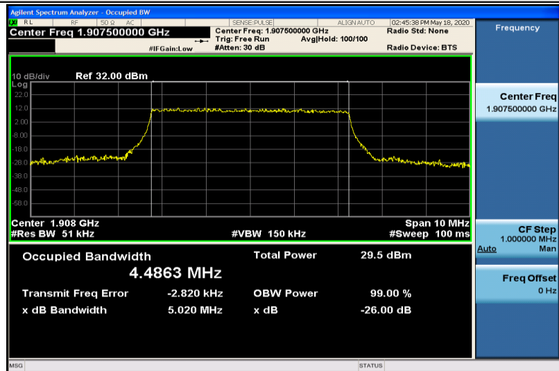
Band2-5MHz-QPSK-19175-25RB#0-4.4863
