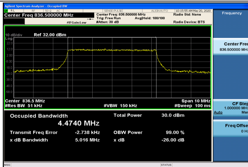
Band5-5MHz-QPSK-20525-25RB#0-4.4740
