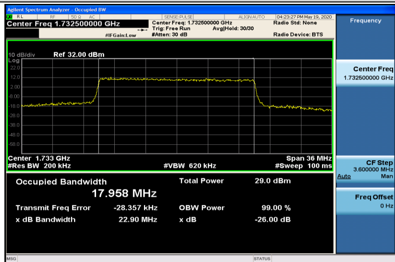
Band4-20MHz-16QAM-20175-100RB#0-17.958
