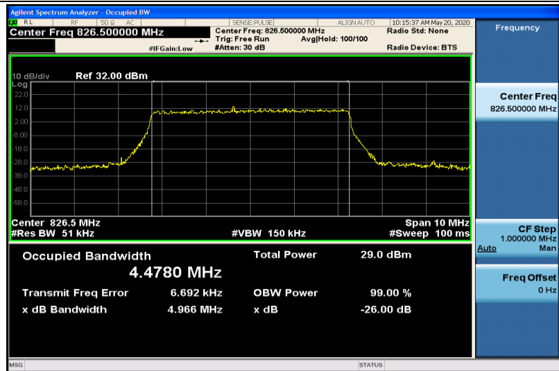
Band5-5MHz-16QAM-20425-25RB#0-4.4780
