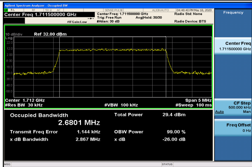
Band4-3MHz-QPSK-19965-15RB#0-2.6801
