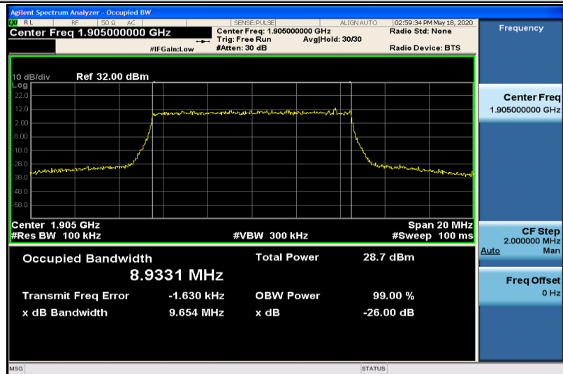
Band2-10MHz-16QAM-19150-50RB#0-8.9331
