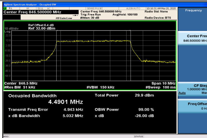
Band5-5MHz-QPSK-20625-25RB#0-4.4901
