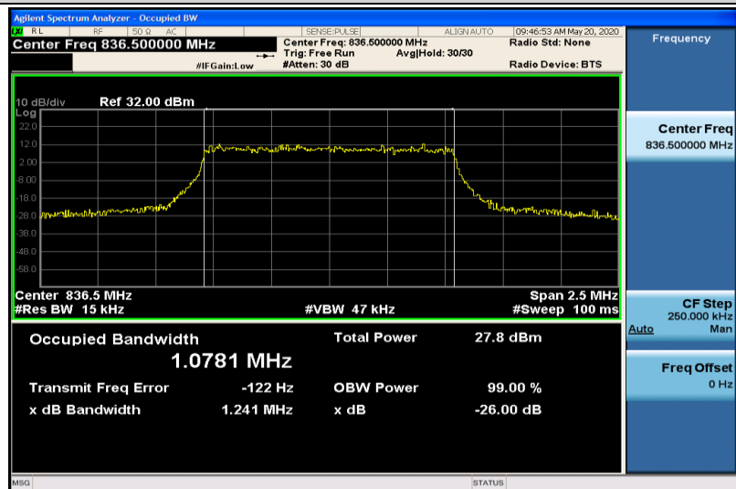
Band5-1.4MHz-16QAM-20525-6RB#0-1.0781
