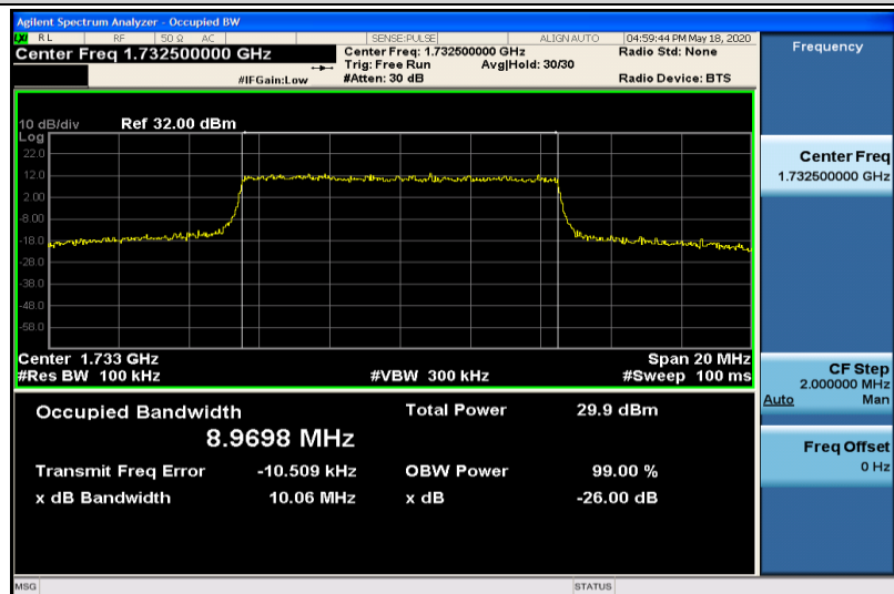
Band4-10MHz-QPSK-20175-50RB#0-8.9698
