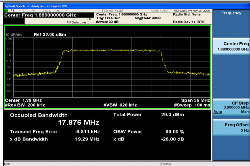
Band2-20MHz-16QAM-18900-100RB#0-17.876
