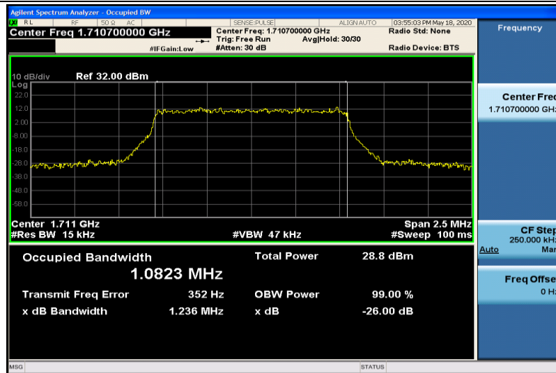
Band4-1.4MHz-QPSK-19957-6RB#0-1.0823
