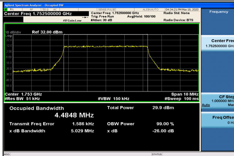
Band4-5MHz-QPSK-20375-25RB#0-4.4848
