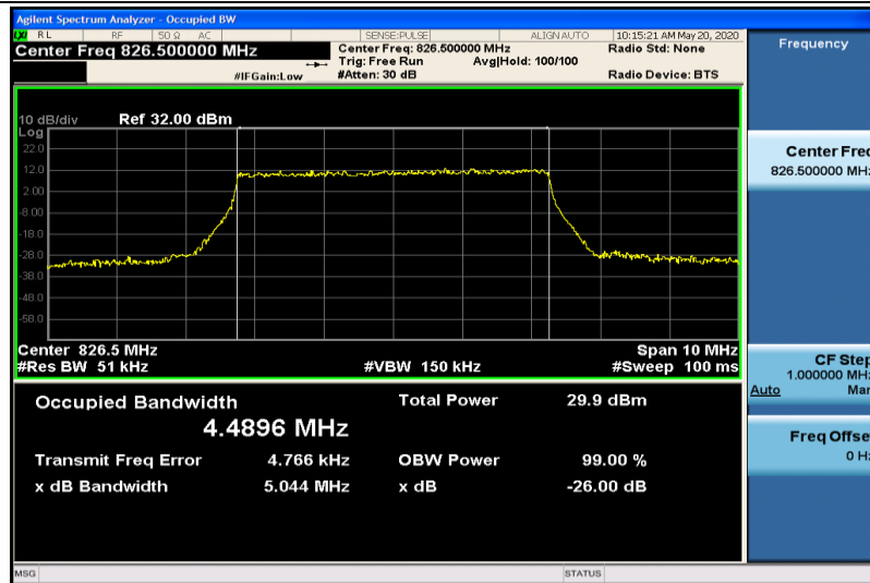
Band5-5MHz-QPSK-20425-25RB#0-4.4896
