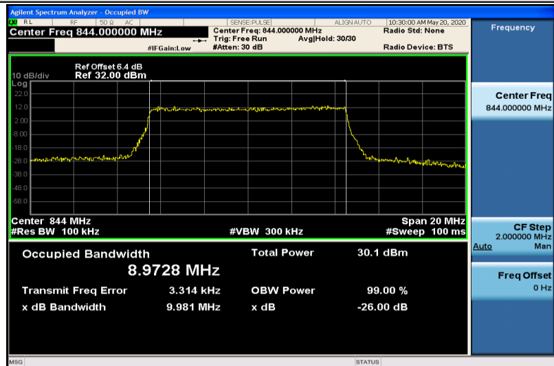
Band5-10MHz-QPSK-20600-50RB#0-8.9728
