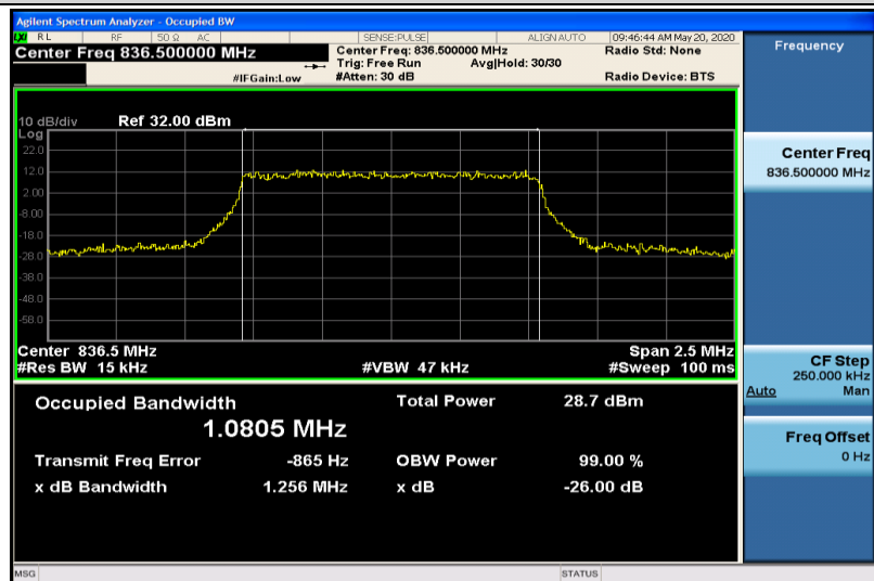
Band5-1.4MHz-QPSK-20525-6RB#0-1.0805
