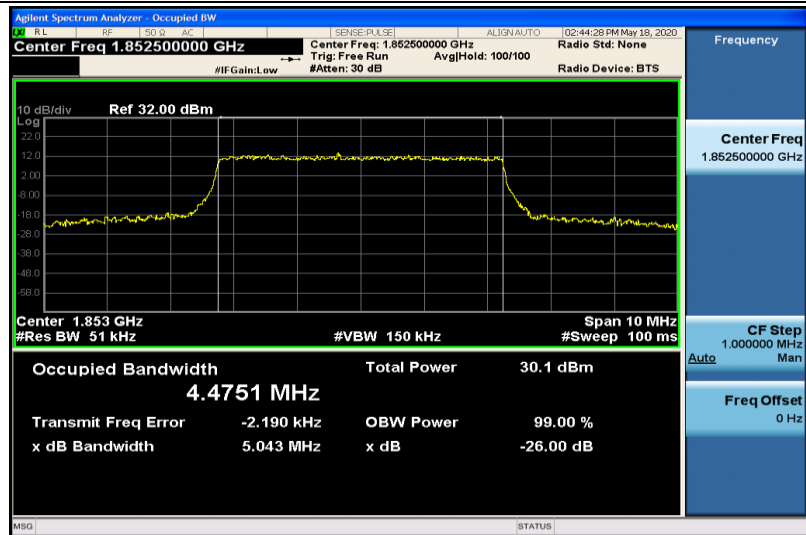
Band2-5MHz-QPSK-18625-25RB#0-4.4751
