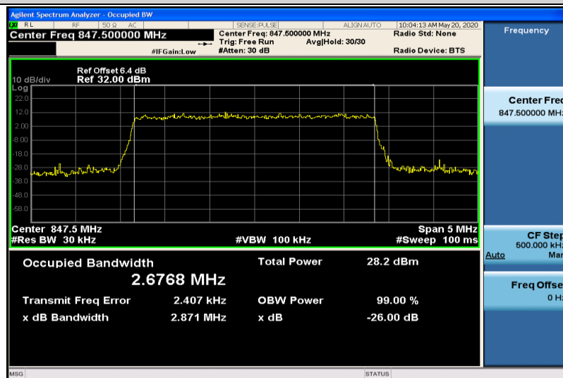
Band5-3MHz-16QAM-20635-15RB#0-2.6768
