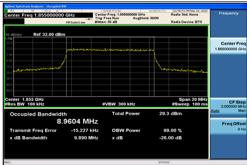
Band2-10MHz-16QAM-18650-50RB#0-8.9604
