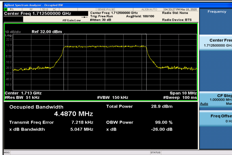
Band4-5MHz-16QAM-19975-25RB#0-4.4870
