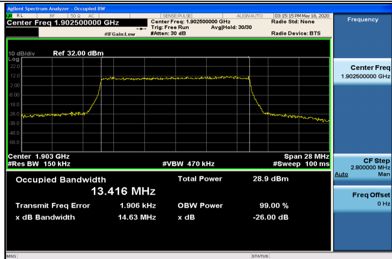
Band2-15MHz-16QAM-19125-75RB#0-13.416
