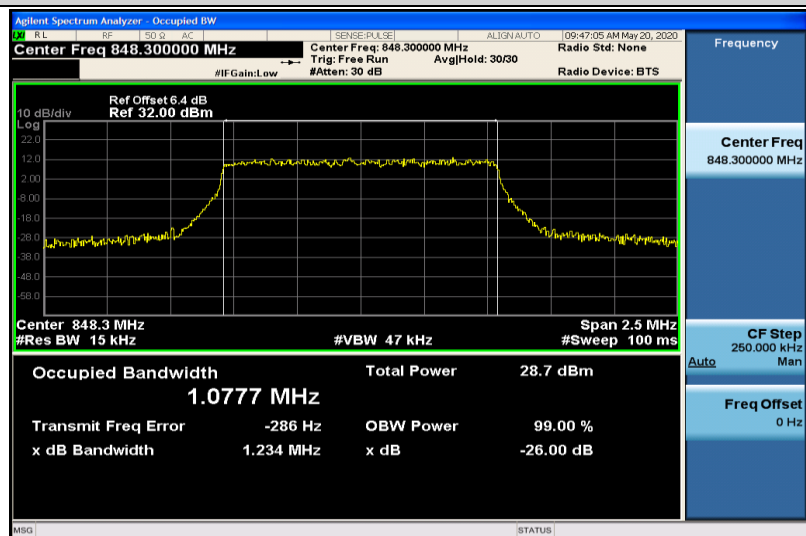
Band5-1.4MHz-QPSK-20643-6RB#0-1.0777
