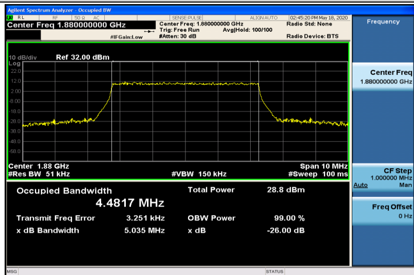
Band2-5MHz-16QAM-18900-25RB#0-4.4817
