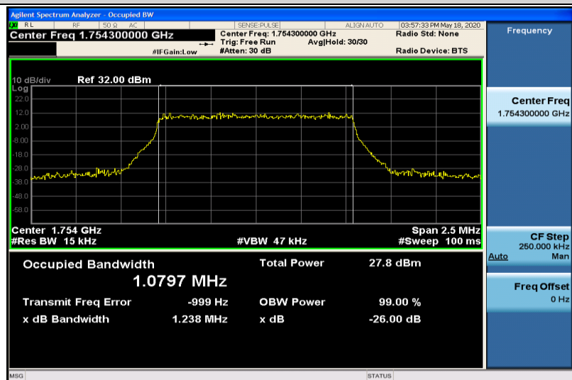
Band4-1.4MHz-16QAM-20393-6RB#0-1.0797
