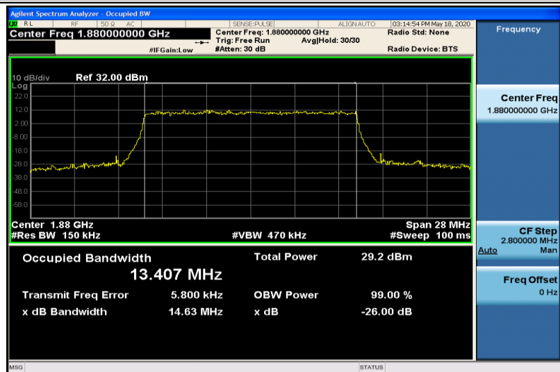
Band2-15MHz-16QAM-18900-75RB#0-13.407
