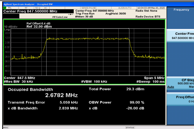
Band5-3MHz-QPSK-20635-15RB#0-2.6782
