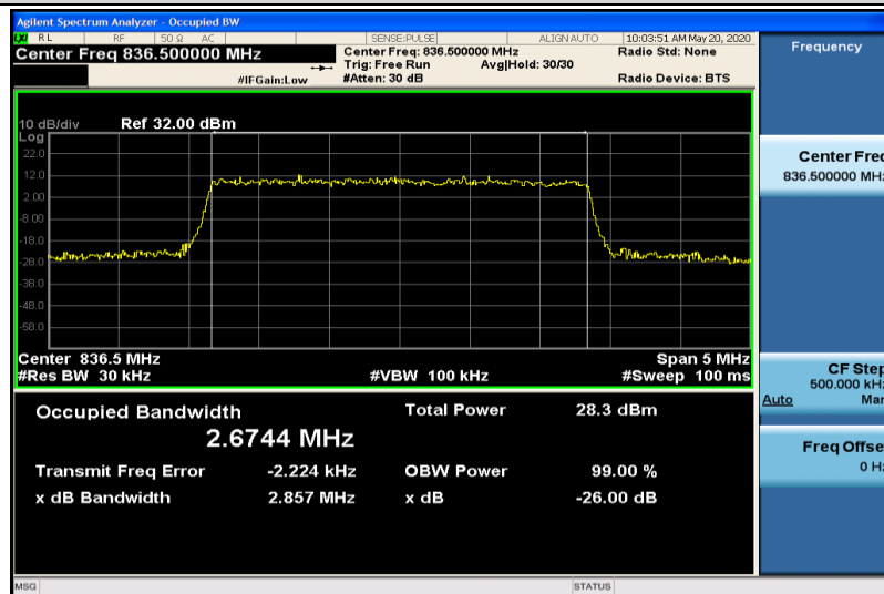
Band5-3MHz-16QAM-20525-15RB#0-2.6744
