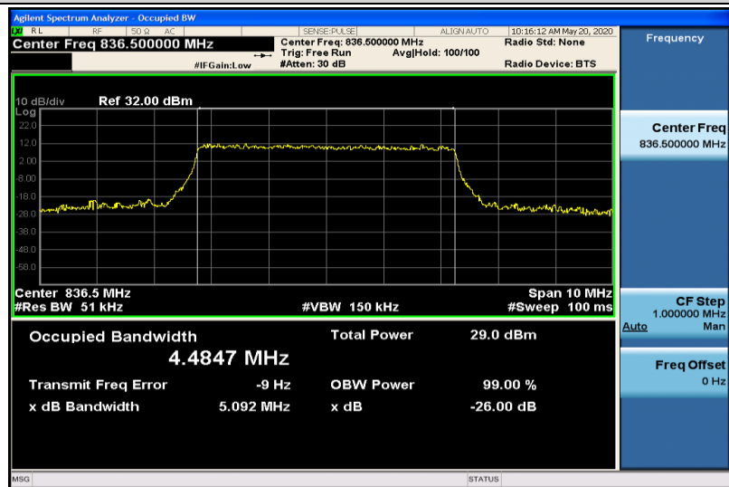
Band5-5MHz-16QAM-20525-25RB#0-4.4847
