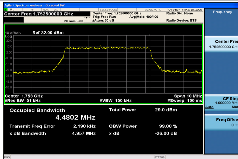
Band4-5MHz-16QAM-20375-25RB#0-4.4802
