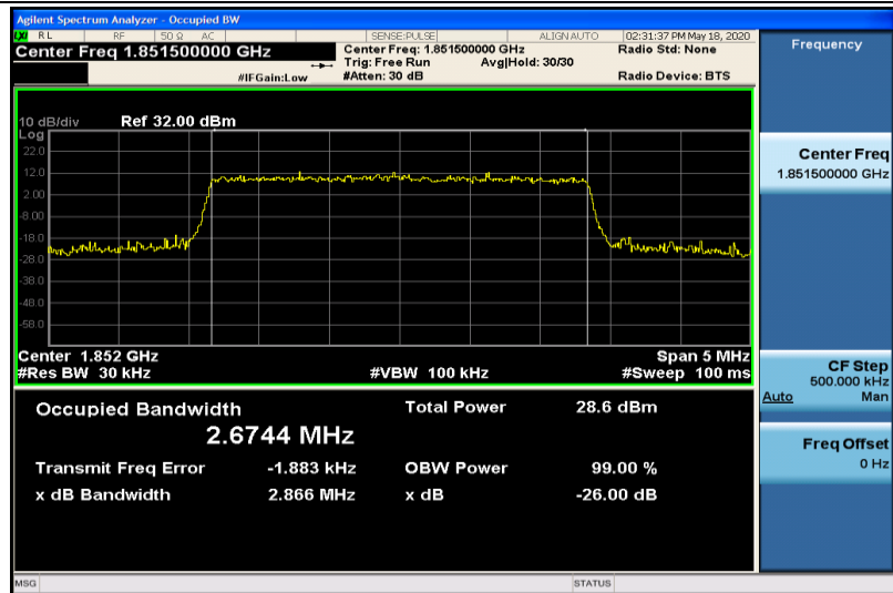
Band2-3MHz-16QAM-18615-15RB#0-2.6744
