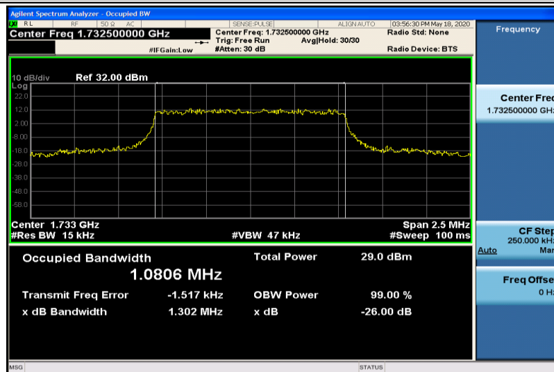
Band4-1.4MHz-QPSK-20175-6RB#0-1.0806
