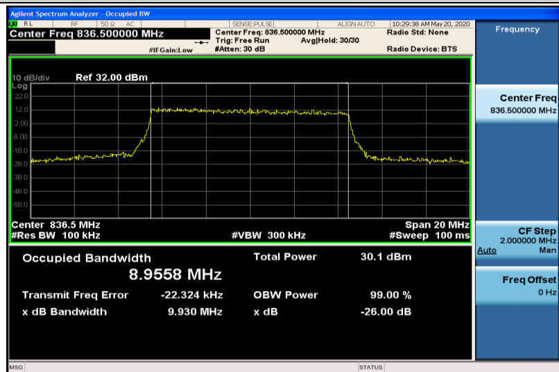
Band5-10MHz-QPSK-20525-50RB#0-8.9558
