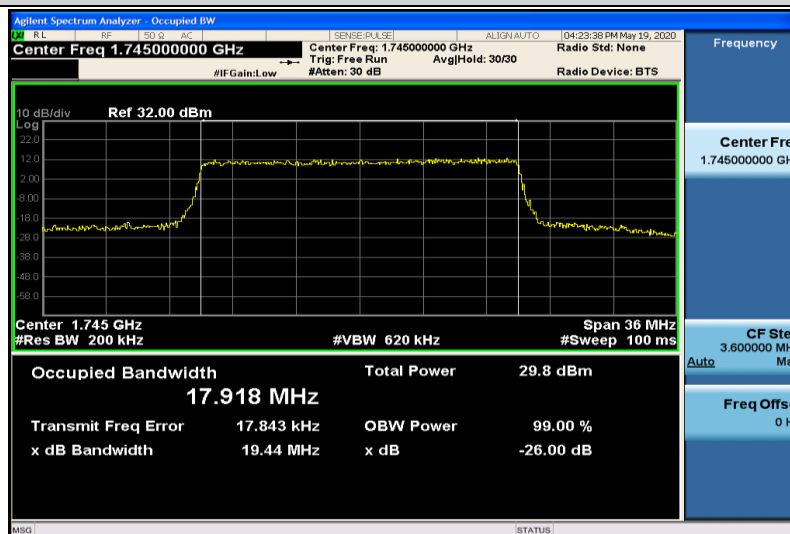
Band4-20MHz-QPSK-20300-100RB#0-17.918
