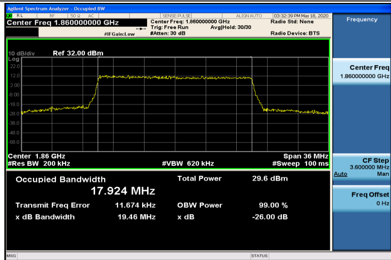
Band2-20MHz-16QAM-18700-100RB#0-17.924
