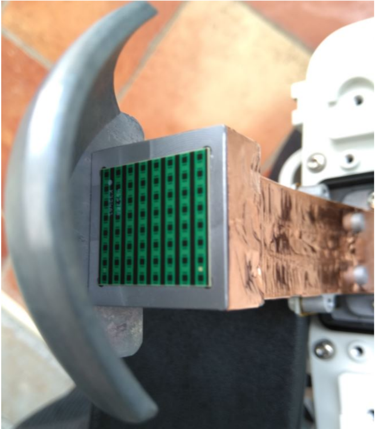
V3000 SSPXA-001326 SWL-QD46 RF Tile Front View
