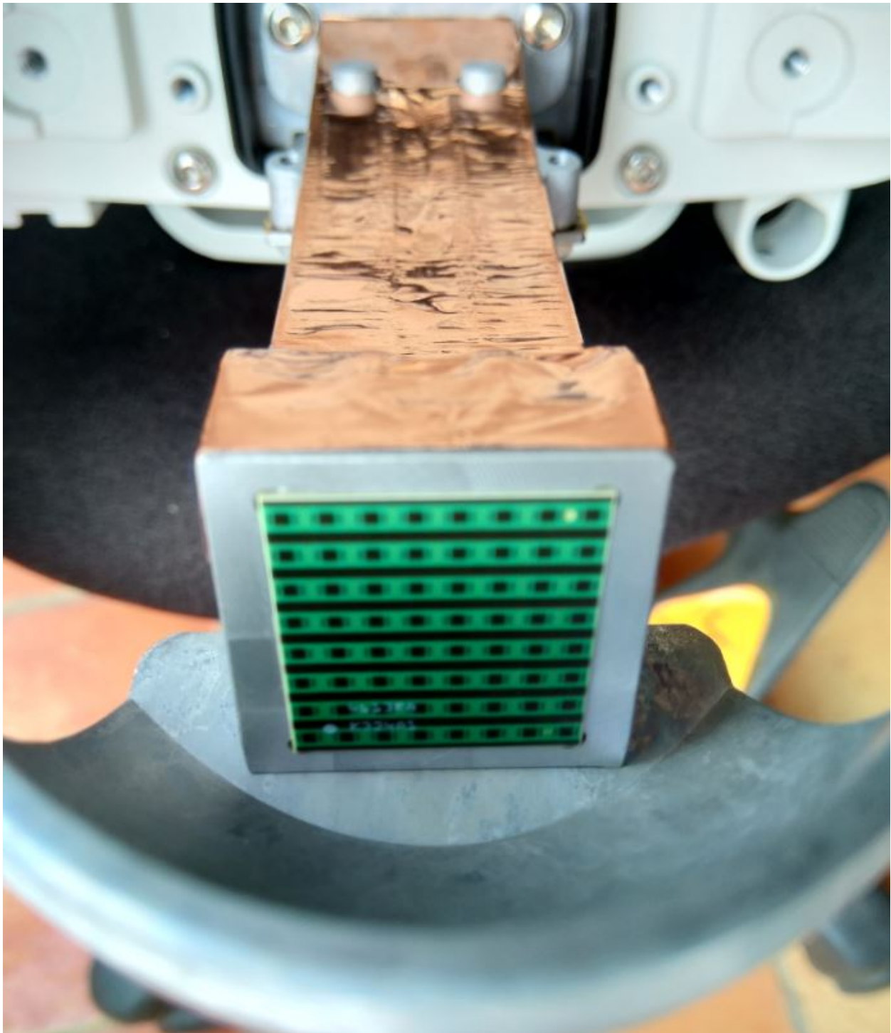
V3000 SSPXA-001326 SWL-QD46 RF Tile Bottom View
