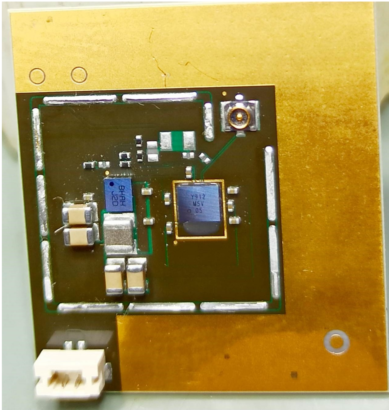
SSPXA-001326 SWL-QD46 RF Tile Top View (Can Removed)
