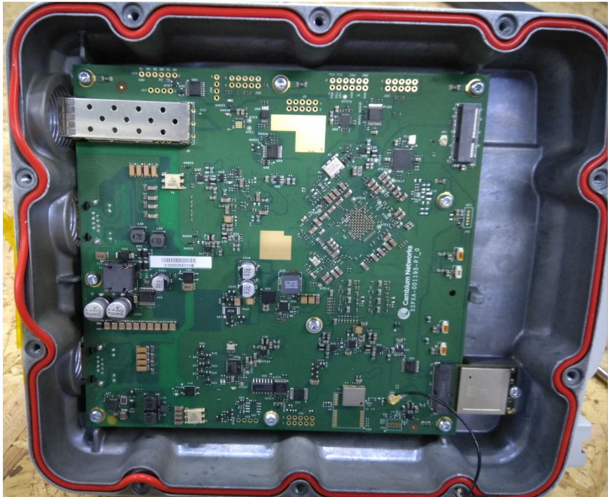
V3000 SSAXA-001000 in Casting Front View
