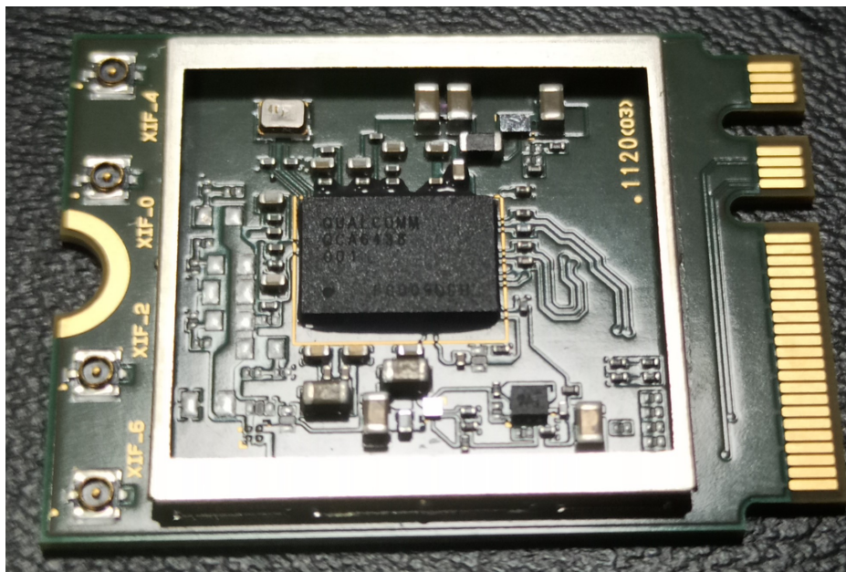
SSPXA-001325 BaseBand Module top View
