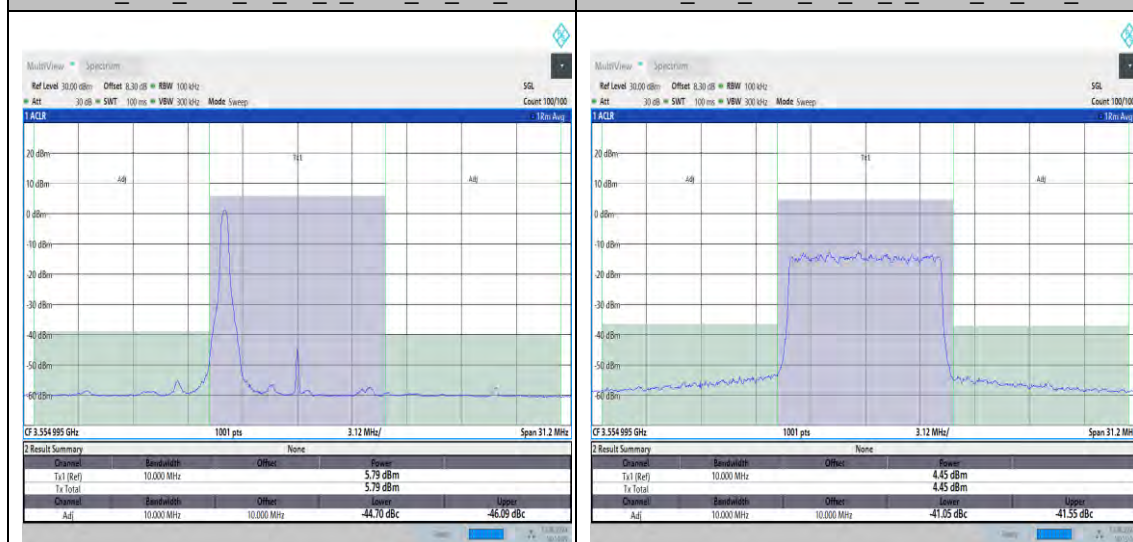
NTNV_N48_PC3_30_10_L_TID5_#1_-10_10
