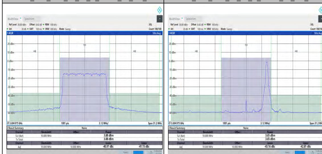
NTNV_N48_PC3_30_10_H_TID19_#1_-10_10
