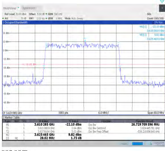
1-N48-30-30-M-5-DFT-256QAM-Outer_Full-75@0-A nt0-26.732-28.020-≤30-PASS
