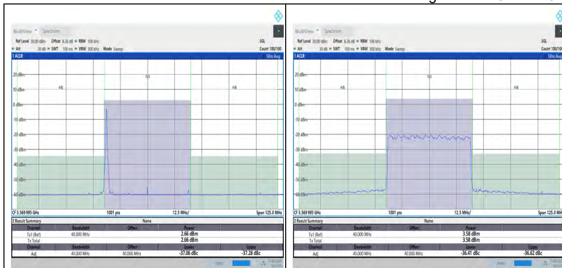
NTNV_N48_PC3_30_40_L_TID14_#1_-40_40
