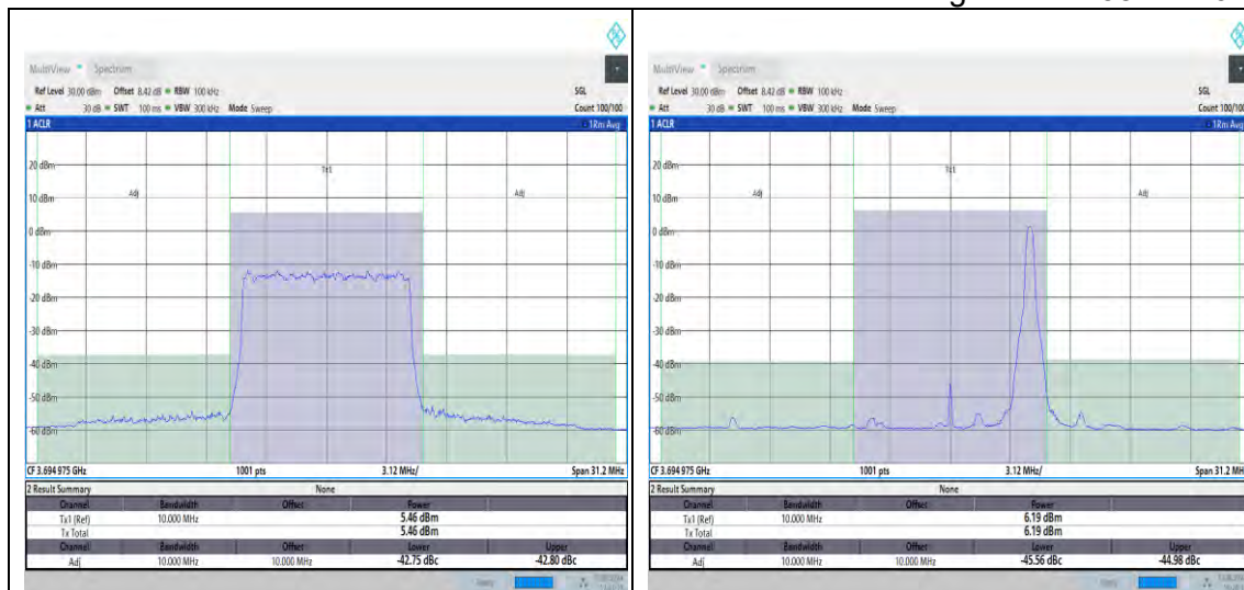
NTNV_N48_PC3_30_10_H_TID4_#1_+10_10
