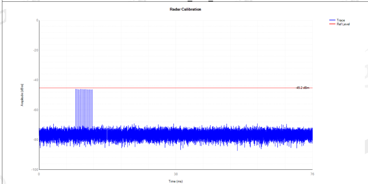
5290MHz DFS_FCC_T5000
