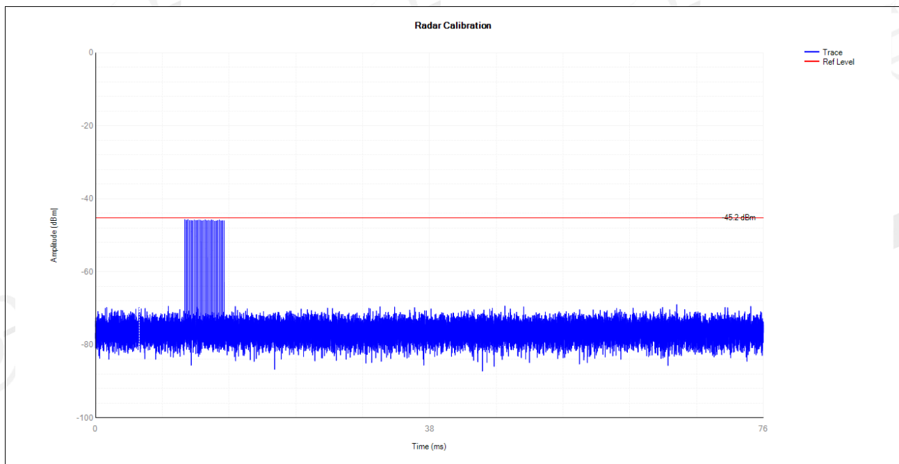
5510MHz DFS_FCC_T3000
