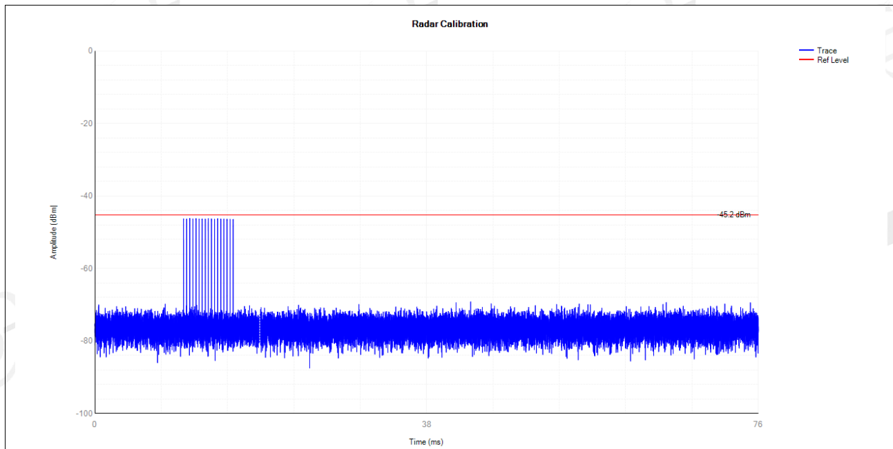
5290MHz DFS_FCC_T4000
