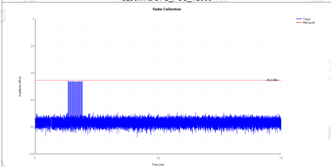
5290MHz DFS_FCC_T3000
