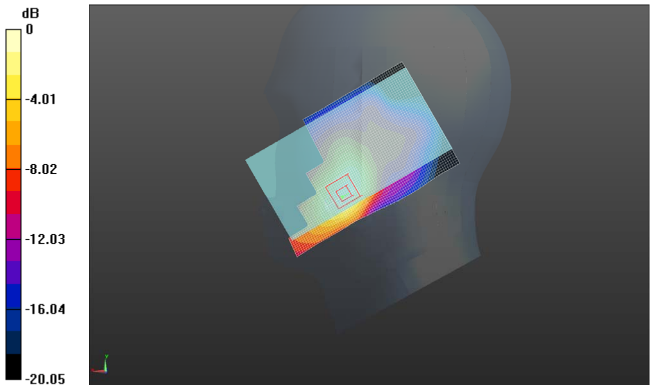
Left Head Cheek (LTE Band VII Middle Channel)
