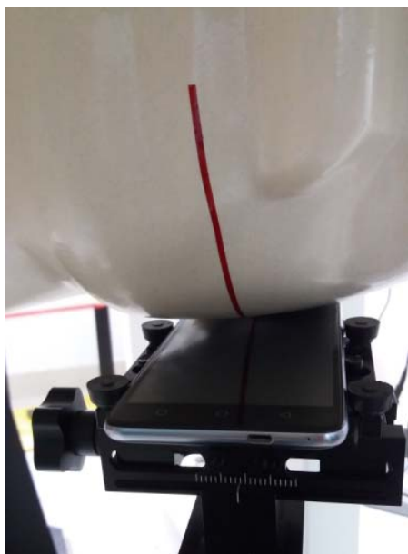
Left Head Tilt (15°)
