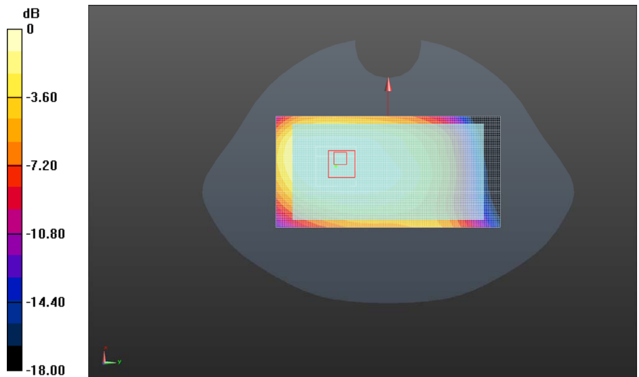
Body- worn Rear Side (LTE Band 17 Middle Channel)
