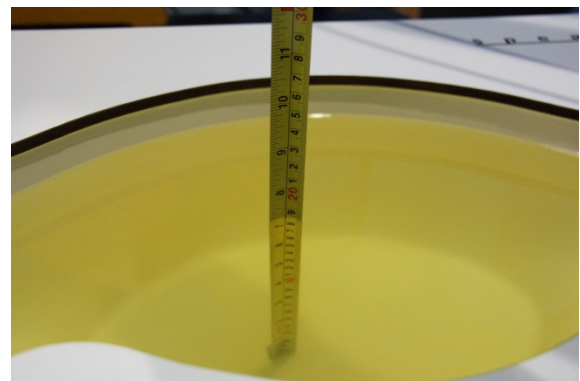
Liquid depth in the body phantom (835MHz)
