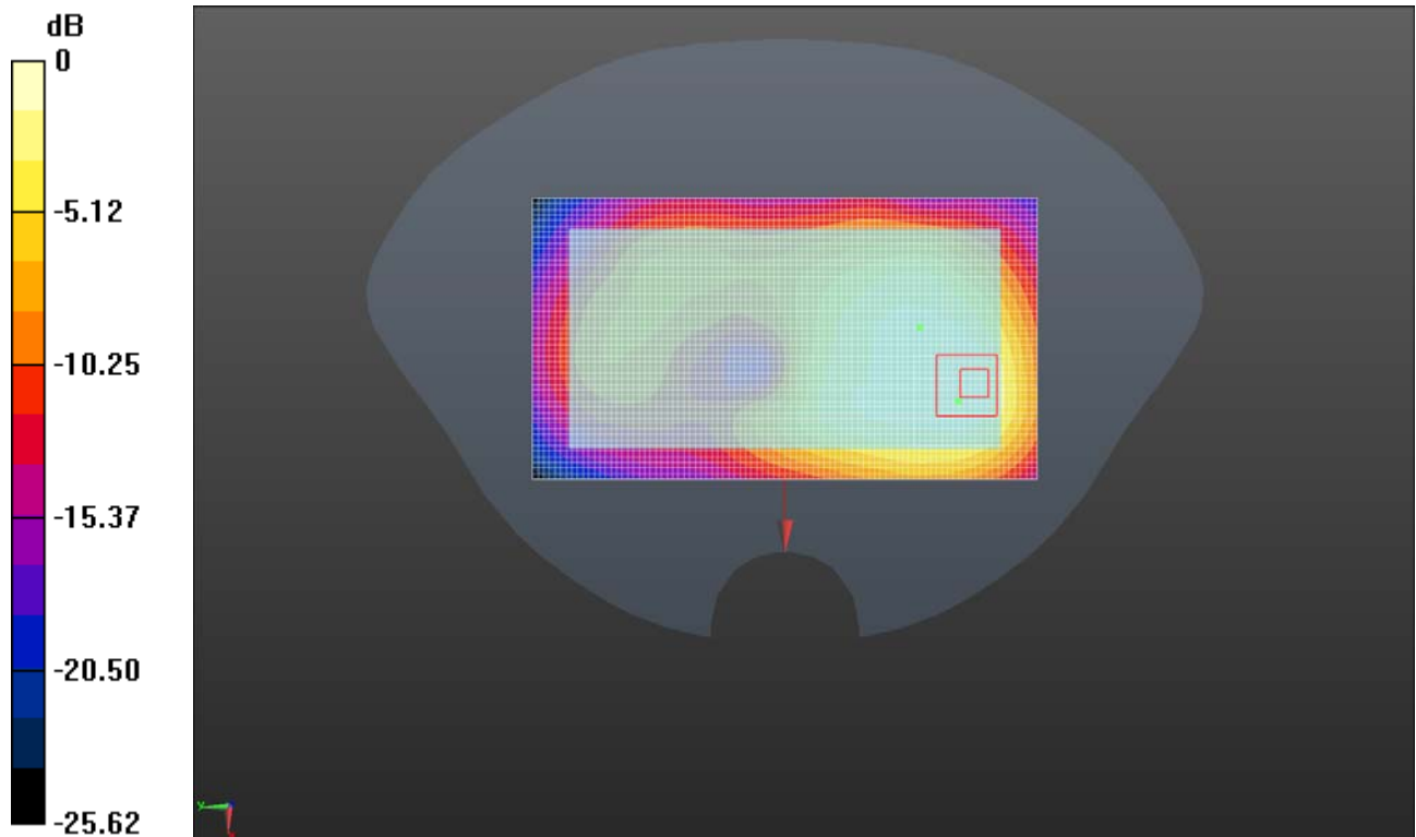
Body- worn Rear Side (LTE Band IV Middle Channel)
