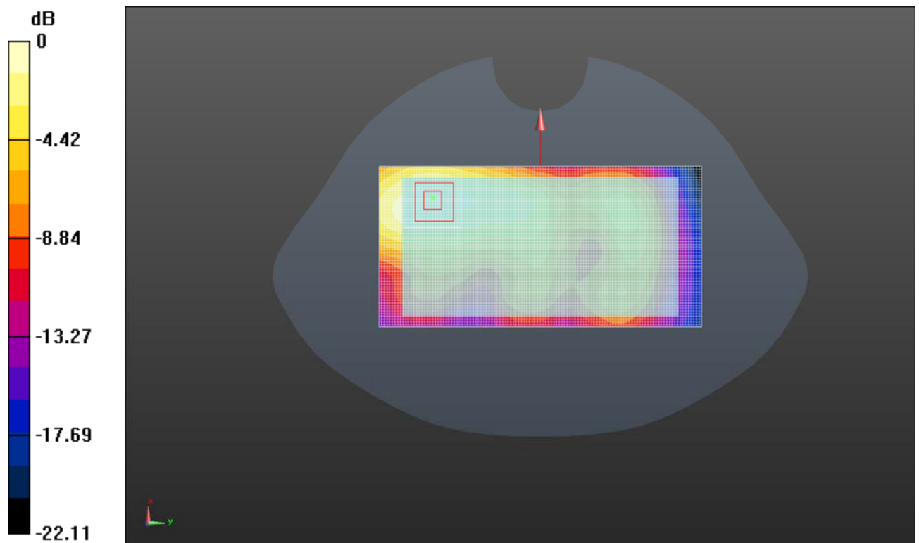
Body- worn Rear Side (LTE Band VII Middle Channel)
