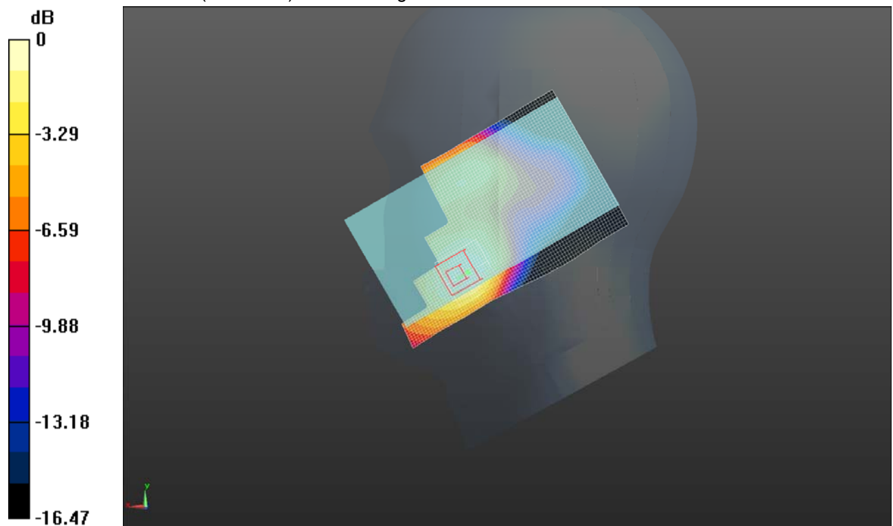
Left Head Cheek (LTE Band IV Middle Channel)
