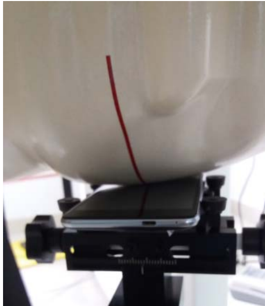
Left Head Touch
