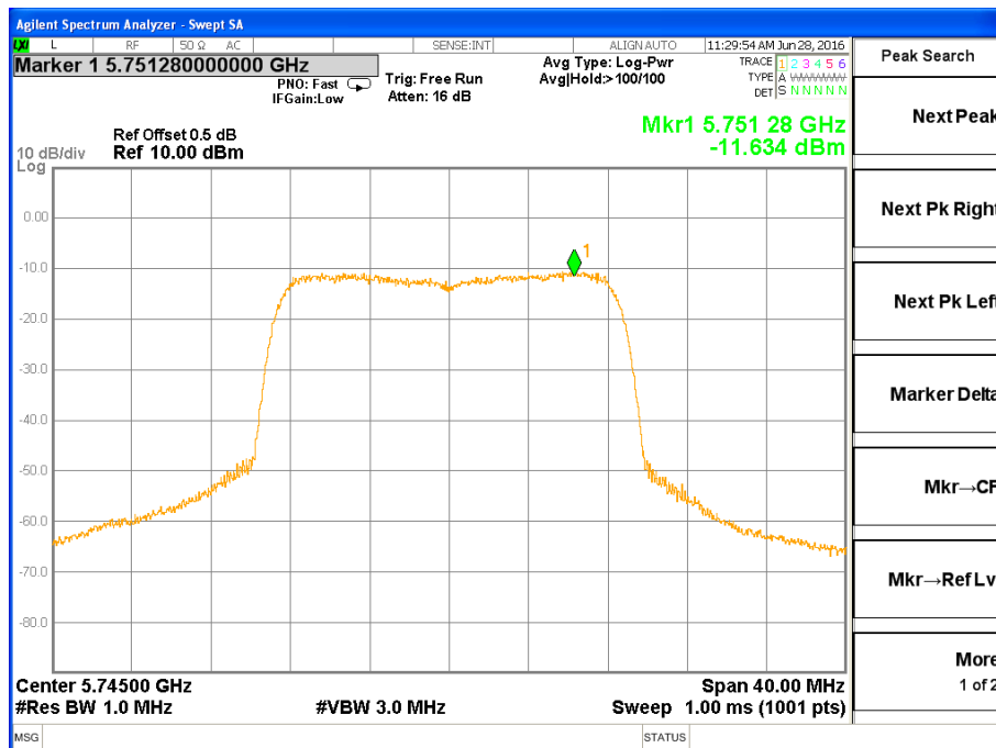
PSD 802.11a Channel 149
