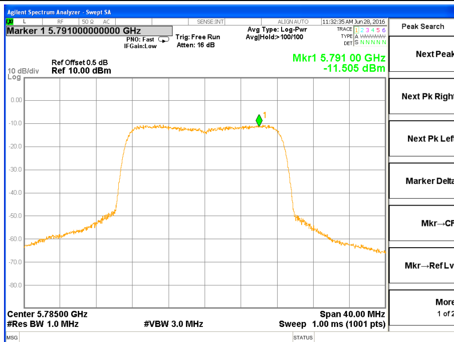
PSD 802.11a Channel 157
