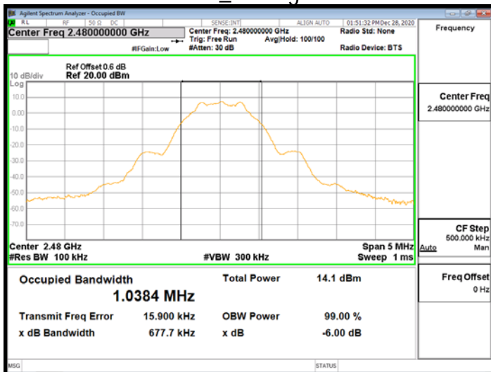
OBW 6dB\BLE_1M\HighCH39-2480
