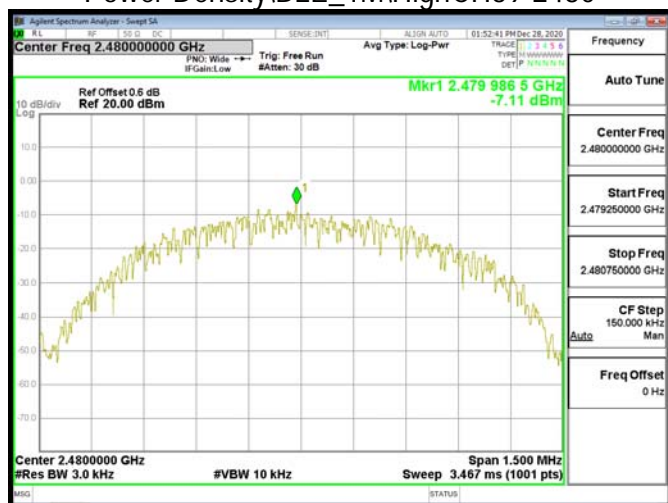
Power Density\BLE_1M\HighCH39-2480
