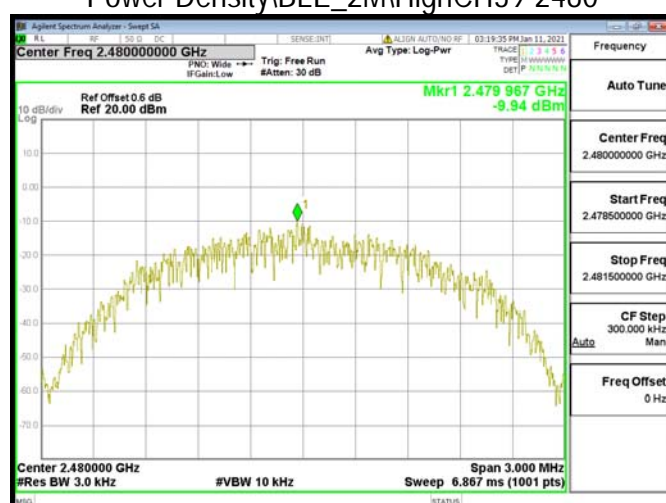
Power Density\BLE_2M\HighCH39-2480
