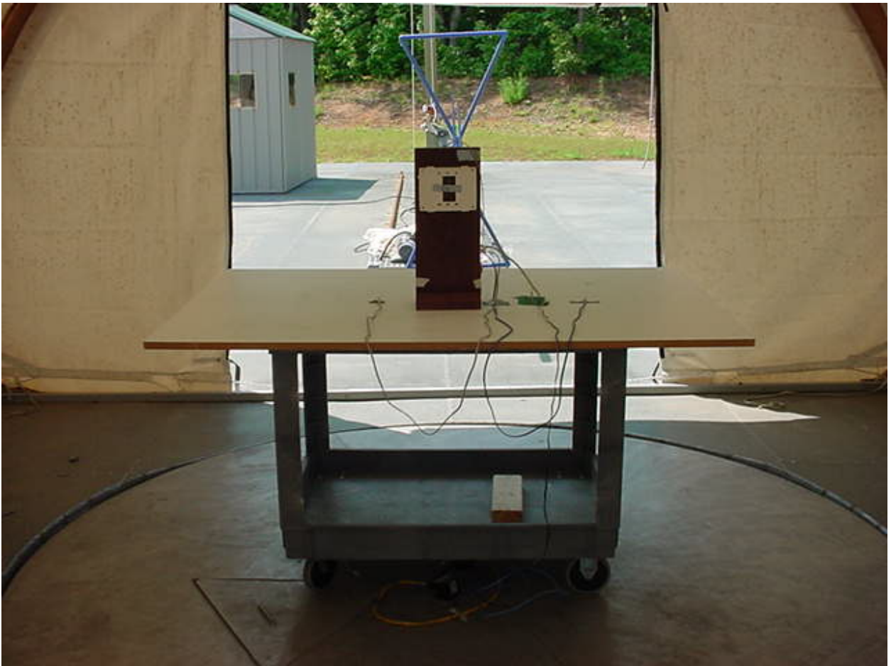
Figure 1: Radiated Emissions – RFRCU Rear View
