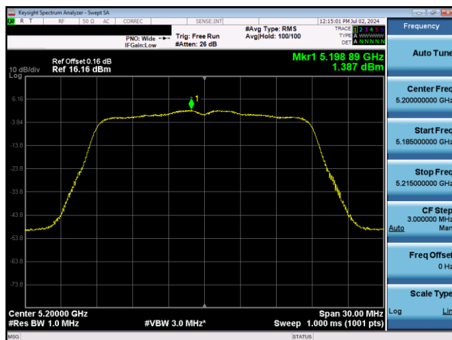
Plot 7-554. ISSED PSD SDM Antenna WF2 (20MHz BW 11n – Ch.40, MCS10)
