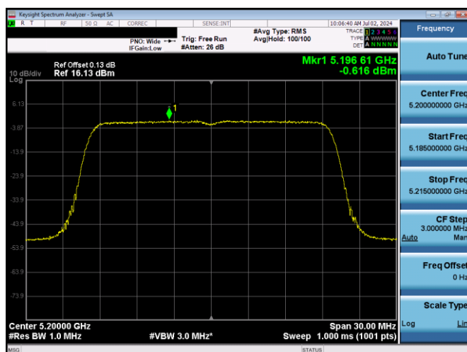
Plot 7-555. ISSED PSD SDM Antenna WF5T (20MHz BW 11ax(SU) – Ch.40, MCS2)
