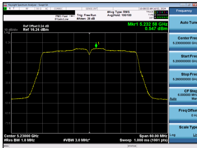
Plot 7-557. ISSED PSD SDM Antenna WF5T (40MHz BW 11n – Ch.46, MCS10)
