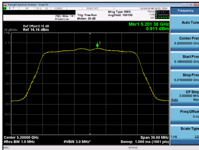
Plot 7-553. ISSED PSD SDM Antenna WF5T (20MHz BW 11n – Ch.40, MCS10)
