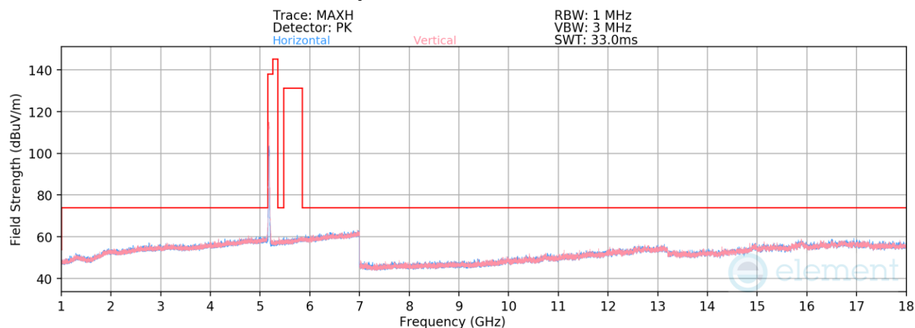
Plot 7-589. Radiated Spurious Emissions above 1GHz Antenna WF5T (802.11n – Ch. 36)
