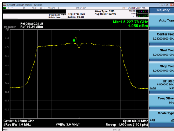
Plot 7-558. ISSED PSD SDM Antenna WF2 (40MHz BW 11n – Ch.46, MCS10)
