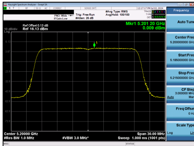
Plot 7-556. ISSED PSD SDM Antenna WF2 (20MHz BW 11ax(SU) – Ch.40, MCS2)
