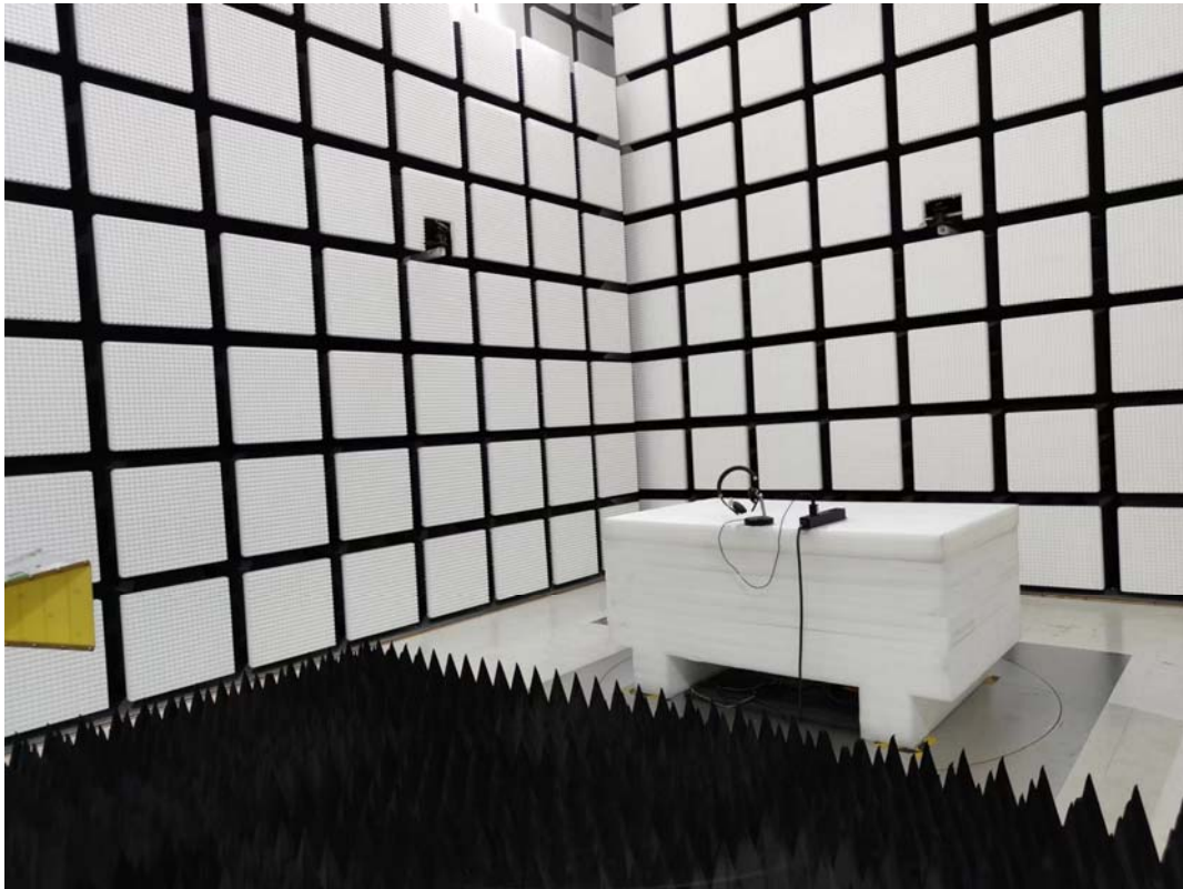
Radiated Emission Above 1GHz rear View -M2
