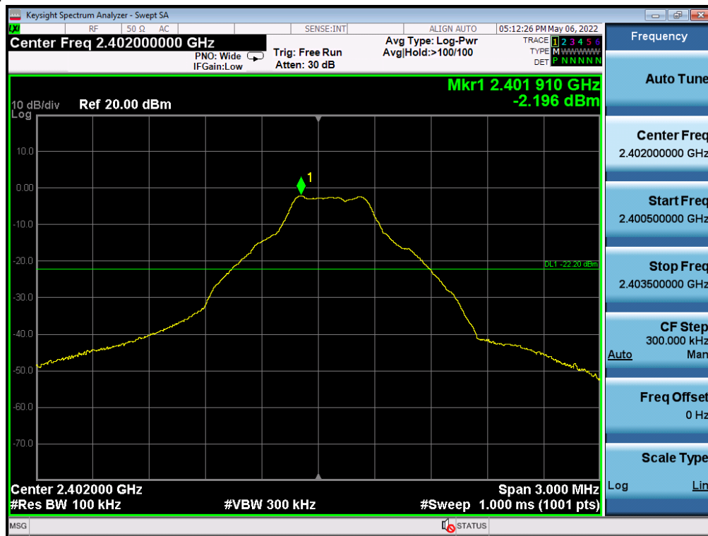
CH:2402MHz
