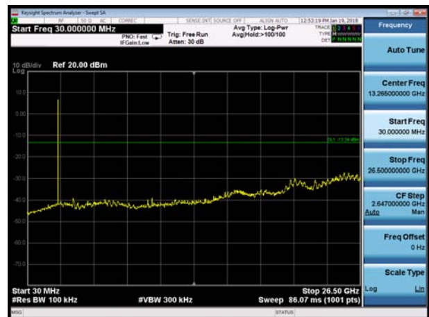
BT 2DH5 CH78 30MHz to 26.5GHz
