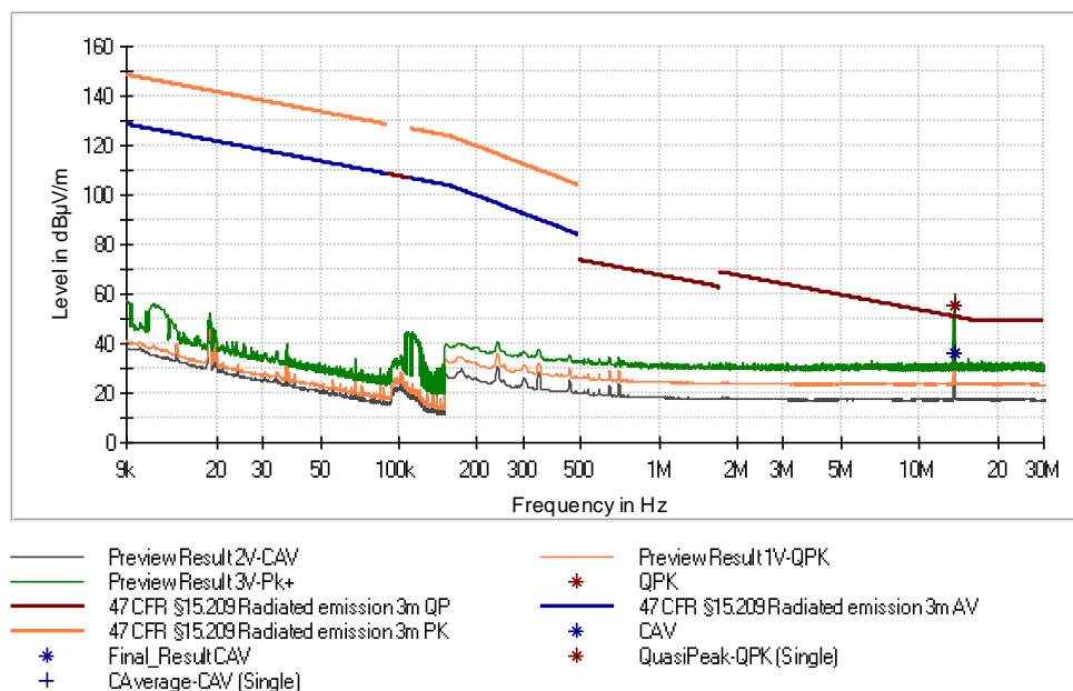
Figure 13: Chart of radiated emissions test below 30 MHz, EUT position Y, antenna polarization parallel, without tag
