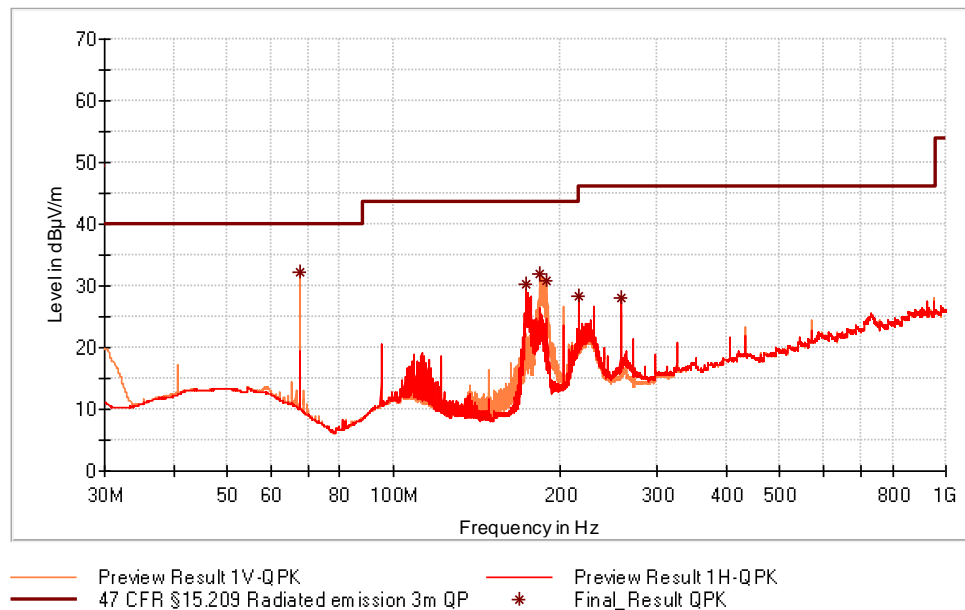
Figure 16: Chart of radiated emissions test from 30 MHz to 1 GHz, EUT position X, antenna polarization horizontal and vertical, with tag
