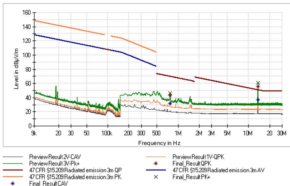
Figure 11: Chart of radiated emissions test below 30 MHz, EUT position Y, antenna polarization parallel, without tag
