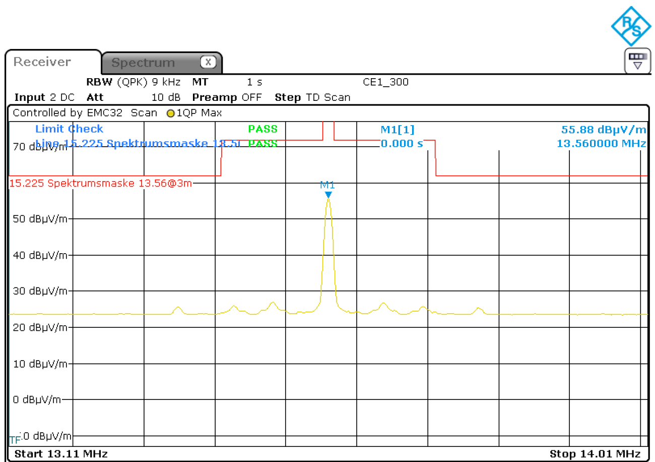
Figure 10: Chart of emission within the band 13.110 MHz to 14.010 MHz, EUT in position Y, without tag, antenna parallel at 3 m distance
