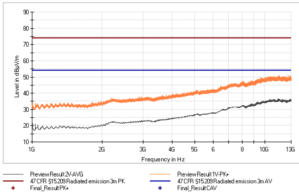
Figure 19: Chart of emissions test from 1 GHz to 13 GHz, EUT position Y, antenna polarization vertical, with tag
