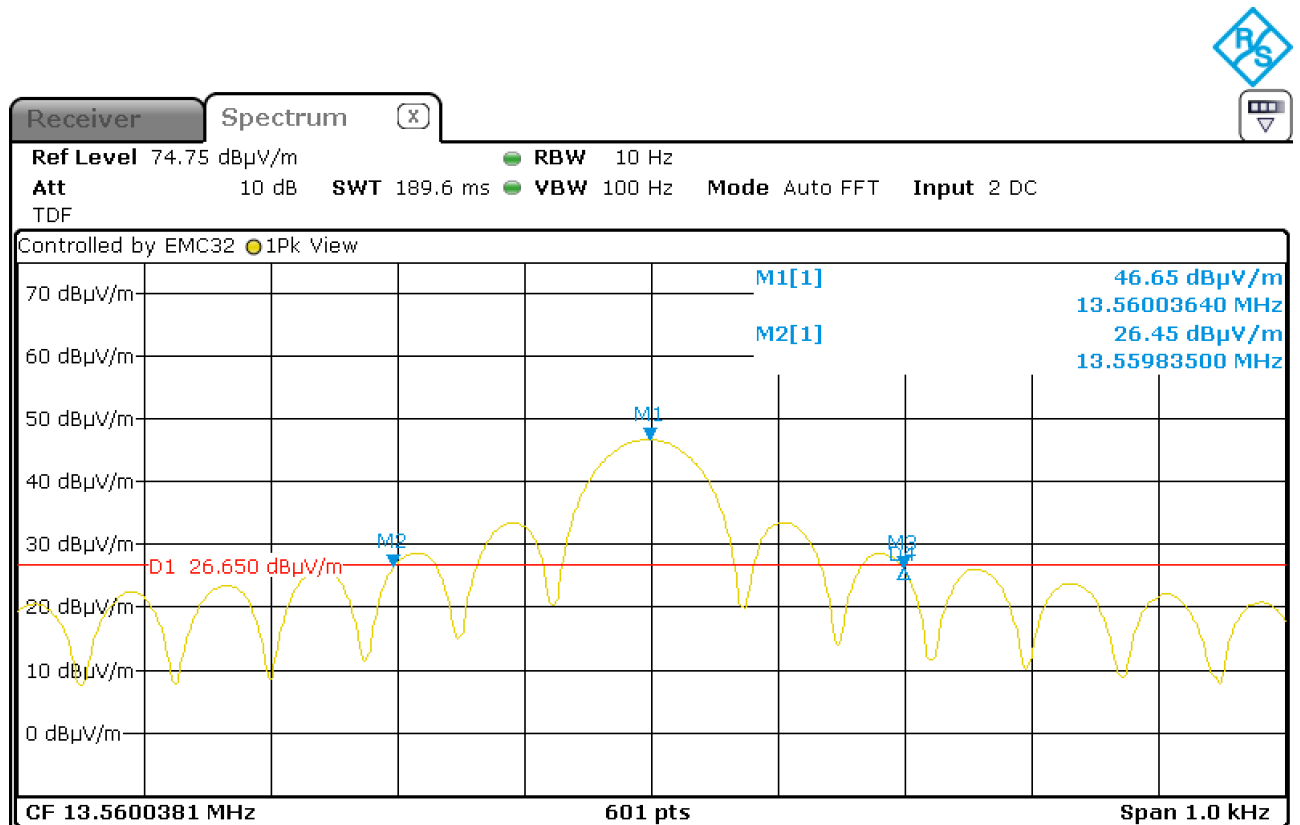
Figure 8: Chart of 20 dB bandwidth tests at normal conditions, without tag
