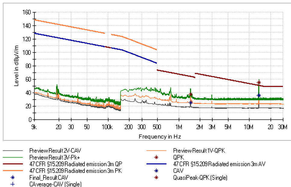
Figure 12: Chart of radiated emissions test below 30 MHz, EUT position Y, antenna polarization parallel, without tag
