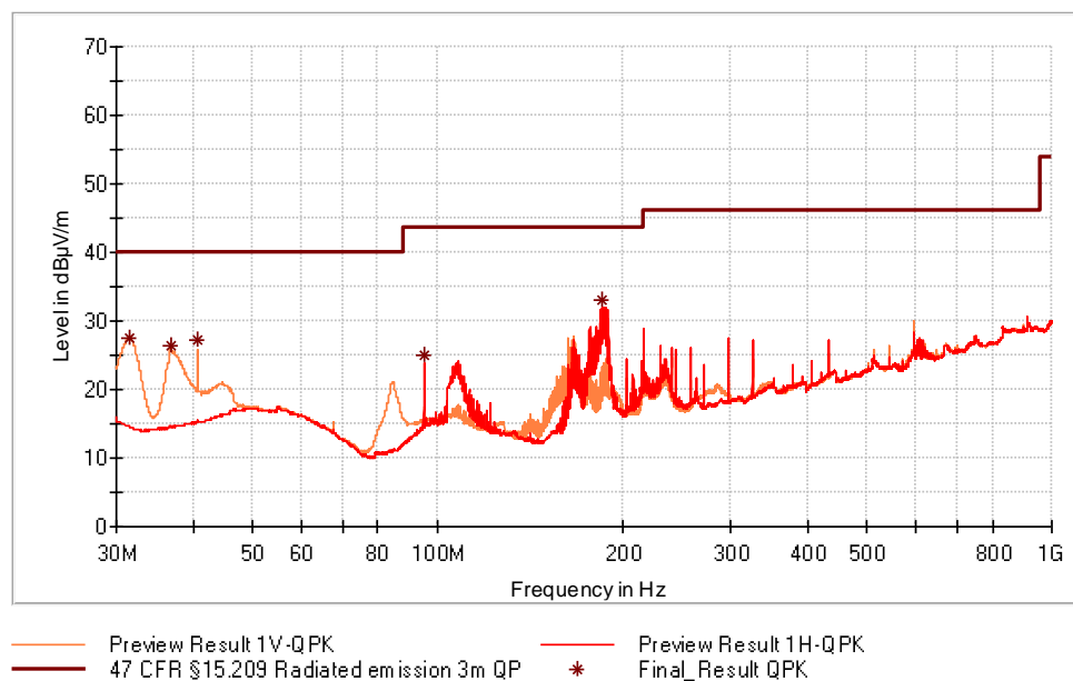
Figure 15: Chart of radiated emissions test from 30 MHz to 1 GHz, EUT position Y, antenna polarization horizontal and vertical, with tag
