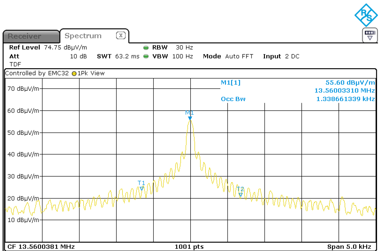
Figure 9: Chart of occupied bandwidth test, without tag
