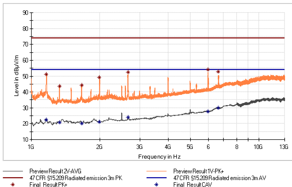
Figure 17: Chart of emissions test from 1 GHz to 13 GHz, EUT position Y, antenna polarization vertical, with tag
