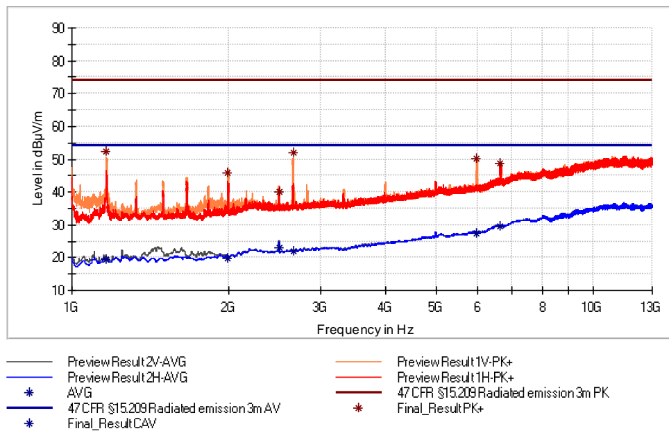
Figure 18: Chart of emissions test from 1 GHz to 13 GHz, EUT position Y, antenna polarization horizontal and vertical, with tag
