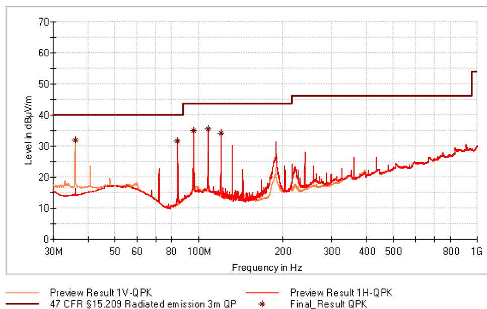
Figure 14: Chart of radiated emissions test from 30 MHz to 1 GHz, EUT position Y, antenna polarization horizontal and vertical, with tag
