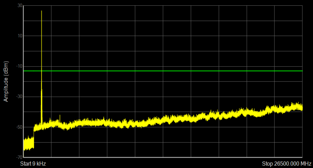
Band66 16QAM BW=10MHz Channel=132322 RB Size=1 Position=#0
