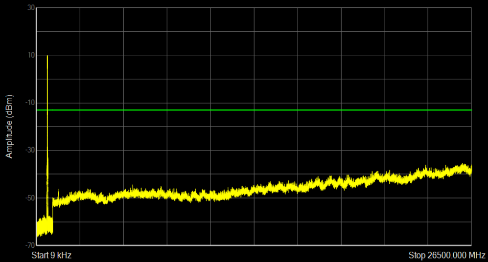
Band71 QPSK BW=20MHz Channel=133372 RB Size=100 Position=#0
