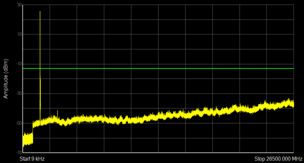
Band66 QPSK BW=20MHz Channel=132072 RB Size=1 Position=#0
