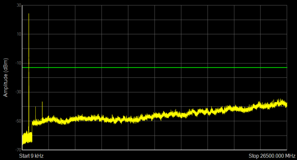
Band71 QPSK BW=10MHz Channel=133297 RB Size=1 Position=#0
