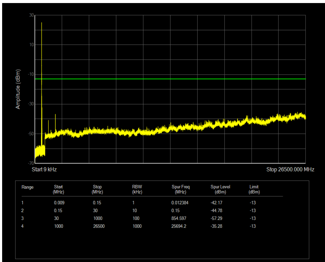
Band71 16QAM BW=20MHz Channel=133322 RB Size=100 Position=#0
