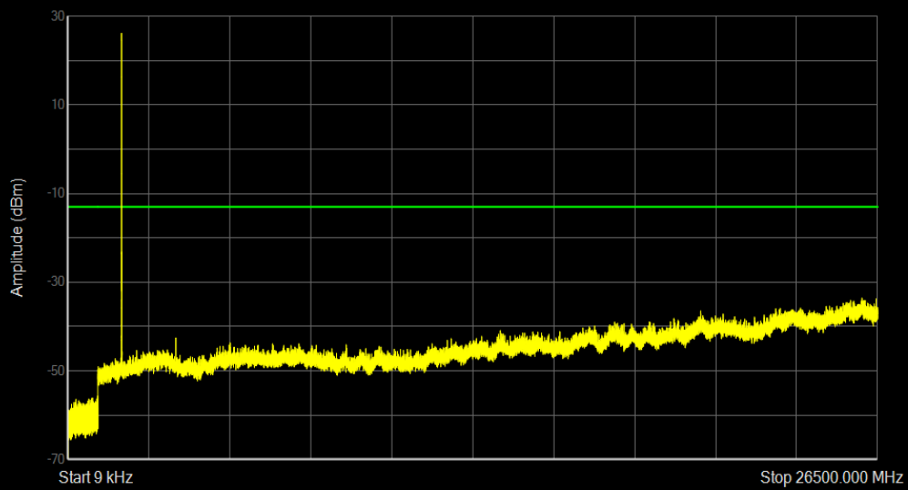
Band66 16QAM BW=5MHz Channel=132647 RB Size=1 Position=#0
