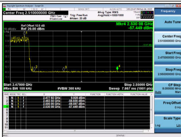
3DH5-Ant1-Hop_2480-PASS
