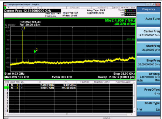
DH5-Ant1-2480-30~25000-PASS
