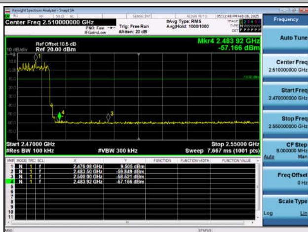
3DH5-Ant1-2480-PASS
