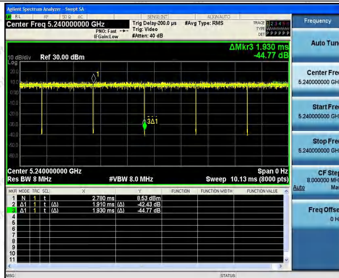
11N20SISO_Ant2_5240
