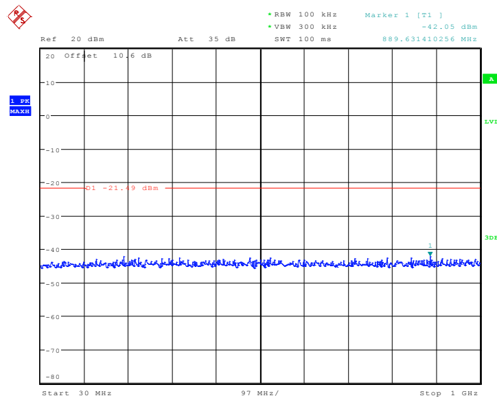
Fig.A.6.1.73 Conducted Spurious Emission (802.11n-HT40, Ch3, Center Frequency)
