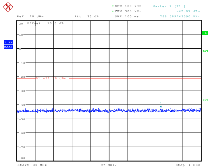
Fig.A.6.1.89 Conducted Spurious Emission (802.11n-HT40, Ch9, Center Frequency)
