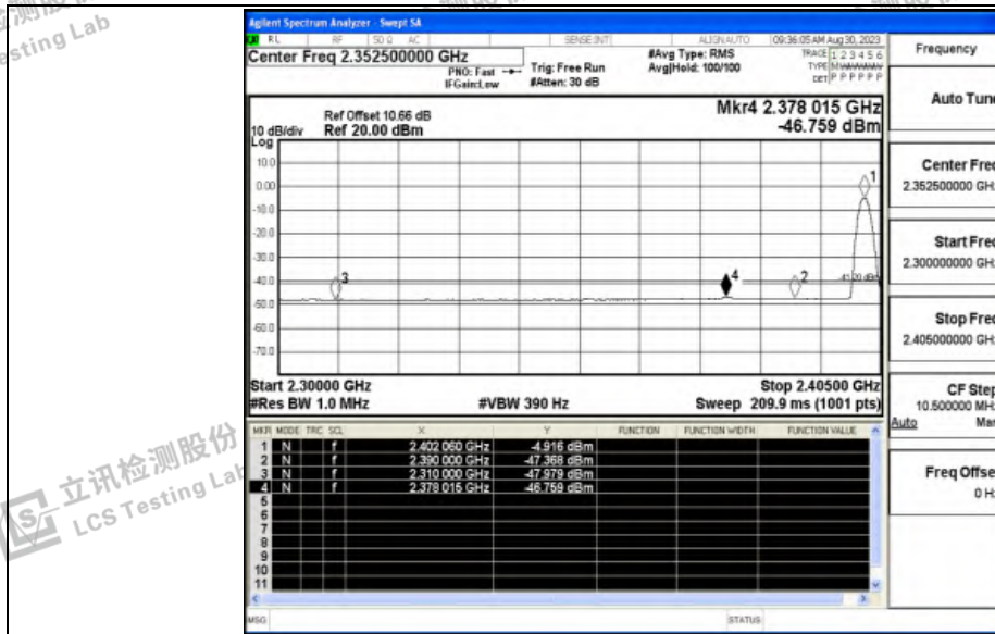
3DH5_Ant_Low_2402_Peak
