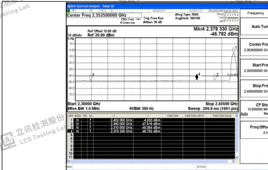
2DH5_Ant_Low_2402_Peak
