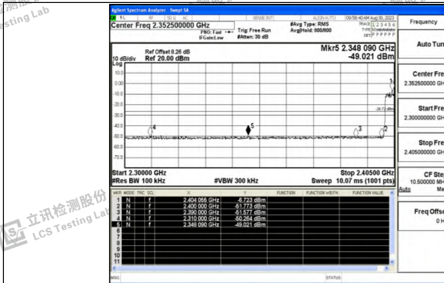
2DH5_Ant_High_Hop_2480
