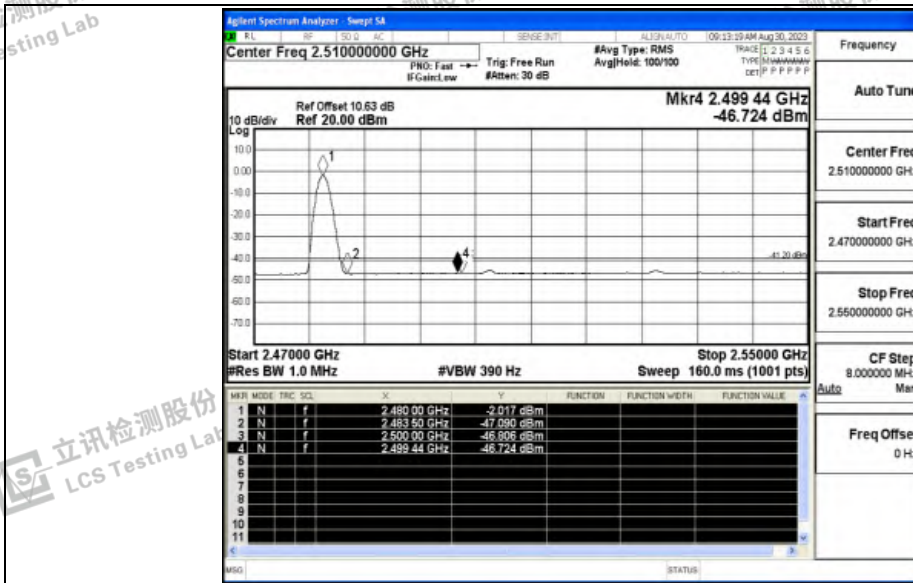
DH5_Ant_High_2480_Peak
