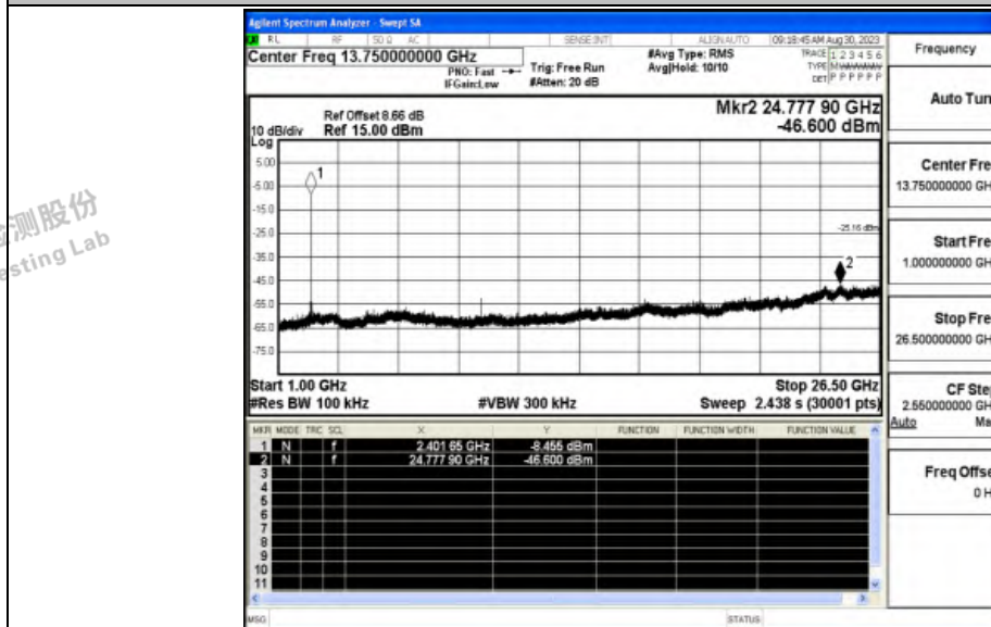
2DH5_Ant_2441_0-Reference
