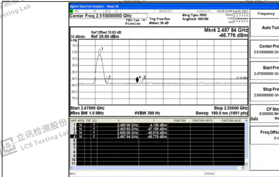
2DH5_Ant_High_2480_Peak
