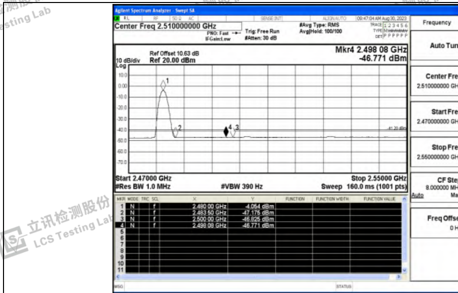
3DH5_Ant_High_2480_Peak
