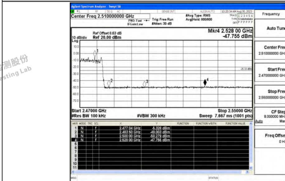
3DH5_Ant_High_Hop_2480
