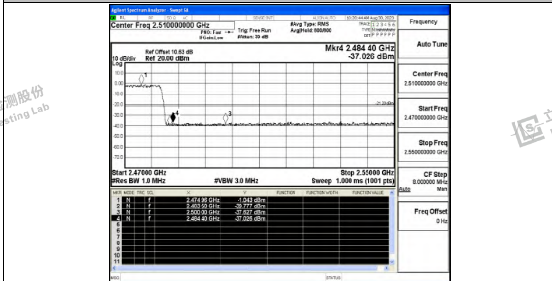
3DH5_Ant_High_Hop_2480_Peak
